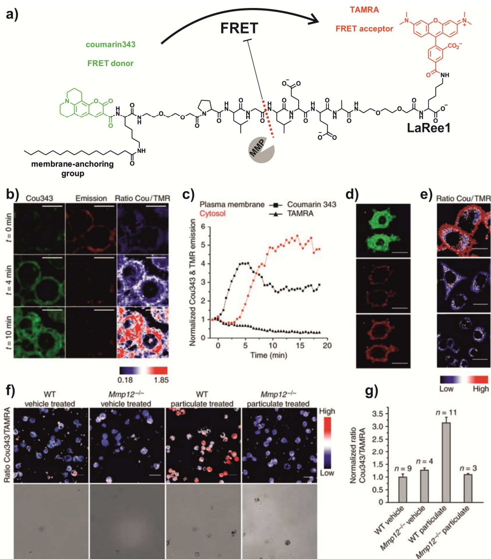
Fig. 3. FRET probes for imaging MMP-12 activity on macrophages. a) Chemical structure of the FRET probe LaRee1 incorporating coumarin343 as the donor and TAMRA as the acceptor. b) Time-course fluorescence microscopy images of macrophages after treatment with LaRee1 and recombinant MMP-12: t=0 , coumarin343 fluorescence emission was quenched and TAMRA showed sensitized emission, t=4 and 10 min: strong ratiometric change was observed and the green fluorescence shifted from the plasma membrane to the cell interior (scale bar: 10 \mu\text{m} ). c) Plots of coumarin343 and TAMRA fluorescence emission traces at the plasma membrane and in the cytosol over time. d) After LaRee1 was added to LPS-stimulated macrophages, the emission ratio was accompanied by an increase of green fluorescence inside cells (top panel) and a loss of FRET signal emission (centre panel). Direct TAMRA excitation showed the predominant plasma membrane location of the remaining intact reporter and demonstrated extracellular cleavage (bottom panel) (scale bar: 20 \mu\text{m} ). e) MMP activity was found on LPS-stimulated macrophages (top panel) but not in unstimulated ones (centre panel) or those stimulated but also treated with the MMP inhibitor GM6001 (bottom panel). f) LaRee1 images MMP12 activity from wild-type (WT) and Mmp12^{-/-} mice that were challenged with particulate fraction or vehicle by intratracheal instillation. g) Quantification of MMP-12 activity showed a significant increase in WT particulate-challenged mice compared to control or Mmp12^{-/-} mice. Reproduced with permission from the Nature Publishing Group. 34
