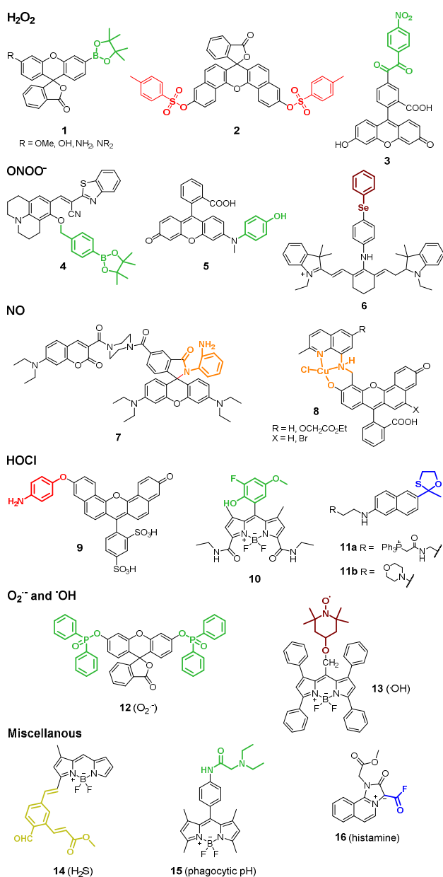
Fig. 2. Smart fluorescent probes for imaging intracellular activity in macrophages. Representative structures of reactive fluorophores for the detection of ROS/RNS as well as other metabolites associated to macrophage activity. The different probes are classified according to their targets: H 2 O 2 , ONOO - , NO, HOCl, O 2 - , • OH, H 2 S, phagocytic pH and histamine. The different chemical reactive groups in the smart probes are highlighted in bold and in the colour of the resulting fluorescence emission after activation.
