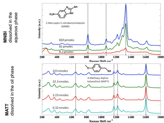
Fig.10. SERS dilution series for analytes dissolvable in different phases. Amount of analyte is given per 1mL of water or oil, correspondingly. This figure has been edited from reference 16 with permission from Nature Publishing Group.
