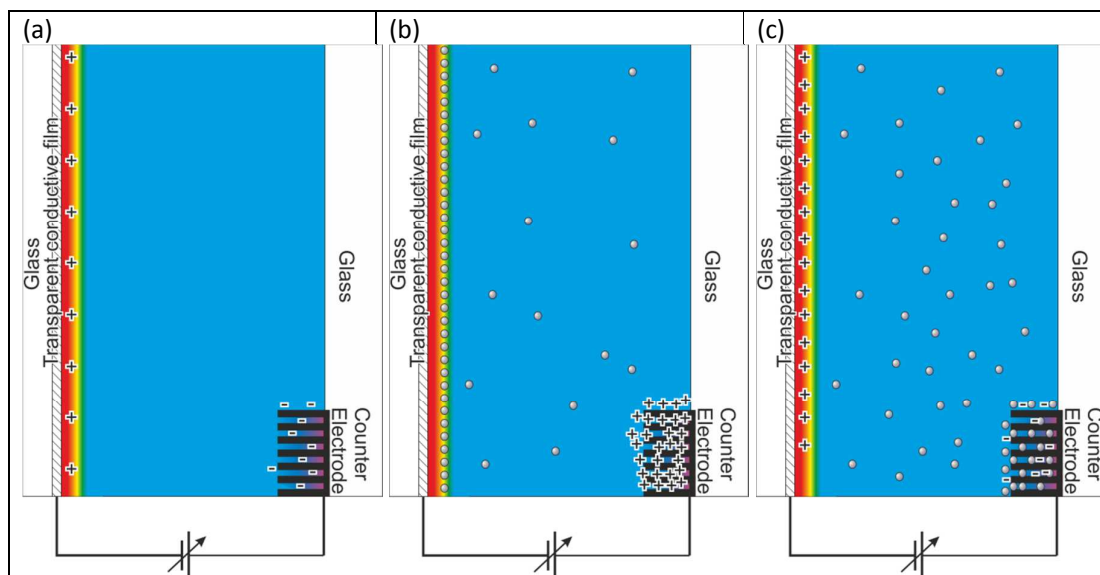
Fig.4. Cartoon of a polarized transparent electrochemical cell involving a solid/liquid interface. (a) The double layers rich in cations forming on negatively polarized transparent conducting film electrode and rich in anions on the positively charged high surface area counter electrode in a metal particle free solution. (b) In the metal NP containing solution, the negatively charged particles are drawn to the TCO film from the solution due to the electric double layer and at the same time positively charged ions build up on the counter electrode; (c) polarising the electrode so that the negatively charged nanoparticles are no longer stable at the interface leads to their dispersal throughout the solution and at the counter electrode. For simplicity, the negative charges on the NP are not shown, and neither are the free charges in solution.
