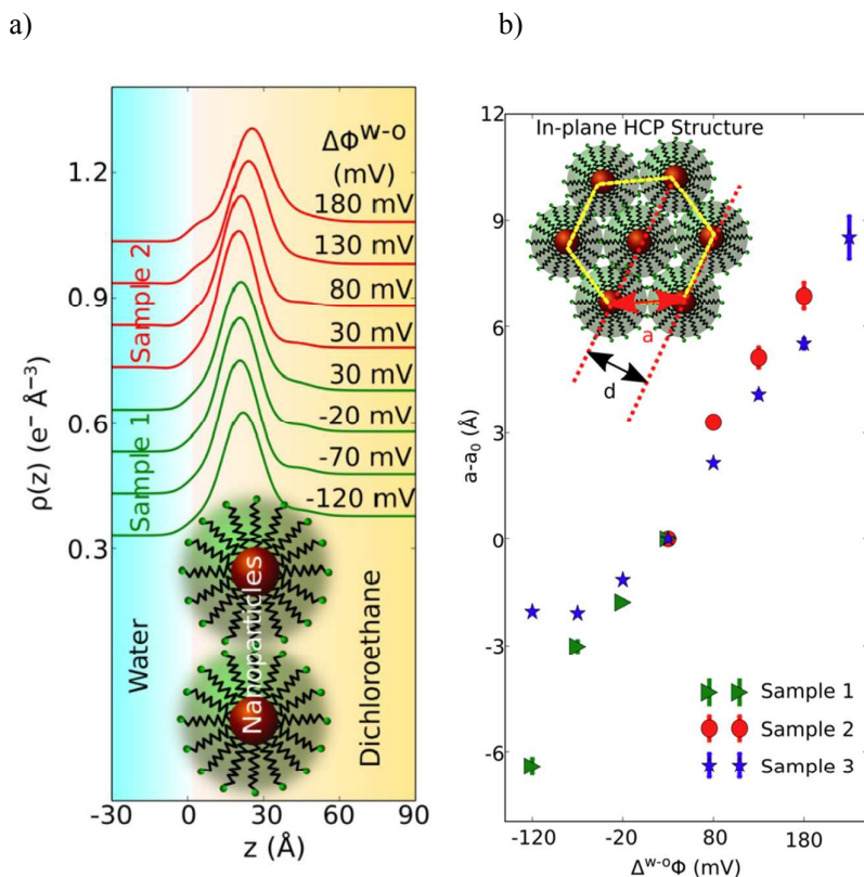
Fig.9. a) Electron density profiles of TTMA-functionalized Au NPs at the water | DCE ITIES. Variation of electron density \rho(z) along the direction z (perpendicular to the interface) obtained from fitting X-ray reflectivity data. A cartoon of NPs at the interface is also shown. The peak in the electron density profiles indicates the location of the NP gold core. The profiles demonstrate that TTMA-functionalized Au NPs are located primarily on the DCE side of the interface with small changes in their depth as the electric potential difference \Delta\phi^{w-o} across the interface is varied from -120 mV to +180 mV. b) Electrovariable lattice spacing of a 2-dimensional NP array formed at the water | DCE ITIES. 25 The variation in the nearest-neighbour spacing a , measured by grazing-incidence X-ray diffraction, is shown for three different samples as a function of the electric potential difference across the interface, \Delta\phi^{w-o} . The spacing a is referenced to the spacing a_0 measured at \Delta\phi^{w-o} = 30 mV for each sample ( a_0 = 67.2, 61.5 and 64.5 Å for samples 1, 2 and 3 respectively). Inset: Cartoon of the 2D hexagonal close-packed structure of NPs illustrating the nearest-neighbour spacing a and lattice spacing d . This figure has been reproduced from reference 25 with permission from the American Chemical Society.
