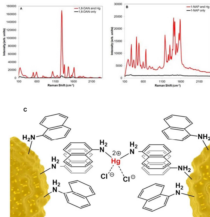
Fig.11. Enhancement of the Raman signal of A) 1,8 DAN and B) 1-NAP ligands in the presence 10^{-4} molar concentration of \text{Hg}^{2+} ions. (C) A putative model for binding of 1-naphthylamine (1-NAP) to the NP surface and the complexing mechanism for \text{Hg}^{2+} binding to outstanding free nitrogen terminals. This figure has been reproduced from reference 34 with permission from Wiley.
