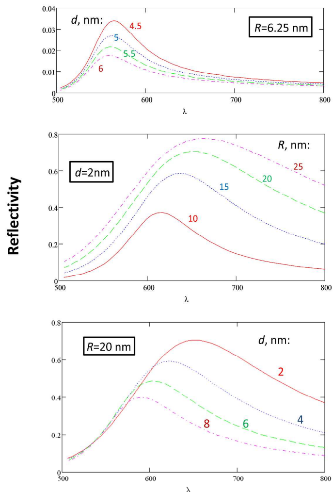
Fig.12. Reflection from a hexagonally structured monolayer of gold NPs at water/DCE interface (light propagating from the DCE side at normal incidence), calculated following the Effective Medium Dipole Approximation Theory 36,37 and Drude-Lorentz approximation for dielectric function of gold. The upper panel displays weak reflection from the layer of medium size NPs (of radius 6.25 nm) for indicated values of surface to surface separation, d . Middle panel shows the effect of the size of NPs at dense packing ( d = 2 ). The lowest panel shows the effect of surface-to-surface separation for medium size NP, R = 20 nm. Decrease of surface-to-surface separation moves maximum of reflection to the red; the effect is stronger for larger NPs. This figure has been reproduced from reference 37 with permission from the American Chemical Society.
