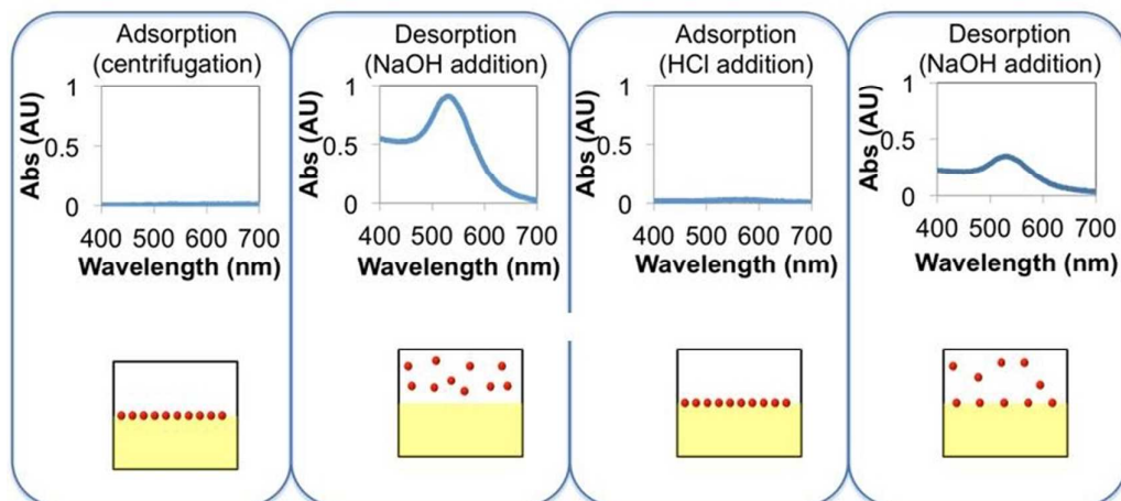
Fig.7. Adsorption desorption of gold NPs from aqueous electrolyte/1,2-dichloroethane interface induced by varying the charge on NPs via varying the acidity of aqueous solution. This figure has been reproduced from reference 19 with permission from the American Chemical Society.
