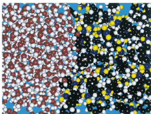
Fig.3. Molecular dynamic simulations of an interface between water and nitrobenzene (a) Room temperature density profiles water and nitrobenzene. Liquid-liquid interface is around Z=0 . (b) A snapshot of the complete water (on the left)/nitrobenzene (on the right) simulation system. This figure has been reproduced from reference 3 with permission from Elsevier.
