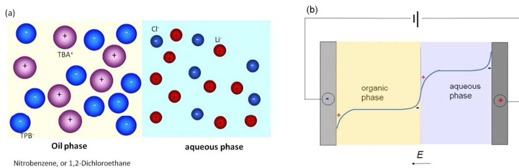
Fig.2. (a) A cartoon of a typical ITIES at the molecular scale. The positive free energy of solvation of the ionic species in the neighbouring phase mean that they do not spontaneously into that phase. \text{TBA}^+ = Tetrabutyl ammonium cation; \text{TPB}^- = Tetraphenyl borate anion. (b) Polarised ITIES. Sign denote the excess of cations (+) and anions(-) in the electrical double layers.
