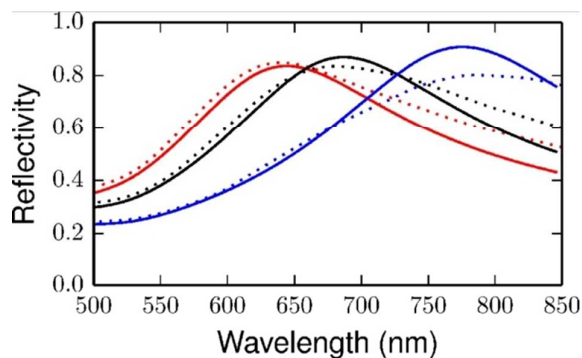
Fig.13. Calculated reflectivity of an array of core-shell [SiO 2 @Au] NPs assembled in water at a semi-infinite ITO electrode covered by SAM spacer. Compared are the spectra calculated with the Effective Medium Dipole Approximation theory (solid lines) and finite difference time domain numerical simulations (dotted lines). Optical dielectric constant 1.78; for simplicity the same value is assumed for the spacer. In the results shown, the centres of NPs are aligned in a hexagonal array (at surface coverage \Gamma = 0.722 ) in the plane disposed a distance h = 18 nm from the surface of the ITO electrode. The outer radius of NPs, R_s = 16 nm, the optical dielectric constant of silica is taken as 2.25, and the frequency dependent dielectric permittivities of gold and ITO are fitted to the literature experimental data (c.f. 37 ). Light incidence is from water, normal to the interface. The plot shows the effect of varying shell thickness: R_c = 4 nm (blue), 6 nm (black), and 8 nm (red). This figure has been reproduced from reference 36 with permission from the American Chemical Society.
