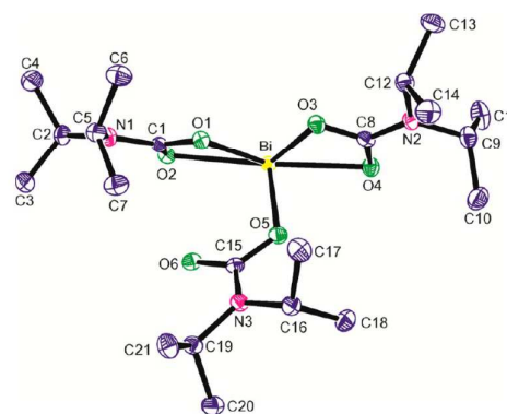
Fig. 31. Asymmetric unit of [Bi(O 2 CN i Pr 2 ) 3 ] thermal ellipsoids are at 40% probability, the co-crystallised disordered solvent, and hydrogen atoms omitted for clarity. Reproduced with permission from ref. 244. Copyright 2013 American Chemical Society.
