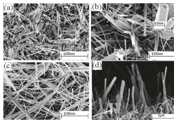
Fig. 13. SEM of \text{Bi}_2\text{S}_3 deposited via AACVD from [\text{Bi}(\text{S}_2\text{CNET}_2)_3]_2 in chloroform at (a) 350 °C, (b) 400 °C, (c) 450 °C and (d) cross-section of film deposited at 400 °C. The inset of (b) shows a high resolution image of a nanotube. Reproduced with permission from ref. 114. Copyright 2014 American Chemical Society.
