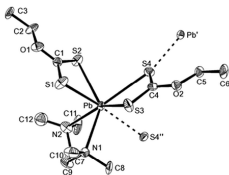
Fig. 12. The asymmetric unit of [\text{Pb}(\text{S}_2\text{COEt})_2 \cdot \text{tmeda}] showing the labelling scheme used; thermal ellipsoids are at the 40% level. Reproduced from ref. 104 with permission from The Royal Society of Chemistry.
