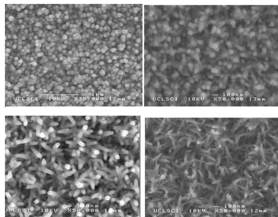
Fig. 25. Combinatorial AACVD: SEM images taken across the deposited film, showing the change from Ga 2 O 3 (top left), through mixed gallium-indium-oxide (top right, bottom left) to In 2 O 3 (bottom right). Reproduced from ref. 191 with permission from The Royal Society of Chemistry.
