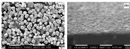
Fig. 33. SEM images of \text{Bi}_2\text{Se}_3 deposited from [\text{Bi}(\text{N}[\text{SeP}]\text{Pr}_2)_2]_3 by AACVD at 475 °C on glass. Reproduced with permission from ref. 116. Copyright 2004 Copyright 2013 American Chemical Society.
