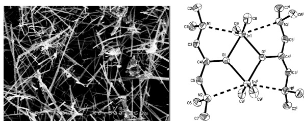
Fig. 23. Left, SEM image of \text{In}_2\text{O}_3 deposited from the reaction of \text{InMe}_3 and \text{HOCH}_2\text{CH}_2\text{OMe} at 550 °C, and right, X-ray structure of [\text{Me}_2\text{In}(\text{OCH}(\text{CH}_2)\text{NMe}_2)_2] with thermal ellipsoids shown at the 50% probability level. Reproduced with permission from ref. 171. Copyright 2012 American Chemical Society.
