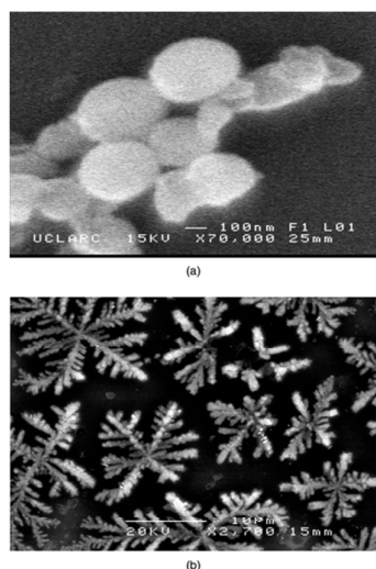
Fig. 19. SEM images of Ga_2O_3 deposited at 550 °C from [Ga(NMe_2)_3]_2 with (a) HOCH(CH_2NMe_2)_2 and (b) HOCH(CH_3)CH_2NMe in toluene. Reproduced from ref. 154 with permission from The Royal Society of Chemistry
