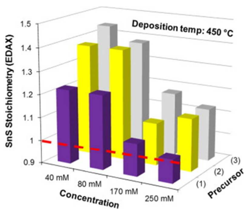
Fig. 9. The effect of concentration of precursors where (1) is [Sn(S 2 CNEt n Bu) 2 ], (2) is [Sn(S 2 CNEt n Bu) 2 ] and (3) is [Sn(S 2 CNEt) 2 ] on the stoichiometry (%Sn divided by %S found experimentally by EDAX) of SnS films deposited at 450 °C by AACVD. The dashed line indicates an ideal 1:1 Sn:S stoichiometry i.e. SnS. Reproduced with permission from ref. 99. Copyright 2014 Elsevier.
