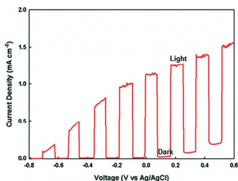
Fig. 36. J-V plot of \text{In}_2\text{S}_3 films obtained from AACVD at 400 °C from [\text{In}(\text{S}_2\text{CN}^i\text{Pr}_2)_3.1.5(\text{py})] . Reproduced with permission from ref. 85. Copyright 2013 RSC.
