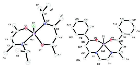
Fig. 21. ORTEP diagrams showing [\text{Ga}((\text{Me})\text{CN}(\text{H})\{\text{Pr}\})\text{-CHC}(\text{Me})=\text{O}]_2\text{Cl} , left and [\text{Ga}((\text{CH}_2)_2\{\text{N}(\text{H})\text{C}(\text{Me})\text{-CHC}(\text{C}_6\text{H}_5)=\text{O}\}_2)\text{Me}] , right. Thermal ellipsoids are drawn at 50% probability. Reproduced from ref. 168 with permission from the Centre National de la Recherche Scientifique (CNRS) and the Royal Society of Chemistry.
