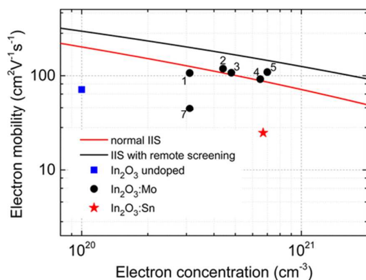
Fig. 26. Electron mobility and concentration for undoped, Sn-doped and Mo-doped In 2 O 3 . The numbers by the data points correspond to the mol % of Mo dopant in the solution used in the AACVD. The model curves for regular ionized impurity scattering (IIS) (red line) and for remotely screened IIS (black line). All calculations are for singly ionized Mo donor atoms. Reproduced with permission from ref. 193. Copyright 2015 American Chemical Society.
