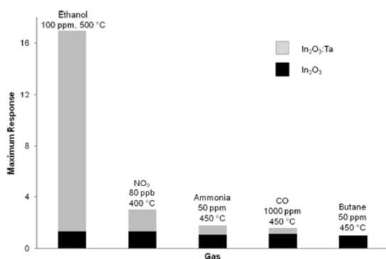
Fig. 37. Maximum gas response of \text{In}_2\text{O}_3 and \text{In}_2\text{O}_3:\text{Ta} sensors to different gases in flowing air at optimum operating temperatures. Reproduced with permission from ref. 256. Copyright 2012 American Chemical Society.
