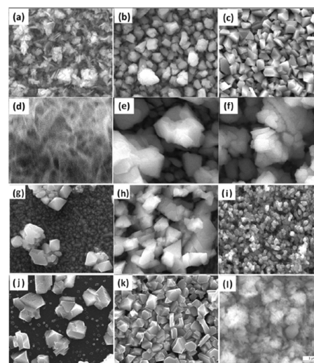
Fig. 8. SEM images of \beta\text{-In}_2\text{S}_3 films deposited using the precursors [\text{In}(\text{S}_2\text{CN}(\text{C}_2)_3) \cdot 2\text{py}] at (a) 300 °C, (b) 350 °C and (c) 400 °C; [\text{In}(\text{S}_2\text{CN}(\text{Pr}_2)_3) \cdot 1.5\text{py}] at (d) 300 °C, (e) 350 °C and (f) 400 °C; [\text{In}(\text{S}_2\text{CN}(\text{Pip})_3) \cdot 0.5\text{py}] at (g) 300 °C (h), 350 °C and (i) 400 °C and [\text{In}(\text{S}_2\text{CNBzMe}_3)] at (j) 300 °C, (k) 350 °C and (l) 400 °C. Reproduced from ref. 85 with permission from The Royal Society of Chemistry.
