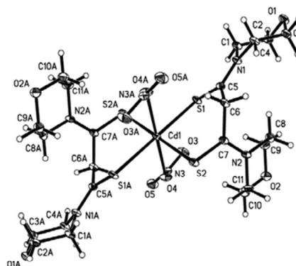
Fig. 2. Molecular structure of [Cd(msacmsac)_2(NO_3)_2] with thermal ellipsoids plotted at the 50% probability. Reproduced from ref. 31 with permission from The Royal Society of Chemistry.
