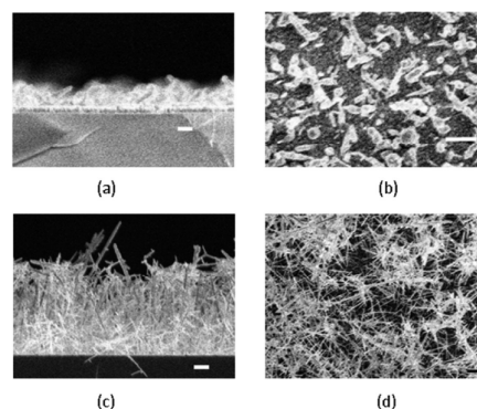
Fig. 32. SEM of the films grown from [Bi(O 2 CN i Pr 2 ) 3 ], (a,b) at 300 °C for 40 minutes, and (c,d) at 450 °C for 40 minutes. Reproduced with permission from ref. 244. Copyright 2013 ACS.
