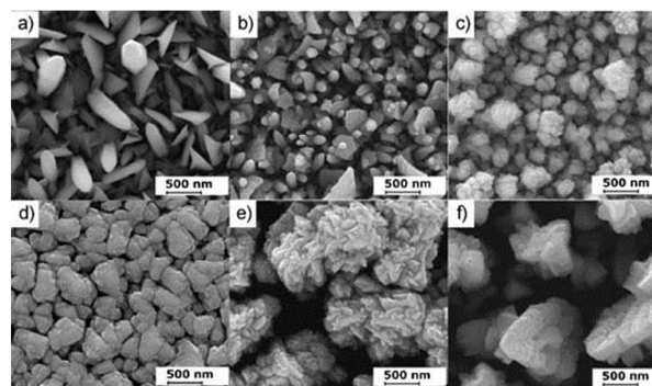
Fig. 3. SEM images of CdS thin films deposited from [Cd(S_2CNCy_2)_2.py] on FTO (a–c) and soda glass (d–f) at 350, 400, and 450 °C from THF solution. Reproduced with permission from ref. 37. Copyright 2012 Wiley.
