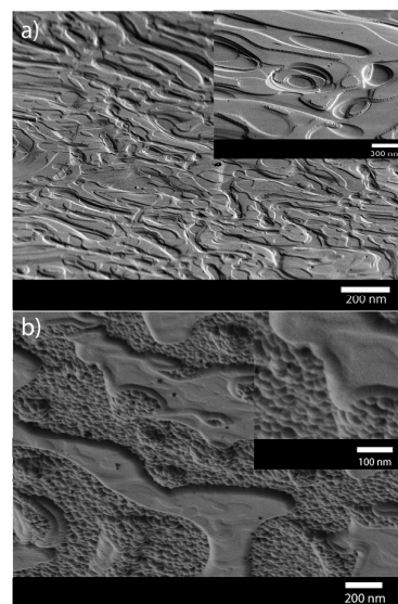
Fig. 5. SEM images of crystalline GaAs films grown via AACVD from As(NMe_2)_3 and GaMe_3 at (a) 500 °C and (b) 550 °C. Reproduced from ref. 63 with permission from The Royal Society of Chemistry.
