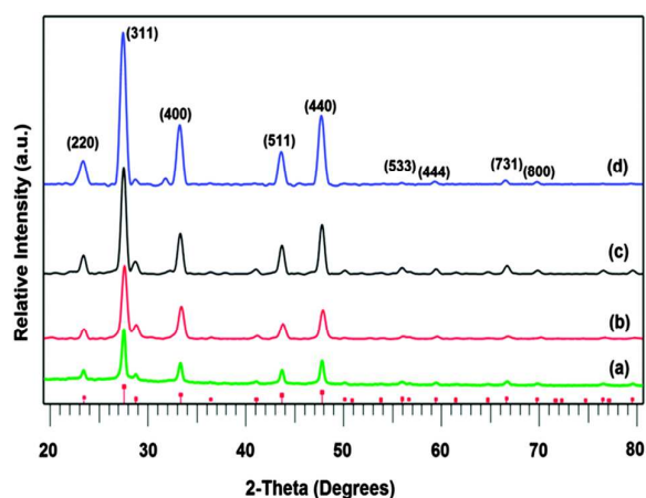
Fig. 6. p-XRD patterns of as deposited In 2 S 3 thin films from In[(S 2 P i Bu 2 ) 3 ] precursor at temperatures (a) 350 °C, (b) 400 °C, (c) 450 °C and (d) 500 °C. Vertical lines below show the standard ICDD pattern 01-084-1385 for In 2 S 3 . Reproduced from ref. 82 with permission from The Royal Society of Chemistry.
