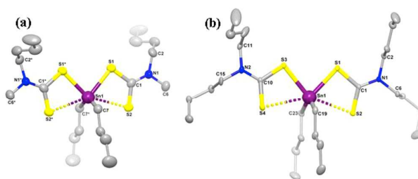
Fig 10. Molecular structures of (a) [Sn(C 4 H 9 ) 2 (S 2 CNMe n Bu) 2 ] and (b) [Sn(C 4 H 9 ) 2 (S 2 CN n Bu) 2 ] with 50% ellipsoidal probability level. All the H atoms on carbon frames are removed for clarity. Reproduced with permission from ref. 97. Copyright 2014 American Chemical Society.
