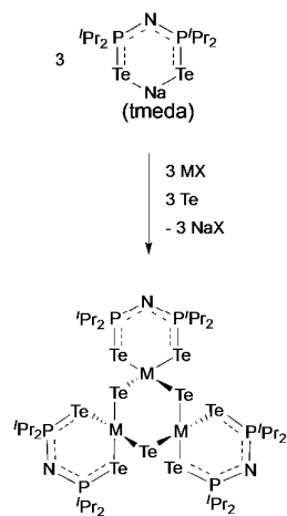
Scheme 3. General synthesis of [\text{Ga}(\mu\text{-Te})\{\text{N}(\text{TeP}'\text{Pr}_2)_2\}_3] ( \text{M} = \text{Ga} , \text{X} = \text{I} ) and [\text{In}(\mu\text{-Te})\{\text{N}(\text{TeP}'\text{Pr}_2)_2\}_3] ( \text{M} = \text{In} , \text{X} = \text{Cl} ).
