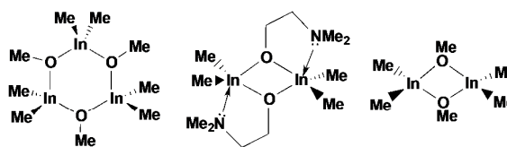
Fig. 22. Structures of dimethylindium alkoxides
