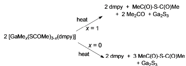
Scheme 2. Decomposition of [GaMe(SCOMe) 2 (dmpy)] and [Ga(SCOMe) 3 (dmpy)]
