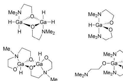
Fig. 20. Structural diagrams of \{[GaH_2(L_1)]_2\} and \{[GaH(L_2)]_2\} (where L = (Me_{3-x}N(CH_2CH_2O)_x) and x = 1, 2 ) and [Ga(L_1)_3] .
