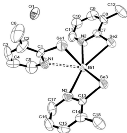
Fig. 16. Crystal structure of [\text{Bi}\{\{\text{Se-C}_5\text{H}_5(\text{Me-3})\text{N}\}_3\} \cdot 0.5\text{H}_2\text{O}] with atomic number scheme. Reproduced from ref. 121 with permission from The Royal Society of Chemistry.
