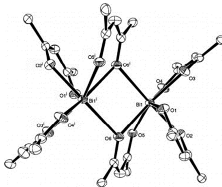
Fig. 30. X-ray crystallographic structure of [Bi(dbm) 3 ] 2 . Thermal ellipsoids set at 50% probability, phenyl rings, CH 2 Cl 2 solvent and hydrogen atoms omitted for clarity. Reproduced with permission from ref. 243. Copyright 2012 Elsevier.
