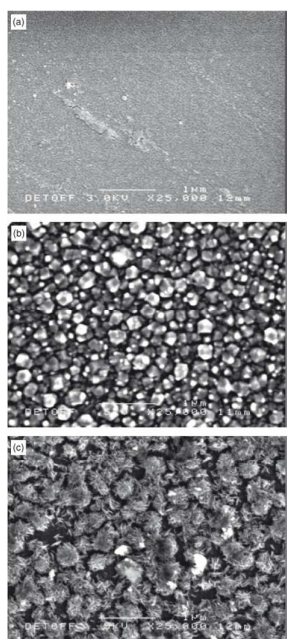
Fig. 24. SEM of films grown from AACVD deposition of InMe 3 and MeOH at (a) 400°C; (b) 450°C; and (c) 500°C. Reproduced with permission from ref. 176 Copyright 2013 Royal Australian Chemical Institute.
