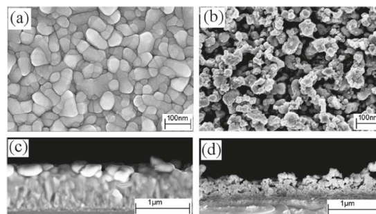
Fig. 14. SEM of \text{Bi}_2\text{S}_3 thin films deposited via AACVD from [\text{Bi}(\text{S}_2\text{CNET}_2)_3]_2 in chloroform/toluene at (a) 400 °C, (b) 450 °C, (c) and (d) show cross-section of films deposited at 400 and 450 °C, respectively. Reproduced with permission from ref. 114. Copyright 2014 American Chemical Society.
