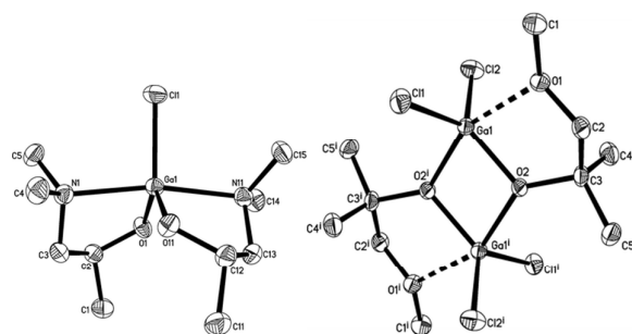
Fig. 18. Crystal structure of: left, [\text{Ga}(\text{OCH}(\text{CH}_3)\text{CH}_2\text{NMe}_2)_2\text{Cl}] , right, [\text{Ga}(\text{OC}(\text{CH}_3)_2\text{CH}_2\text{OMe})\text{Cl}_2] both with thermal ellipsoids shown at the 50% probability level (hydrogen atoms omitted for clarity). Reproduced from ref. 153 with permission from the Centre National de la Recherche Scientifique (CNRS) and the Royal Society of Chemistry.
