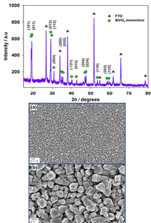
Fig. 35. XRD pattern of monoclinic \text{BiVO}_4 (green) on FTO (red) coated glass substrate deposited via AACVD; below: SEM image of \text{BiVO}_4 thin film at a) 20 000 X and b) 100 000 X. Reproduced with permission from ref. 248. Copyright 2012 Wiley.
