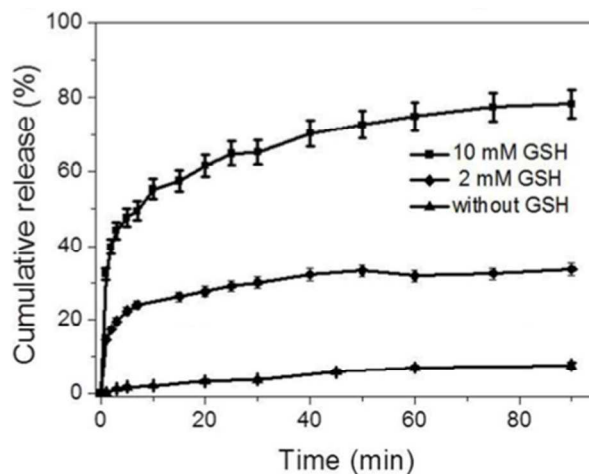
Fig.20 DOX release from DOX@MSN-S-S-RGD in PBS with different concentrations of GSH for 90 min. Reproduced from Ref. 362 with permission from the Royal Society of Chemistry.
