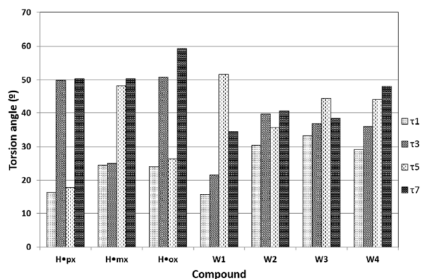
Fig. 8 Plot of torsion angles of Werner complexes based on values presented in Table 6
