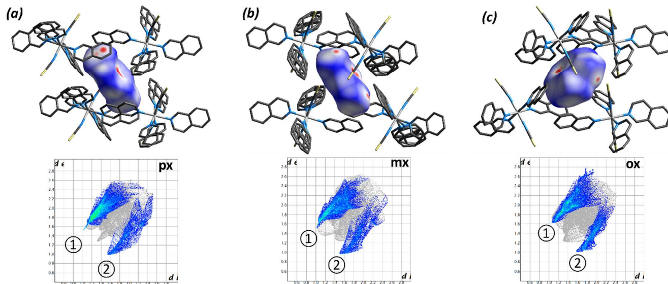
Fig. 2 Hirshfeld surfaces and their fingerprint plots of px (a), mx (b) and ox (c, ordered guest only); ① indicates close contacts between the guest hydrogens to the aromatic system of the host, while ② shows the contacts between the ligand hydrogens and the aromatic region of the guest.
