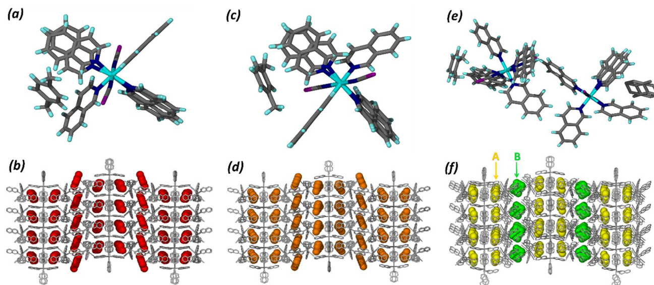
Fig. 1 Structural comparison of \mathbf{H}\cdot\mathbf{px} (a- molecular structure, b- packing viewed down c , \mathbf{px} is presented with spacefill model, red), \mathbf{H}\cdot\mathbf{mx} (c- molecular structure, d- packing viewed down c , \mathbf{mx} is presented with spacefill model, orange) and \mathbf{H}\cdot\mathbf{ox} (e- molecular structure, f- packing viewed down c , \mathbf{ox} is presented with spacefill model, yellow and green)
