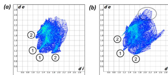
Fig. 6 Fingerprint plots for (a) ox guest and (b) mx guest in their inclusion compounds with bis(isothiocyanato) tetrakis(4-phenylpyridine) nickel (II)
