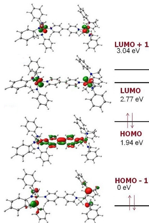
Fig. 3 Frontier MO energy levels calculated for model system (4,4'\text{-bipy})\{\text{Ti}(\text{N}[\text{Me}]\text{Ph})_3\}_2 . 16
