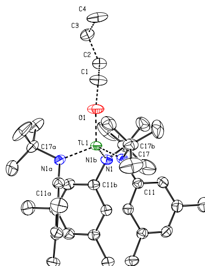
Fig. 10 Diagram of n -butoxy complex {}^nBuOTi(N[{}^tBu]Ar)_3 with 50% probability ellipsoids. 15 The molecule has a crystallographic C_3 axis coincident with the Ti-O vector and the n -butyl group occupies two positions (one shown).
