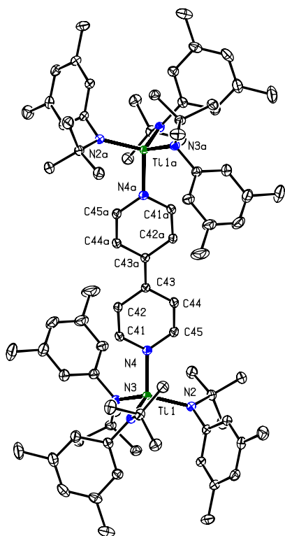
Fig. 2 Diagram of (4,4'\text{-bipy})\{\text{Ti}(\text{N}[\text{Me}]\text{Ph})_3\}_2 with thermal ellipsoids at the 50% probability level. 15
