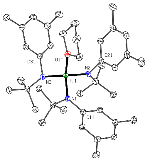
Fig. 9 Diagram of cation \{(THF)Ti(N[{}^tBu]Ar)_3\}^+ with 50% probability ellipsoids. 15 The [B(C_6F_5)_4]^- counter-anion, ether molecule of crystallization and hydrogen atoms are omitted for clarity (no close anion/cation contacts were observed).
