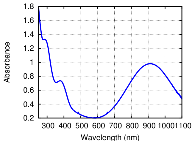
Fig. 4 Electronic absorption spectrum of (4,4'\text{-bipy})\{\text{Ti}(\text{N}[\text{ᵀBu}]\text{Ar})_3\}_2 as a solution in THF.
