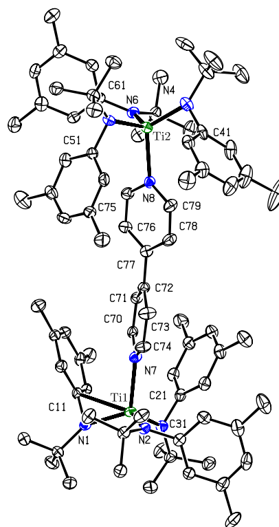
Fig. 7 Diagram (50% probability ellipsoids) of dication [(4,4'-bipy) \{\text{Ti}(\text{N}^t\text{BuAr})_3\}_2\}^{2+} with hydrogen atoms, [\text{B}(\text{C}_6\text{F}_5)_4]^- ions, and an o -difluorobenzene solvent molecule omitted. 15
