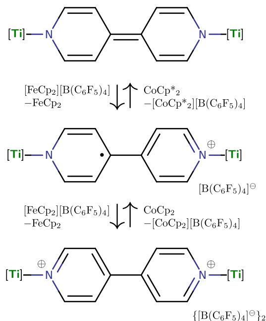
Fig. 6 Isolable in three states of charge, the figure depicts schematically (4,4'\text{-bipy})\{\text{Ti}(\text{N}[\text{ᵀBu}]\text{Ar})_3\}_2 , its mono-cation, and di-cation, the latter cations both having been isolated as perfluoro-tetraphenyl borate salts.
