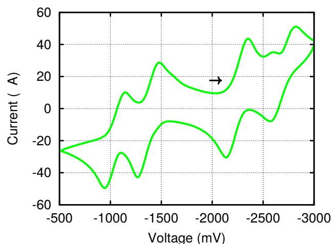
Fig. 5 Cyclic voltammogram for (4,4'\text{-bipy})\{\text{Ti}(\text{N}[\text{ᵀBu}]\text{Ar})_3\}_2 in THF with a sweep rate of 800 mV/s referenced vs. \text{Fc}/\text{Fc}^+ with [\text{N}^n\text{Bu}_4][\text{B}(\text{C}_6\text{F}_5)_4] (0.2 M) as the supporting electrolyte. The arrow signifies the rest potential and the direction of the sweep.
