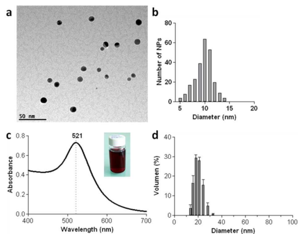
Fig. 2 Main features of the synthesized PEI-capped AuNPs (PEI-AuNPs). (a) TEM image and (b) size distribution histogram showing an average diameter of 9.8 ± 1.8 nm. (c) UV-Vis spectra showing the surface plasmon resonance at 521 nm with a representative photograph of the PEI-AuNPs in water (inset) and (d) hydrodynamic diameter.
