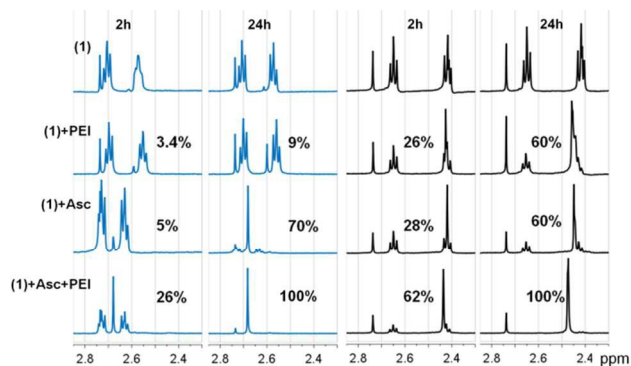
Fig. 1 Changes in 1 H NMR spectrum of ( 1 ) (1 mM) in D 2 O at pH 3-4 (blue) and pH 7 (black) in the presence and absence of PEI (10 μM) and ascorbic acid (10 mM).
