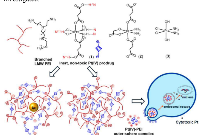
Scheme 1. Structure of PEI, (1), (2) and (3), plausible supramolecular synthons involved in the formation of PEI-(1) outer-sphere complexes and cancer killing mechanism.
