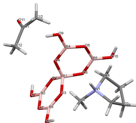
Fig. 4 Drawing of the structure of [\text{C}_4\text{H}_8\text{NMeH}][\text{B}_5\text{O}_6(\text{OH})_4] \cdot 1/2\text{C}_3\text{H}_6\text{O} ( 3 ) ( 1/2\text{C}_3\text{H}_6\text{O} ), showing the atomic numbering scheme.
