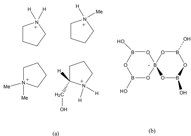
Fig. 1 Diagrams of the (a) pyrrolidinium cations and (b) the pentaborate(1-) anion, [\text{B}_5\text{O}_6(\text{OH})_4]^- , as found in [\text{C}_4\text{H}_8\text{NH}_2][\text{B}_5\text{O}_6(\text{OH})_4] ( 1 ), [\text{C}_4\text{H}_8\text{NMe}_2][\text{B}_5\text{O}_6(\text{OH})_4] ( 2 ), [\text{C}_4\text{H}_8\text{NMeH}][\text{B}_5\text{O}_6(\text{OH})_4] ( 3 ) and [(2\text{-CH}_2\text{OH})\text{C}_4\text{H}_7\text{NH}_2][\text{B}_5\text{O}_6(\text{OH})_4] ( 4 )
