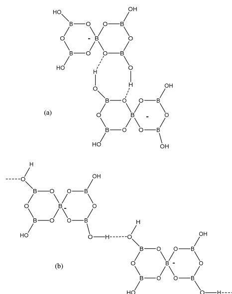
Fig. 6. H-bond interactions as found in 1-4 . (a) R 2 2 (8) reciprocal- \alpha , (b) C(8) \beta -chain.
