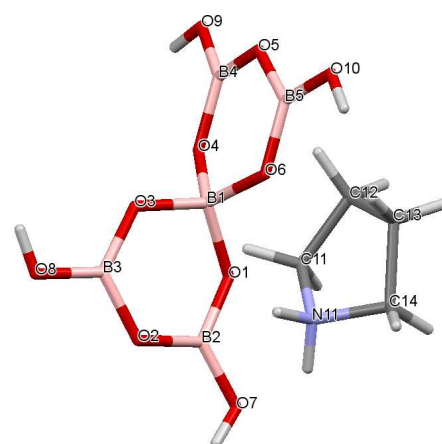
Fig. 2 Drawing of the structure of [\text{C}_4\text{H}_8\text{NH}_2][\text{B}_5\text{O}_6(\text{OH})_4] ( 1 ), showing the atomic numbering scheme.
