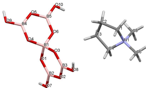
Fig. 3 Drawing of the structure of [\text{C}_4\text{H}_8\text{NMe}_2][\text{B}_5\text{O}_6(\text{OH})_4] ( 2 ) showing the atomic numbering scheme.
