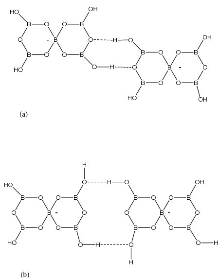
Fig. 7. H-bond interactions observed in pentaborate structures (a) R_2^2(8) reciprocal- \gamma (b) R_2^2(12) reciprocal- \beta
