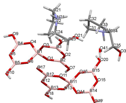
Fig. 5 Drawing of the structure of [2\text{-HOCH}_2\text{C}_4\text{H}_7\text{NHMe}][\text{B}_5\text{O}_6(\text{OH})_4] \cdot 1/2\text{H}_2\text{O} ( 4 ) ( 1/2\text{H}_2\text{O} ) showing the atomic numbering scheme.
