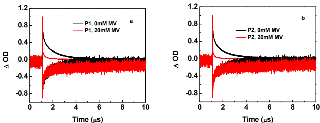
Figure 5. Absorbance bleach at 460 nm and emission decay at 630 nm for P1 (a) and P2 (b) with and without MV^{2+} (20 mM), following 425 nm excitation in degassed DMF. Ru(II) site concentration, 20 \mu M. The absorbance-traces for slow recovery of the bleach feature at 460 nm
