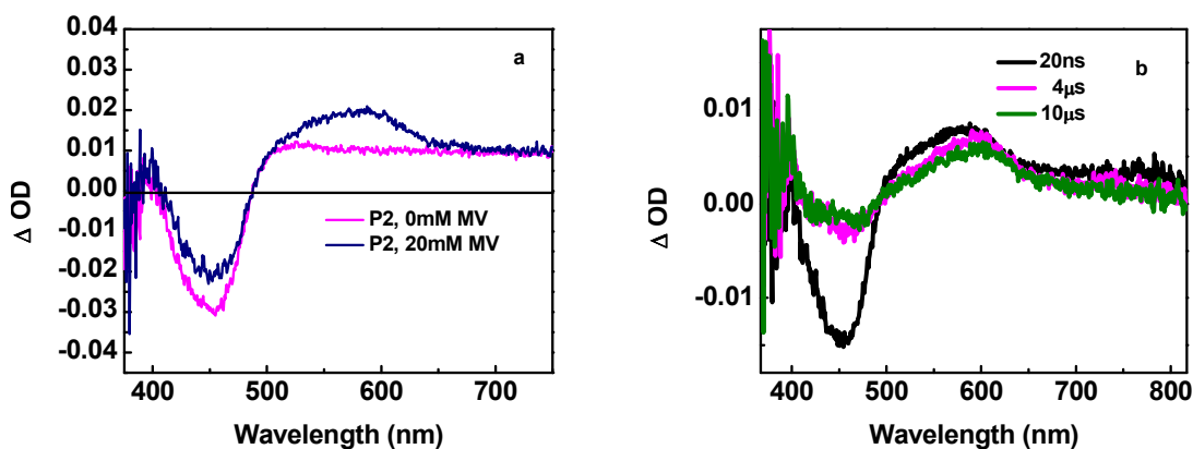
Figure 4. (a) Transition absorption difference spectra for P2 with and without added \text{MV}^{2+} in deaerated DMF obtained \sim 20 ns after 425 nm laser flash excitation, and (b) the spectra at different times following excitation. Ruthenium site concentration, 20 \mu\text{M} .
