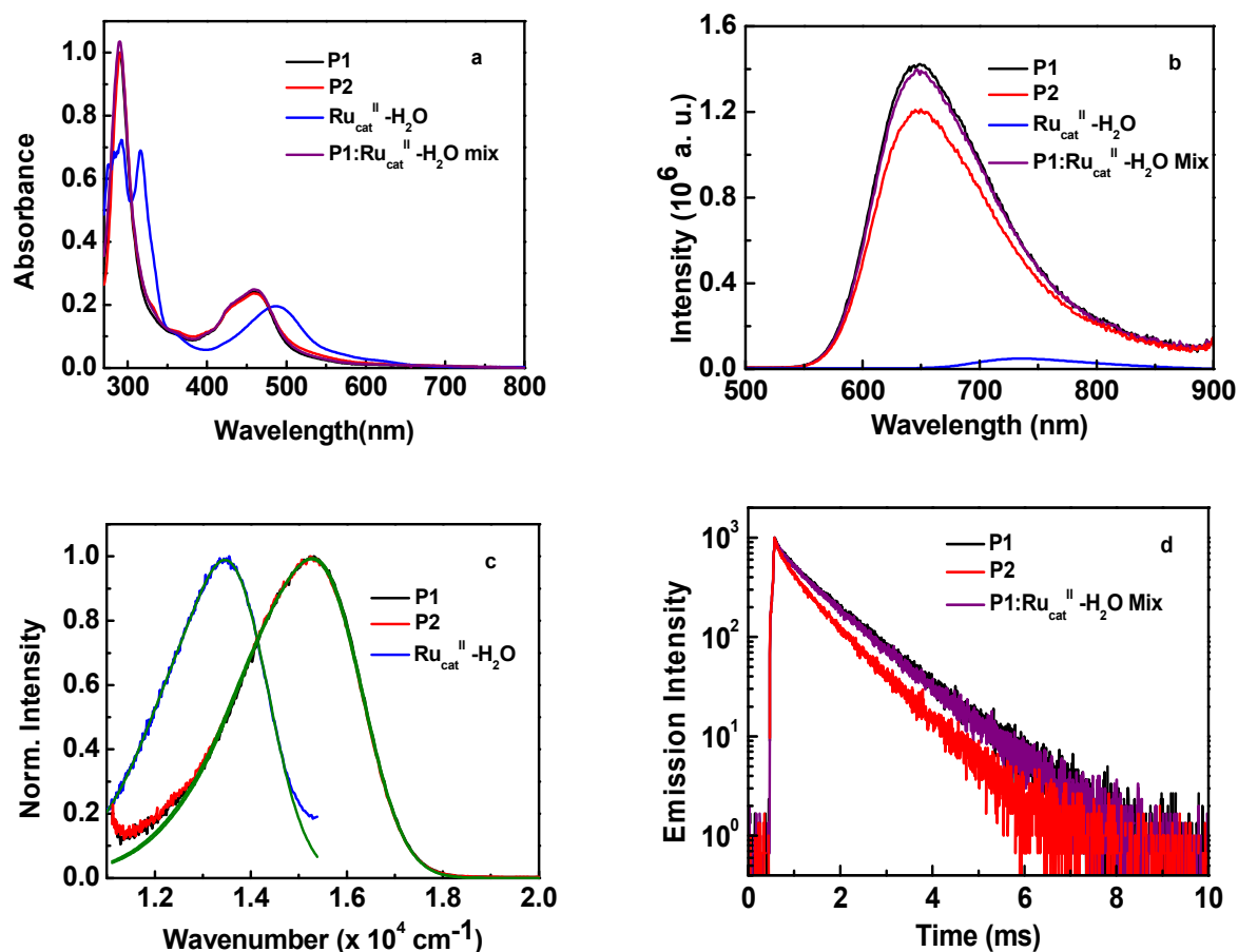
Figure 2. (a) Absorption and (b) emission spectra of P1 , P2 , Ru cat II -H 2 O ([[4'-phenyl-2,2':6',2''-terpyridine]Ru(bpy)(H 2 O)] 2+ ) and a mixture of P1 with Ru cat II -H 2 O, (c) wavenumber-scale emission spectra of P1 , P2 and Ru cat II -H 2 O at 298 K with simulated spectra (olive curves) obtained by single-mode Franck-Condon analysis of emission spectra (eq 1) with the fitting parameters listed in Table 1, and (d) emission decay profiles for P1 , P2 and the mixture of P1 and Ru cat II -H 2 O in DMF at 298 K monitored at 650 nm. Ru(II) concentration, 10 μM; Ratio of Ru(II) in P1 to Ru cat II -H 2 O in the mixed sample was 20:1; Excitation wavelength, 445 nm.
