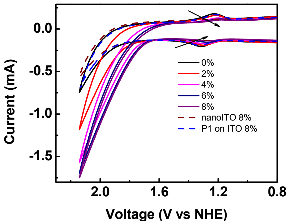
Figure 7. Cyclic voltammograms of P2 on nanoITO , in propylene carbonate 0%, 2%, 4%, 6%, and 8% added water by volume. Scan rate, 50 mV/s; 0.1 M \text{Bu}_4\text{NPF}_6 as the supporting electrolyte. The nanoITO electrode area is \sim 1 \text{ cm}^2 .
