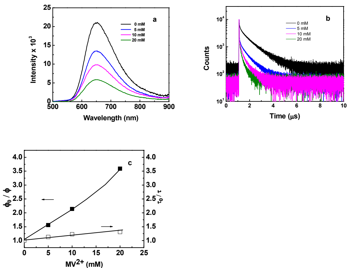
Figure 3. Emission spectra (a) and decay profiles (b) for P2 in the absence and presence of MV^{2+} . Stern-Volmer plots (c) for P2 quenched by pre-association (closed squares) and by diffusional quenching (open squares) by MV^{2+} . The concentration of Ru(II) sites in the DMF
