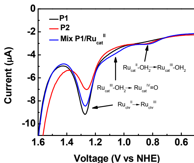
Figure 1. Differential pulse voltammograms of P1 , P2 and a P1/Ru cat II -H 2 O ([[4'-phenyl-2,2':6',2''-terpyridine]Ru(bpy)(H 2 O)] 2+ ) mixture (20:1) in deaerated 0.1 M Bu 4 NPF 6 propylene carbonate solution, scan rate: 50 mV/s.
