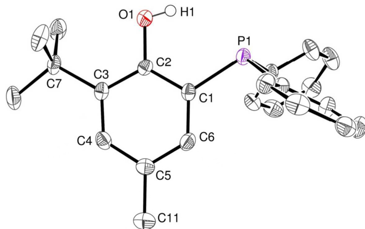
Figure 1. ORTEP drawing of the molecular structure of proligand 2 ·H. Thermal ellipsoids are set at the 50% probability level. Hydrogens are omitted for clarity except the crystallographically observed O-H1 hydrogen. Selected bond distances (Å): P1-C1 1.827(2), O1-C2 1.372(2), and angles (deg): O1-C2-C3 118.1(2), P1-C1-C6 124.0 (1), P1-C1-C2 117.3(1).
