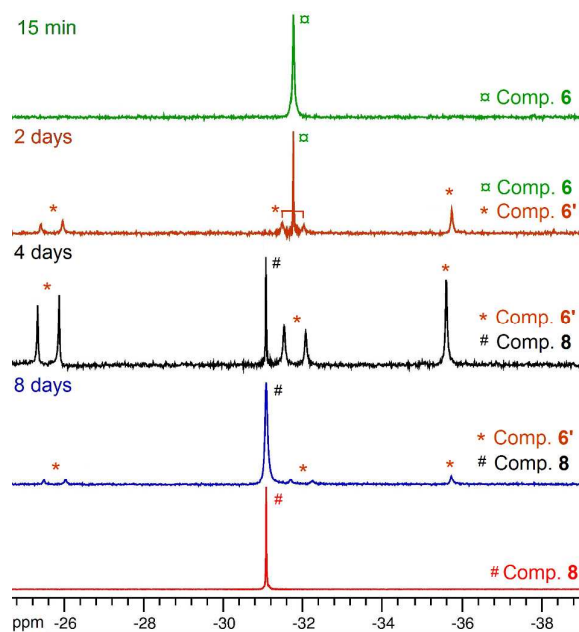
Scheme 2. Conversion of heteroleptic species 6 to homoleptic species 8 via the transient formation of 6' .
