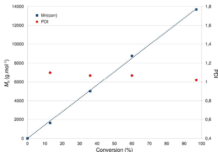
Figure 7. Linear dependence of M_n and PDI [ M_w/M_n ] of PLA versus monomer ( rac -LA) conversion with 5 as a catalyst. Reaction conditions: [Zn]/[LA]_0 = 100 , [LA]_0 = 1 M, CH_2Cl_2 , room temp.
