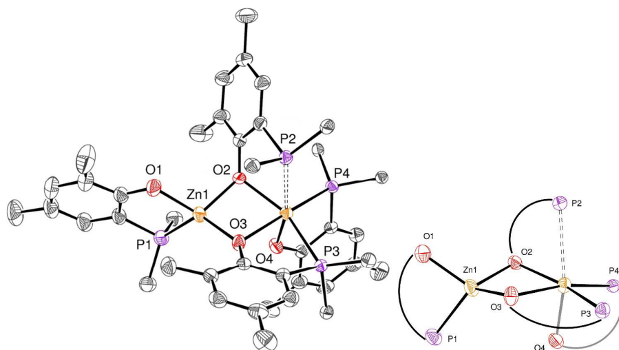
Figure 5. Left: ORTEP drawing of the molecular structure of 7 . Thermal ellipsoids are set at the 50% probability level. Hydrogen atoms are omitted and only the ipso -carbons of the PPh_2 rings are represented for clarity. Selected bond distances ( \text{\AA} ) around Zn1: Zn1-P1 2.393(9), Zn1-O1 1.936(1), Zn1-O2 1.973(2), Zn1-O3 1.946(2) and around Zn2: Zn2-P2 2.690(6), Zn2-O2 2.116(1), Zn2-P3 2.531(7), Zn2-O3 2.201(2), Zn2-P4 2.543(8), Zn2-O4 2.005(2) and angles (deg) around Zn1: P1-Zn1-O1 86.77(6), O2-Zn1-O3 87.52(7) and around Zn2: P2-Zn2-O2 73.72(5), P2-Zn2-P3 97.43(2), P3-Zn2-O4 94.68(5), O4-Zn2-O2 92.81(7), P4-Zn2-O3 168.05(5). Right: a zoom on the different coordination environment for Zn1 and Zn2.
