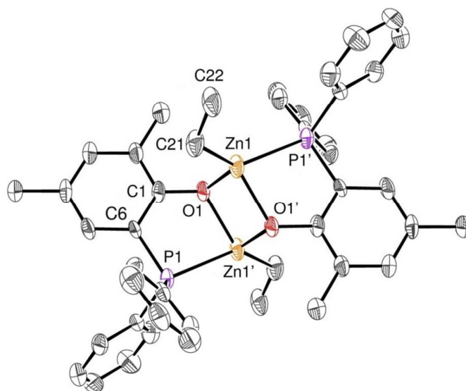
Figure 2. ORTEP drawing of the molecular structure of 3 . Thermal ellipsoids are set at the 50% probability level. Hydrogen atoms are omitted for clarity. Selected bond distances (Å): \text{Zn1-P1'} 2.458(3), \text{Zn1-O1'} 2.069(5), \text{Zn1-C21} 1.985(8), \text{Zn1-O1} 2.058(6), \text{O1-C1} 1.358(6), \text{P1-C6} 1.796(7) and angles (deg): \text{O1-Zn1'-P1} 80.31(1), \text{O1-Zn1-C21} 113.6(3), \text{P1'-Zn1-C21} 133.3(2), \text{O1-Zn1-P1'} 103.8(1), \text{O1'-Zn1-C21} 130.0(3), \text{O1-Zn1-O1'} 82.6(2).
