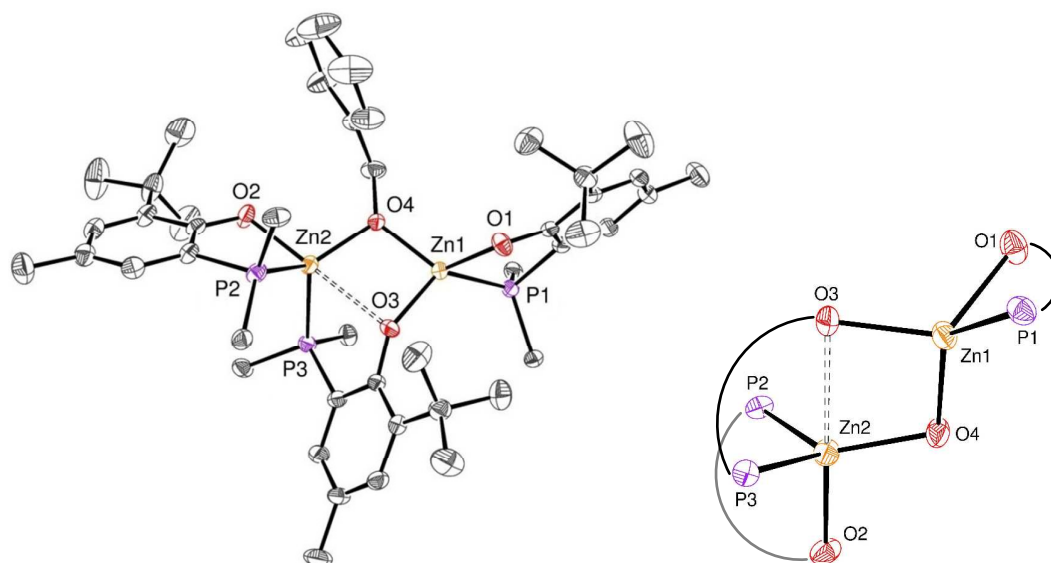
Figure 4. Left: ORTEP drawing of the molecular structure of 6' . Thermal ellipsoids are set at the 50% probability level. Hydrogen atoms are omitted and only the ipso -carbon of each P-phenyl ring is
