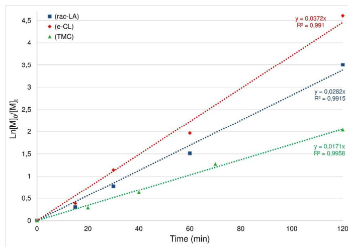
Figure 6. Semilogarithmic plots of rac -LA (blue), \epsilon -CL (red) and TMC (green) conversion versus time for complex 5 . Reaction conditions: [\text{Zn}]/[\text{M}]_0 = 100 , [\text{M}]_0 = 1 \text{ M} , \text{CH}_2\text{Cl}_2 , room temp.
