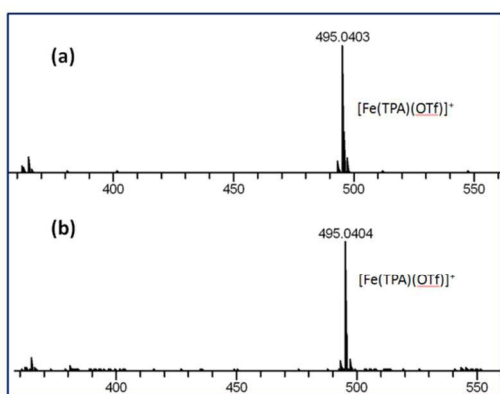
Figure 11. Mass spectra of (a) \text{Fe}(\text{TPA})(\text{CH}_3\text{CN})_2(\text{OTf})_2 2 mM; (b) \text{Fe}(\text{TPA})(\text{CH}_3\text{CN})_2(\text{OTf})_2 2 mM, \text{Zn}(\text{OTf})_2 4 mM in acetonitrile.
