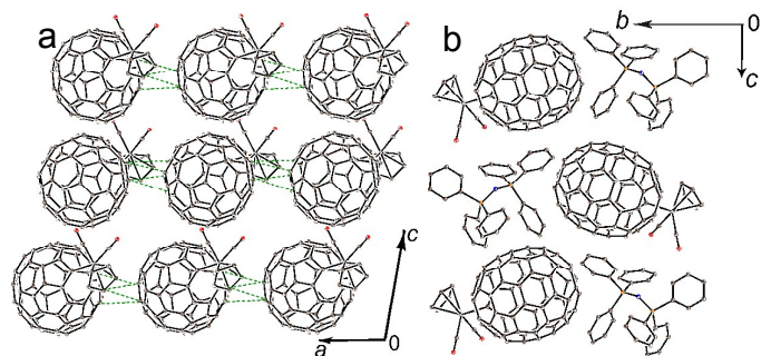
Fig. 5 View on anionic \{\text{CpMo}(\text{CO})_2(\eta^2\text{-C}_{70})\}^- layers (a) and along these layers (b) in 2 . Short van der Waals C...C contacts are shown by green dashed lines.
