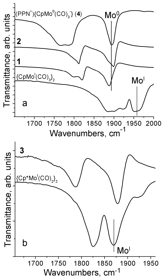
Fig. 2 The position of the absorption bands of the CO stretching mode: (a) the reference compound (\text{PPN}^+)\{\text{CpMo}^{\text{0}}(\text{CO})_3\}^- ( 4 ), the \{\text{CpMo}^{\text{I}}(\text{CO})_3\}_2 dimer and complexes 1 and 2 ; (b) the \{\text{Cp}^*\text{Mo}^{\text{I}}(\text{CO})_2\}_2 dimer and complex 3 . The Royal Society of Chemistry 2012
