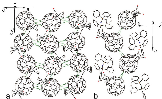
Fig. 4 View on anionic \{\text{CpMo}(\text{CO})_2(\eta^2\text{-C}_{60})\}^- layer in 1 (a) and view along this layer (b). Short van der Waals C...C contacts are shown by green dashed lines.
