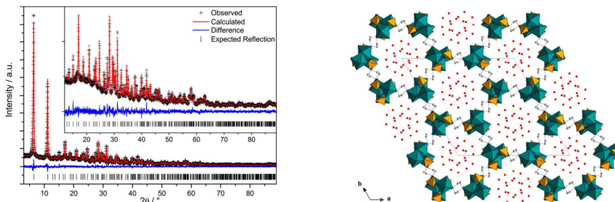
Fig. 6. Rietveld plot of STA-12(Cd) (left) obtained from flow reactor and the structure determined (right). The final cycle of refinement gave R_{wp} = 6.43\% , R_{Bragg} = 1.56\% and \chi^2 = 1.141
