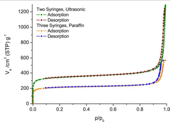
Fig. 2. \text{N}_2 adsorption and desorption isotherms measured at 77 K on samples of UiO-66 produced in a two-pump (ultrasonic probe; green & red traces) and three-pump (paraffin transport; orange & blue traces) flow reactor.
