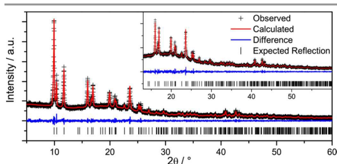
Fig. 3. Pawley fit of CAU-13 obtained from a flow reactor in a two-syringe configuration. Cell refined to a = 6.6111(4) Å, b = 9.4498(6) Å, c = 9.4652(5) Å, \alpha = 107.652(4)^\circ , \beta = 107.690(6)^\circ and \gamma = 93.185(5)^\circ (space group: P\bar{1} ; R_{wp} = 4.71\% , \chi^2 = 1.080 ), consistent with reported lattice parameters. 21
