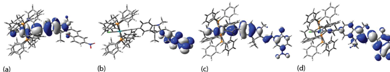
Figure 1. Plots of the (a) HOMO and (b) LUMO of 2-SP and (c) HOMO and (d) LUMO of 2-MC ( \pm 0.02 (e/bohr 3 ) 1/2 ).
