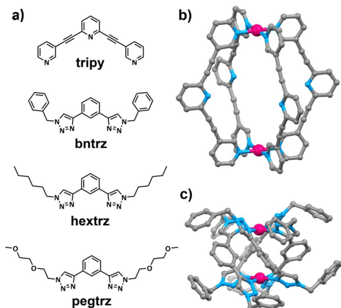
Figure 1 a) Chemical structures of the pyridine- ( tripy ) and triazole- ( bntrz , hextrz and pegtrz ) based ligands; the molecular structures of b) [\text{Pd}_2(\text{tripy})_4](\text{BF}_4)_4 26 and c) [\text{Pd}_2(\text{bntrz})_4](\text{BF}_4)_4 24h architectures. Anions, solvent molecules and hydrogen atoms have been omitted for clarity.
