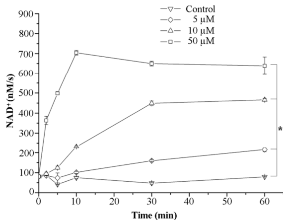
Figure 4. [\text{Pd}_2(\text{hextrz})_4](\text{BF}_4)_4 causes rapid disruption of the cell membrane. A549 cells were treated with [\text{Pd}_2(\text{hextrz})_4](\text{BF}_4)_4 and the change in extracellular LDH levels calculated by measuring enzyme activity. Data represents extracellular LDH activity at each time point and are expressed as means \pm SEM ( n=3 ). *=p<0.05 .
