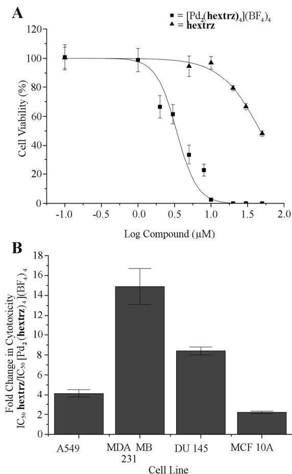
Figure 2. [Pd_2(\text{hextrz})_4](BF_4)_4 cytotoxicity is not due to helicate decomposition. Cells were treated with [Pd_2(\text{hextrz})_4](BF_4)_4 or \text{hextrz} for 24 hours before cell viability analysis. (A) Against DU-145 cells the IC_{50} for the ligand ( 28.5 \mu\text{M} ) was 8 fold higher than for the helicate ( 3.4 \mu\text{M} ); if helicate toxicity was due to rapid decomposition to release the ligand, then the stoichiometry of the complex would predict a 4-fold ratio in IC_{50} . (B) A comparison of the IC_{50} ratio between ligand and helicate across the four cell lines demonstrated no correlation between helicate and ligand toxicity. Data points are expressed as means \pm SEM where n=6 .
