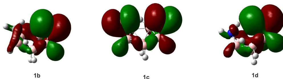
Figure 3 HOMO for 1b-1d at HF/6-311+G(d,p).
