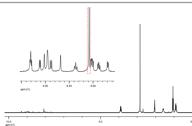
Fig. 2 ^1\text{H} NMR spectrum of dinuclear complex [\text{Re}(\text{OEt})\text{Re}(\text{Et})]^{2+} . The solvent was acetone- d_6 . The red square emphasises the peak attributed to olefin protons.
