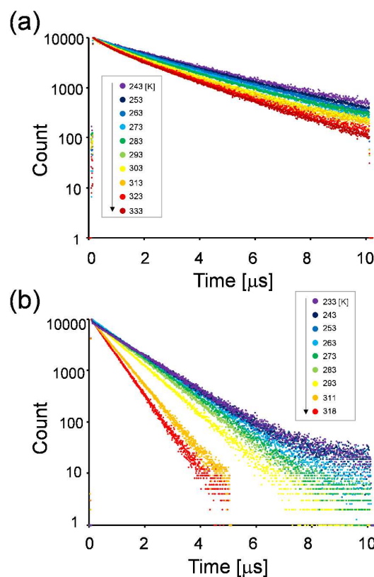
Fig. 5 (a) Temperature dependence of emission decay of [Ru(dmb) 2 Re(Ph)] 5+ . Decay curves were measured from 243 K (purple) to 333 K (dark red). Excitation wavelength was 456 nm and detection wavelength was 738 nm. (b) Temperature dependence of emission decay of [Ru(dmb) 2 ] 2+ . Decay curves were measured from 233 K (purple) to 318 K (red). Excitation wavelength was 456 nm and detection wavelength was 639 nm. The solvent was MeCN.
