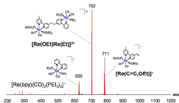
Fig. 1 ESI-MS spectrum of crude products measured after the synthesis of [\text{Re}(\text{OEt})\text{Re}(\text{Et})]^{2+} . The mobile phase was MeCN.
