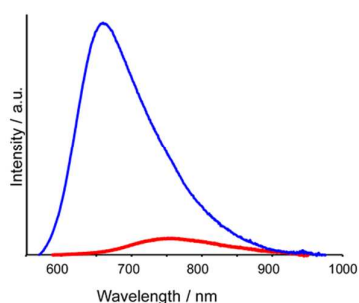
Fig. 4 Emission spectra of [Ru(C=C, dmb)] 2+ (blue) and [Ru(dmb) 2 Re(Ph)] 5+ (red) measured in MeCN (excitation wavelength: 456 nm).
