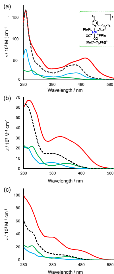
Fig. 3 UV-Vis absorption spectra of obtained trinuclear complexes and corresponding mononuclear complexes. The solvent was MeCN. (a) [\text{Ru}(\text{dmb})_2\text{Re}(\text{Ph})]^{5+} (red), [\text{Ru}(\text{C}=\text{C}, \text{dmb})]^{2+} (blue), [\text{Re}(\text{C}=\text{C}, \text{Ph})]^+ (green) and the 2:1 summation spectrum of [\text{Ru}(\text{C}=\text{C}, \text{dmb})]^{2+} and [\text{Re}(\text{C}=\text{C}, \text{Ph})]^+ (dotted line). (b) [\text{Re}(\text{OEt})_2\text{Re}(\text{Ph})]^{3+} (red), [\text{Re}(\text{C}=\text{C}, \text{OEt})]^+ (blue), [\text{Re}(\text{C}=\text{C}, \text{Ph})]^+ (green) and the 2:1 summation spectrum of [\text{Re}(\text{C}=\text{C}, \text{OEt})]^+ and [\text{Re}(\text{C}=\text{C}, \text{Ph})]^+ (dotted line). (c) [\text{Ir}(\text{ppy})_2\text{Re}(\text{Ph})]^{3+} (red), [\text{Ir}(\text{C}=\text{C}, \text{ppy})]^+ (blue), [\text{Re}(\text{C}=\text{C}, \text{Ph})]^+ (green) and the 2:1 summation spectrum of [\text{Ir}(\text{C}=\text{C}, \text{ppy})]^+ and [\text{Re}(\text{C}=\text{C}, \text{Ph})]^+ (dotted line).
