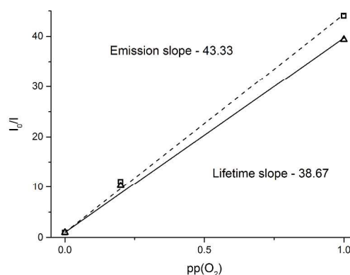
50 Figure 6. Stern-Volmer plot of the relative emission intensities (squares) and lifetimes (triangles) against the partial pressure of oxygen in solution. Estimated error in I_0/I based on 3 repeat measurements = \pm 2\% , calculated lifetime error < \pm 1\% in all measurements and R^2 = 0.99 for both plots.
