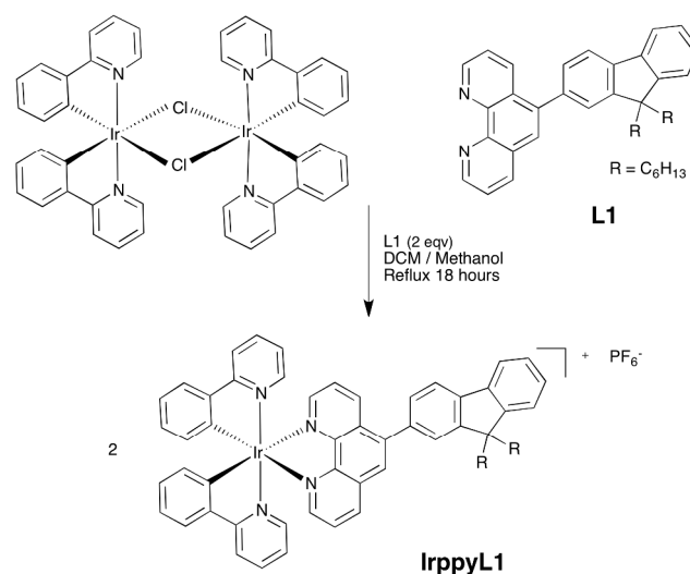
Figure 1. Synthesis of [\text{Ir}(\text{ppy})_2(\text{L1})][\text{PF}_6] ( IrppyL1 ) from the chloro-bridged Ir(III) ppy dimer and ligand L1 ( \text{R} = \text{C}_6\text{H}_{13} )
