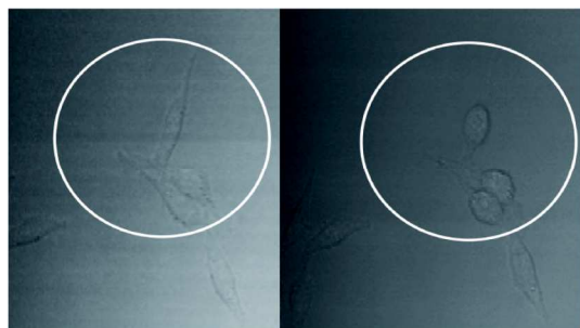
Figure 8. Cells treated with 1 mM IrppyL1 before (left) and after (right) 5 minutes irradiation (one such irradiation area of the whole sample irradiated is in the white circle) at 740 nm, 32.5 \mu W during 6 cycles) and 15 minutes wait - the morphology of the cells on the right has become rounded compared to the elongated shape of the healthy cells. Spot area = 0.13 \mu m which equates to an area of 0.0169 \mu m 2 . The irradiation time per cycle = 50 s, the total light dose per pixel (1.91 e^{-4} s duration) = 3.72 e^{-8} J, which equates to 220 J/cm 2 .
