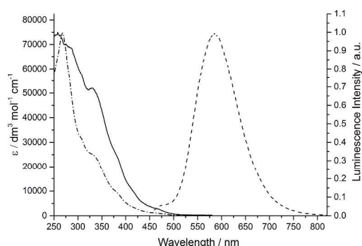
Figure 3. Absorption (solid line), emission (dashed line) and excitation (dot-dashed line) spectra for IrppyL1 in degassed acetonitrile at 2 \times 10^{-5} M concentration (excitation at 400 nm, emission at 590 nm).
