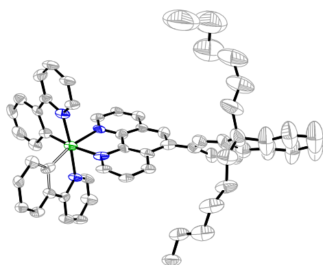
Figure 2. Molecular structure of [\text{Ir}(\text{ppy})_2(\text{L1})]\text{PF}_6 with thermal ellipsoids set at the 50% probability level. H atoms, counterions and the second molecule in the asymmetric unit removed for clarity.
