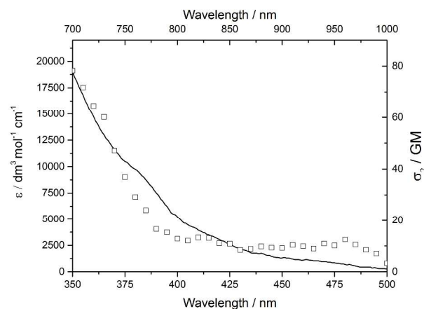
Figure 7. Two-photon excitation (marked squares) and linear excitation (solid line) spectra of IrppyL1 in degassed acetonitrile. (One-photon at 2 × 10 -5 M, two-photon measurement at a concentration of 4 × 10 -5 M, measured by two photon excited fluorescence (2PEF) referenced to fluorescein in 0.01 M NaOH, 1 × 10 -4 M)
