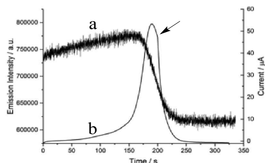
30 Figure 5. Emission intensity (a) and electrochemical current (b) traces for IrppyL1 (1 mM in acetonitrile with NEt 4 PF 6 electrolyte) as a function of time upon linear potential sweep (5 mV/s). The arrow shows the time corresponding to the potential reversal.
