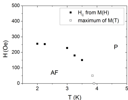
Figure 7. Magnetic phase diagram of 2 .
