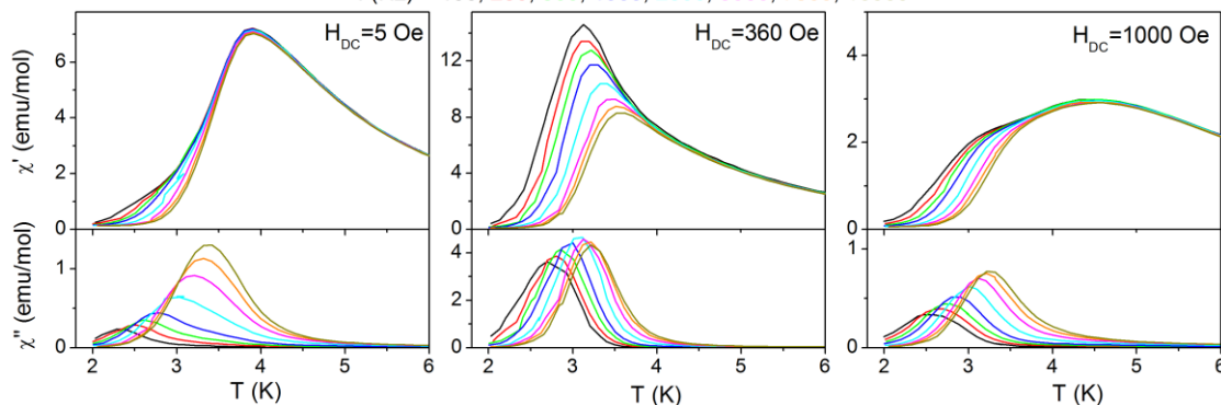
Figure 8. Temperature dependent AC magnetic susceptibilities for 2 measured for various frequencies in different DC magnetic fields.
