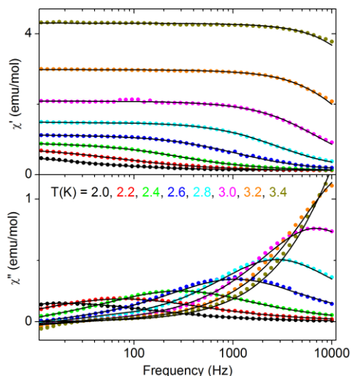
Figure 9. Frequency dependent AC susceptibility for 2 measured at various temperatures. Solid lines are fits with the generalized Debye model.
