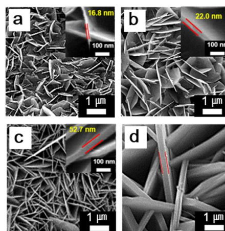
Fig. 2 SEM images of \text{Co}(\text{OH})_2 with reaction times of (a) 20 min, (b) 40 min (two 20 min reactions), (c) 6 h, and (d) 18 h.
