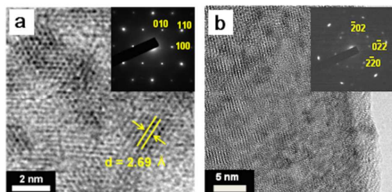
Fig. 8 HRTEM images of (a) Co(OH) 2 -6h (a) and (b) GO-wrapped Co(OH) 2 -6h. Inset images are ED patterns.
