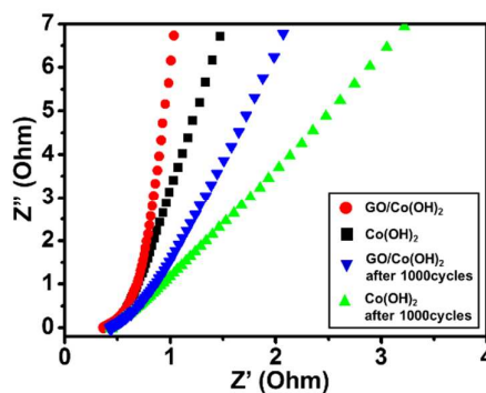
Fig. 7 Nyquist plots of \text{Co(OH)}_2\text{-6h} and GO/ \text{Co(OH)}_2\text{-6h} at 0.3 \text{ V} in the low frequency region.
