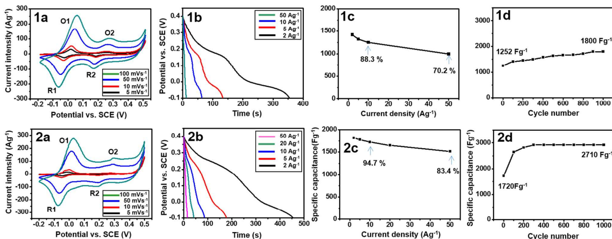
Fig. 6 Electrochemical characterization of (1) \text{Co(OH)}_2\text{-40m} and (2) GO-wrapped \text{Co(OH)}_2\text{-40m} . (a) CV curves, (b) galvanostatic discharge curves, (c) specific capacitance versus current density, and (d) plots of specific capacitance versus cycle number at 10 \text{ A g}^{-1} .
