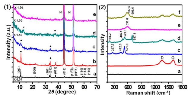
Fig. 9 (1) XRD patterns of (a) Co(OH) 2 powder, (b) Co(OH) 2 on Ni-metal substrate (Co(OH) 2 -6h), (c) GO-Co(OH) 2 -6h, (d) Co(OH) 2 -6h after 1000 cycles, and (e) GO-Co(OH) 2 -6h after 1000 cycles, (● = \alpha -Co(OH) 2 and ▼ = \gamma -CoOOH). (2) Raman spectra of (a) Ni-metal substrate, (b) GO on glass, (c) Co(OH) 2 -6h, (d) GO-Co(OH) 2 -6h, (e) Co(OH) 2 -6h after 1000 cycles, and (f) GO-Co(OH) 2 -6h after 1000 cycles.
