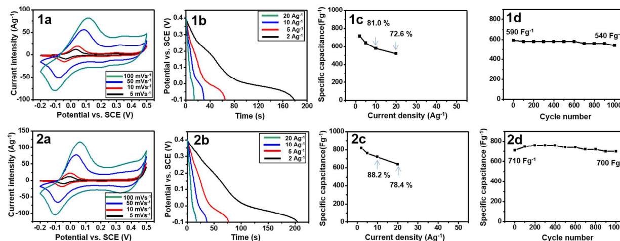
Fig. 5 Electrochemical characterization of (1) \text{Co(OH)}_2\text{-6h} and (2) \text{GO-wrapped Co(OH)}_2\text{-6h} . (a) CV curves, (b) galvanostatic discharge curves, (c) specific capacitance versus current density, and (d) plots of specific capacitance versus cycle number.
