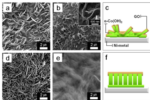
Fig. 4 SEM images and schematic illustrations of (a) \text{Co(OH)}_2 -40m, (b, c) \text{GO-Co(OH)}_2 -40m, (d) \text{Co(OH)}_2 -6h, and (e, f) \text{GO-Co(OH)}_2 -6h.
