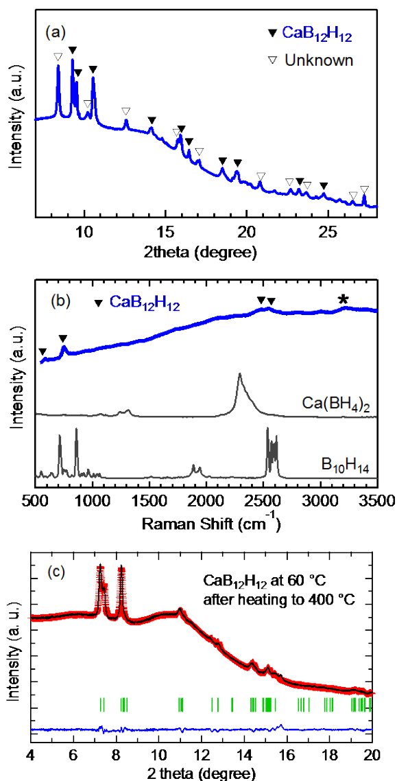
Figure 2. (a) Synchrotron XRD ( \lambda = 1.00117 \text{ \AA} ) pattern and (b) Raman spectra of 5 h ball milled \text{Ca}(\text{BH}_4)_2 + \text{B}_{10}\text{H}_{14} followed by sintering at 380 °C for 2 h. Asterisk indicates the systematic error. (c) Rietveld refinement plot for \text{CaB}_{12}\text{H}_{12} at 60 °C after heating to 400 °C. Red crosses and black line show the experimental and calculated data, respectively. Blue line is the difference profile, and green marks indicate Bragg positions of \text{CaB}_{12}\text{H}_{12} .
