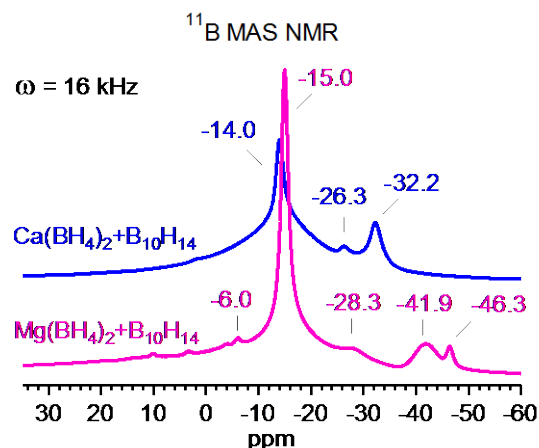
Figure 3. ^{11}\text{B} MAS NMR spectra of synthesized samples from \text{M}(\text{BH}_4)_2 + \text{B}_{10}\text{H}_{14} (M = Mg: 5 h ball milling followed by sintering at 300 °C for 1 h; M = Ca: 5 h ball milling followed by sintering at 380 °C for 2 h).
