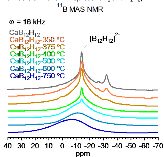
Figure 7. ^{11}\text{B} MAS NMR spectra of \text{CaB}_{12}\text{H}_{12} as synthesized and heated up to respective temperatures.
