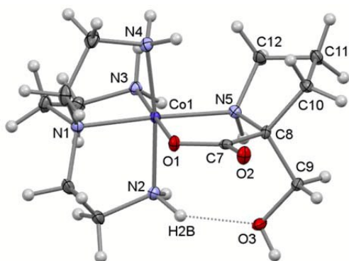
Fig. 3 A view of the molecular structure of the complex cation of [\mathbf{23}]\text{Cl}_2 \cdot 2\text{H}_2\text{O} showing the atom-labelling scheme for selected atoms. Displacement ellipsoids are drawn at the 50% probability level and H atoms are shown as small spheres of arbitrary radii.
