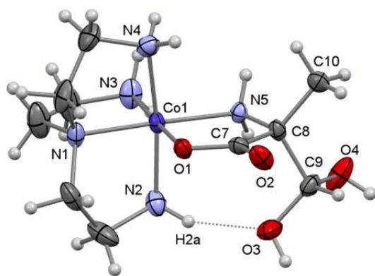
Fig. 1 A view of the molecular structure of one of the two crystallographically independent but structurally similar complex ions of [\mathbf{17}]_2 \cdot \text{H}_2\text{O} showing the atom-labelling scheme for selected atoms. Displacement ellipsoids are drawn at the 30% probability level and H atoms are shown as small spheres of arbitrary radii.
