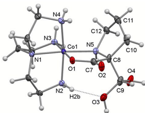
Fig. 2 A view of the molecular structure of the complex cation of [\mathbf{22}]\text{Cl}_2 \cdot 2\text{H}_2\text{O} showing the atom-labelling scheme for selected atoms. Displacement ellipsoids are drawn at the 50% probability level and H atoms are shown as small spheres of arbitrary radii.
