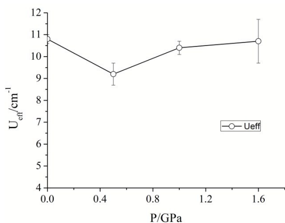
Figure 5. Variation of the barrier to relaxation U_{\text{eff}} of 1 under an applied dc field of 2500 Oe as a function of pressure.
