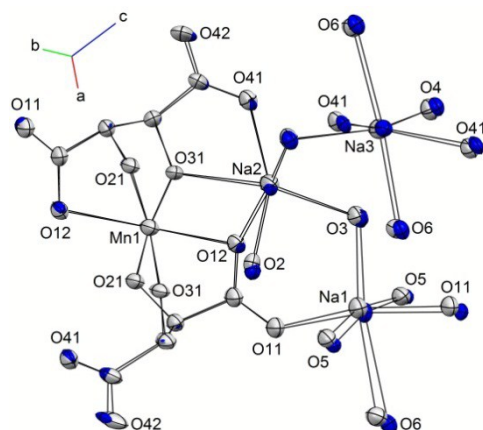
Figure 3. Overlay of the structure of 1 at 0.34 GPa (blue) and 3.49 GPa (light grey). Ellipsoids are shown at the 30 % probability level, hydrogen atoms are omitted for clarity, and only heteroatoms are labelled.
