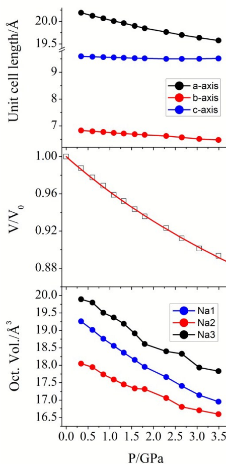
Figure 2. (top) Variation of the crystallographic unit cell lengths in 1 as a function of applied pressure. (middle) Pressure dependence of the relative unit cell volume of 1 . The value at P = 0 is taken from the original crystal structure determination, 18 and the solid line is a fit to a Birch-Murnaghan equation of state. (bottom) The pressure dependence of the octahedral volume around the \text{Na}^+ ions in 1 .
