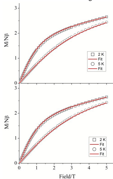
Figure 4. Magnetisation of 1 as a function of applied field at (top) ambient pressure inside the pressure cell and (bottom) 1.6 GPa. Solid lines correspond to fits of the data, performed with the program Phi.
