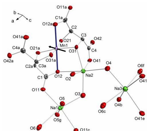
Figure 1. The structure of 1 at 0.34 GPa. Ellipsoids are shown at the 70 % probability level, and hydrogen atoms are omitted for clarity. The Jahn-Teller axis is shown with thicker bonds. The black arrow represents the largest component of the strain tensor (see text). Lower case letters represent the symmetry operations for duplicate atoms: a = (1-x, y, -z), b = (1-x, y, 1-z), c = (1.5-x, 0.5+y, 1-z), d = (x, -1+y, z), e = (1-x, -1+y, 1-z), f = (-0.5+x, -0.5+y, z), g = (1.5-x, 0.5+y, 1-z).
