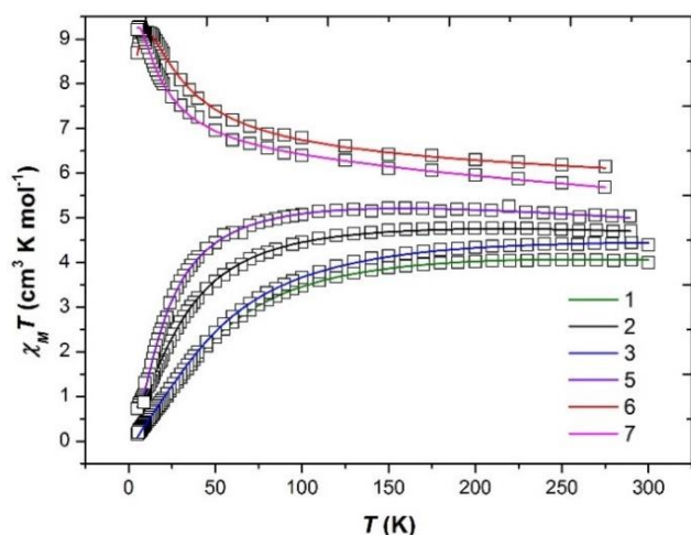
Figure 4. Plot of the \chi_M T product versus T for complexes 1-3 , 5-7 . The solid lines are a fit of the experimental data to isotropic spin-Hamiltonian ( 1 ). See text for details of the best fit parameters. Green = 1 , black = 2 , blue = 3 , purple = 5 , red = 6 and pink = 7 .
