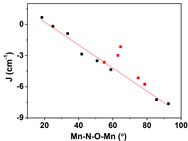
Figure 7. Magneto-structural correlations developed by varying the Mn-N-O-Mn dihedral angle in 1 . The red squares are experimental J values obtained for complexes 1-5 .
