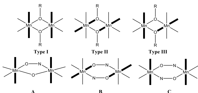
Figure 1. Top: alkoxide bridged dimers [Mn III (OR)] 2 with Type I–III structures differing in the relative orientations of the Jahn-Teller axes, which are highlighted in bold. Bottom: oxime/oxo dimers [Mn III 2 (O)(NO)] ( A ), and the double oxime bridged dimers [Mn III (NO)] 2 in which the Jahn-Teller axes lie in the bridging plane ( B ), and perpendicular to the bridging plane ( C ).
