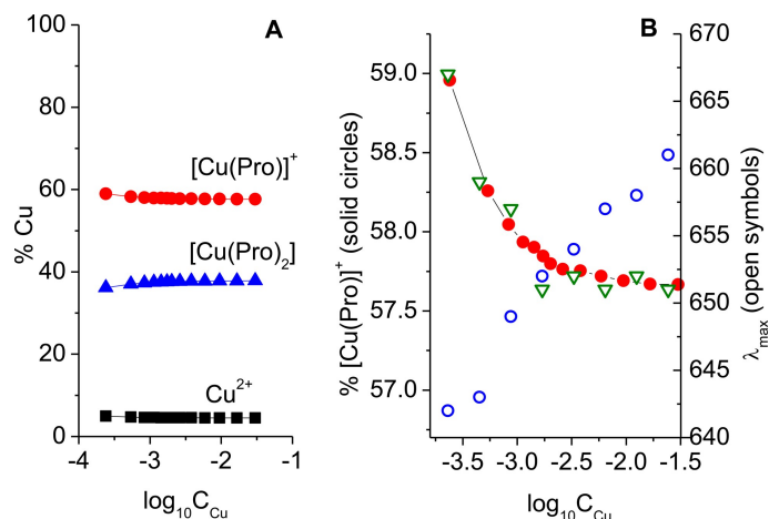
Fig. 11 A: Speciation diagram of the Cu^{2+} /proline system ( Cu:Pro = 6:8 , C_{Cu} = 30 mM, unbuffered solution). B: Red circles: plot of the % [Cu(Pro)]^+ in the system Cu:Pro = 6:8 at different total Cu^{2+} concentrations (red circles). Green triangles: experimental \lambda_{max} values for the dilution of a solution of 1(Na) in water, and in methanol (blue circles).
