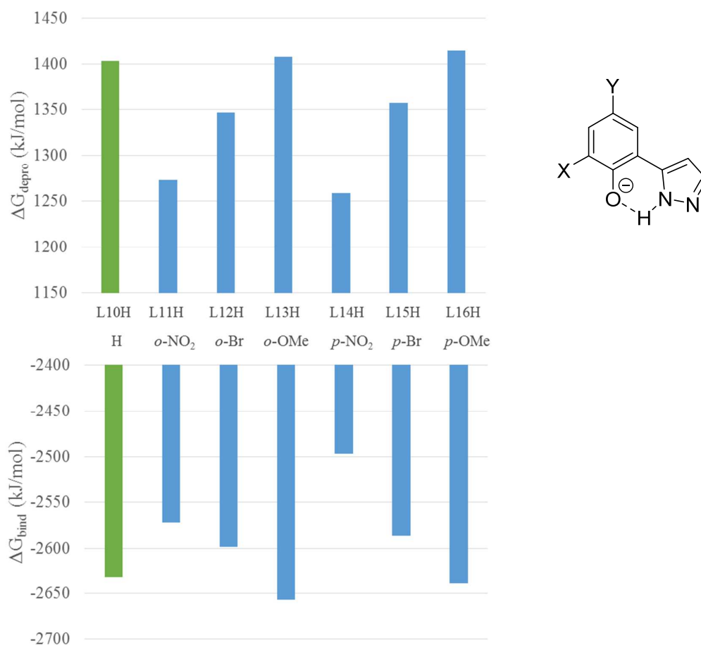
Figure 5: Gibbs free energies of deprotonation of two proligand molecules ( \Delta G_{\text{depro}} , Equation 3) are shown in the upper chart) and those of binding of two ligand anions to \text{Cu}^{2+} ( \Delta G_{\text{bind}} , Equation 4), lower chart) for L10H-L16H, together with the structure of the most stable tautomer of the ligand anions used in calculations.
