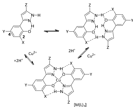
Figure 1: Hydrogen-bonding in proligand monomers and dimers and in copper(II) complexes of substituted phenolic pyrazoles. Outer sphere interactions in the complex are shown by dashed lines.
