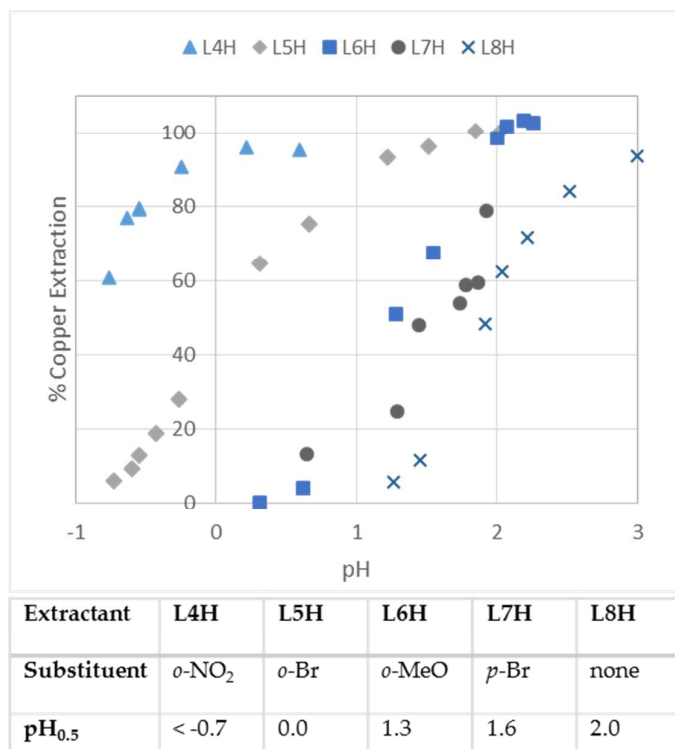
Figure 3: The pH dependence of Cu-loading by 0.005 M chloroform solutions of L4H-L8H from equal volumes of 0.005 M aqueous solution of \text{CuSO}_4 and the \text{pH}_{0.5} values of the extractants; 100% Cu-loading is based on the formation of a \text{CuL}_2 complex.
