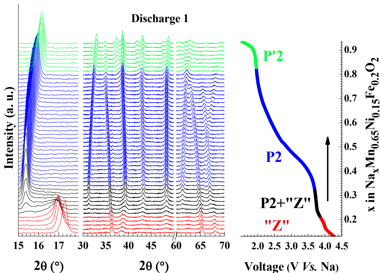
Figure 4: Operando XRD data recorded during galvanostatic cycling of \text{Na}_{0.67}[\text{Mn}_{0.65}\text{Ni}_{0.15}\text{Fe}_{0.2}]\text{O}_2 at a rate of C/20 (left) along with illustration of sodium content vs. voltage of the cell (right) for the first discharge. The traces in the operando XRD patterns are colour-coded with respect to the electrochemical profile on the right.
