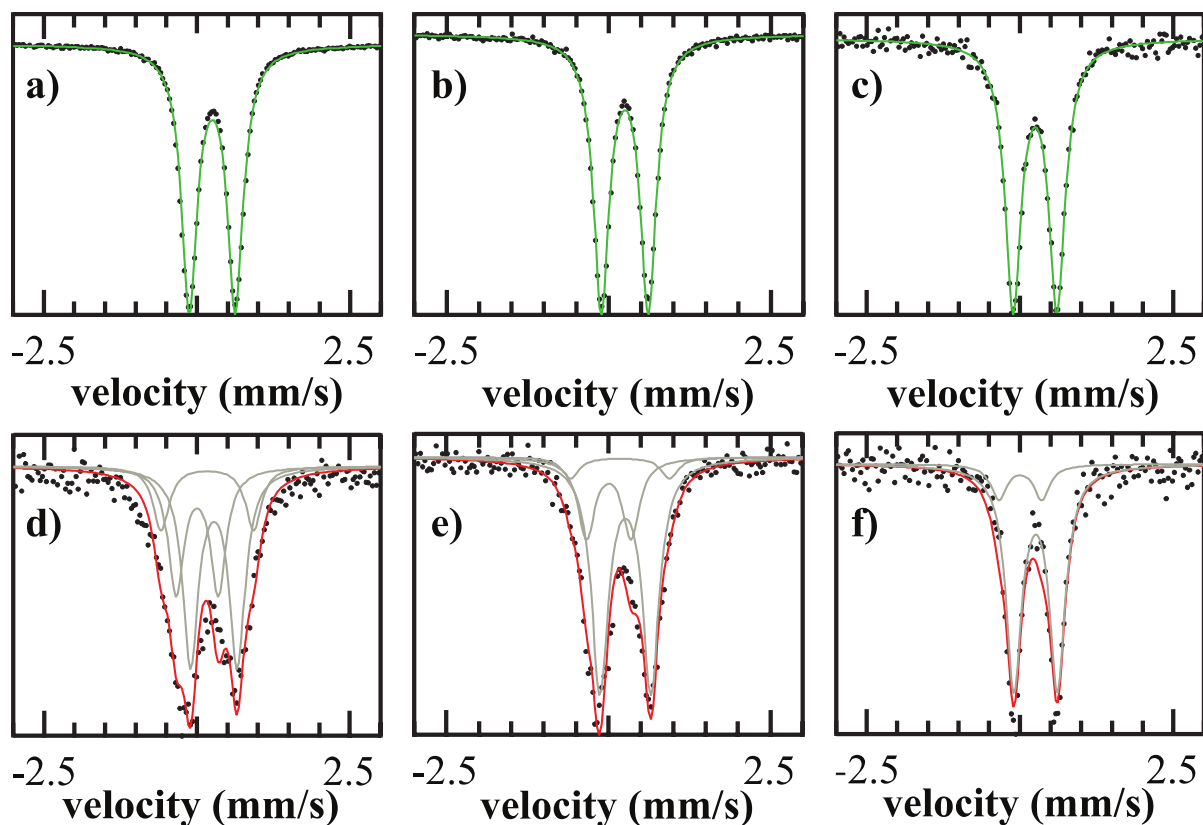
Figure 10: ^{57}\text{Fe} Mössbauer spectra of \text{Na}_x[\text{Mn}_{0.5+y}\text{Ni}_y\text{Fe}_{0.5-2y}]\text{O}_2 pristine (a-c) and charged to 4.3V (d-f) for y = 0 (a,d), y = 0.1 (b,e), and y = 0.15 (c,f). Raw data is shown in black. Individual spectral components of \text{Fe}^{3+}\text{O}_6 , \text{Fe}^{3+}\text{O}_4 and \text{Fe}^{4+}\text{O}_6 from fitting are shown in grey and the sum of all spectral components results in the colored curves.
