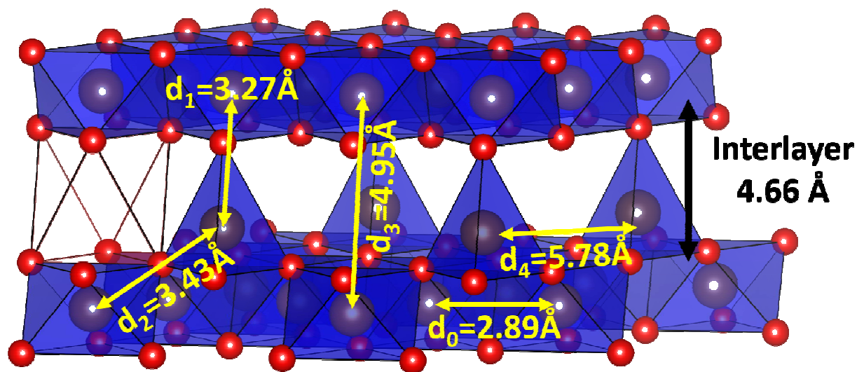
Figure 8: Representation of the bilayer used to fit the PDF curve of Na 0.14 Fe 0.5 Mn 0.5 O 2 . Transition metal atoms from the lower layer shift along the c direction (see yellow arrows) to form interlayer MO 4 tetrahedra. A vacant octahedral site is represented in red for clarity.
