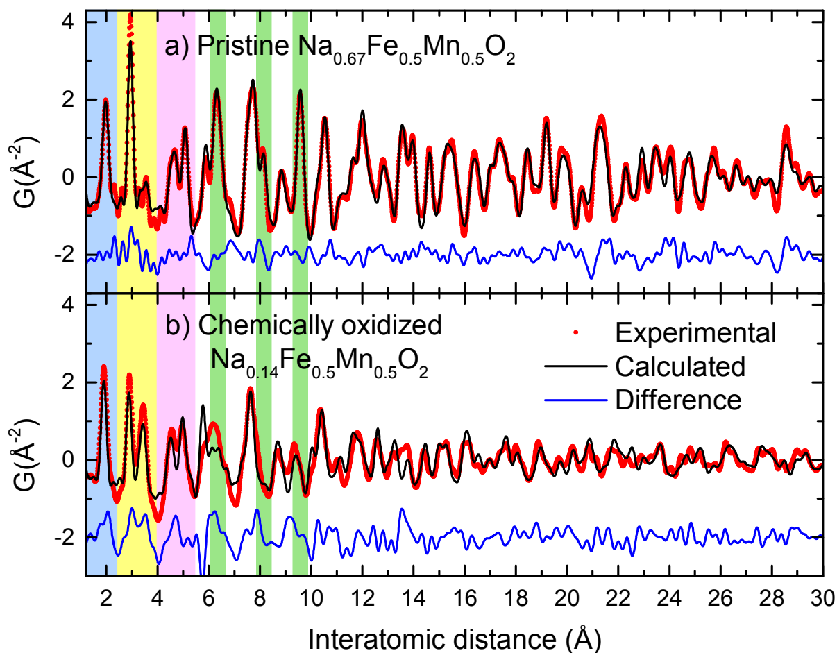
Figure 7: Fit of the PDF of a) P2- \text{Na}_{0.67}\text{Fe}_{0.5}\text{Mn}_{0.5}\text{O}_2 and b) \text{Na}_{0.14}\text{Fe}_{0.5}\text{Mn}_{0.5}\text{O}_2 . First neighbor M-O and M-M distances are highlighted in blue and yellow respectively; second neighbor in-plane M-O and M-M distances are highlighted in lavender, and characteristic interlayer M-M distances are highlighted in green (see text for details).
