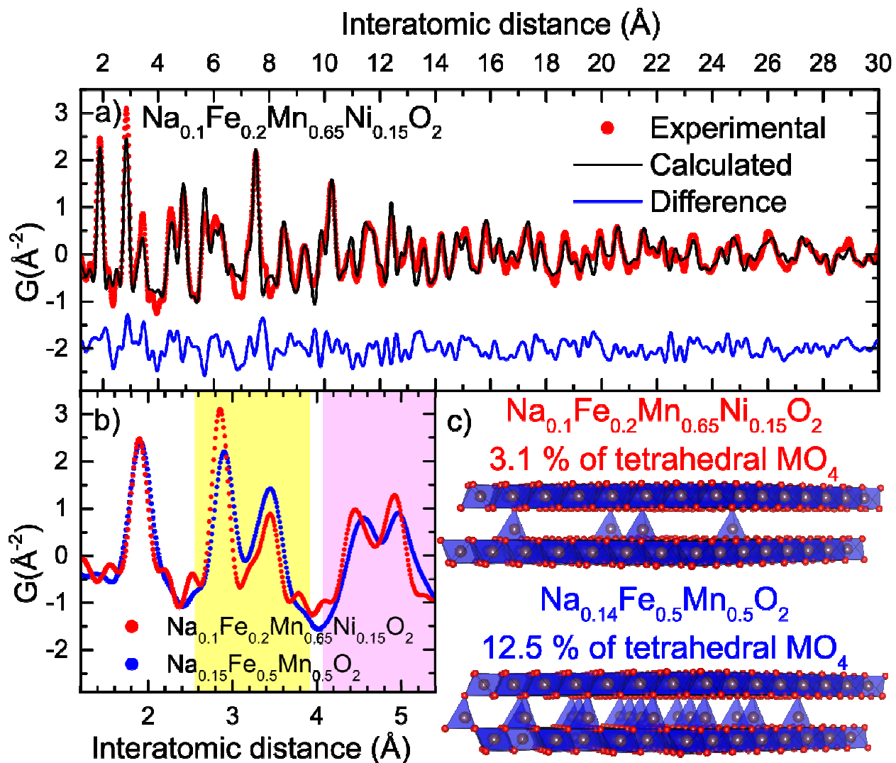
Figure 9: a) Fit of the PDF curves of chemically oxidized Z-Na 0.1 Fe 0.2 Mn 0.65 Ni 0.15 O 2 using a 4x4x10 supercell, b) comparison of the short range experimental PDF of Z-Na 0.1 Fe 0.2 Mn 0.65 Ni 0.15 O 2 and Z-Na 0.14 Fe 0.5 Mn 0.5 O 2 , showing the evolution in the MO 6 /MO 4 ratio (yellow shading) and the contraction of the bilayer thickness (lavender shading); c) representation of the two structures.
