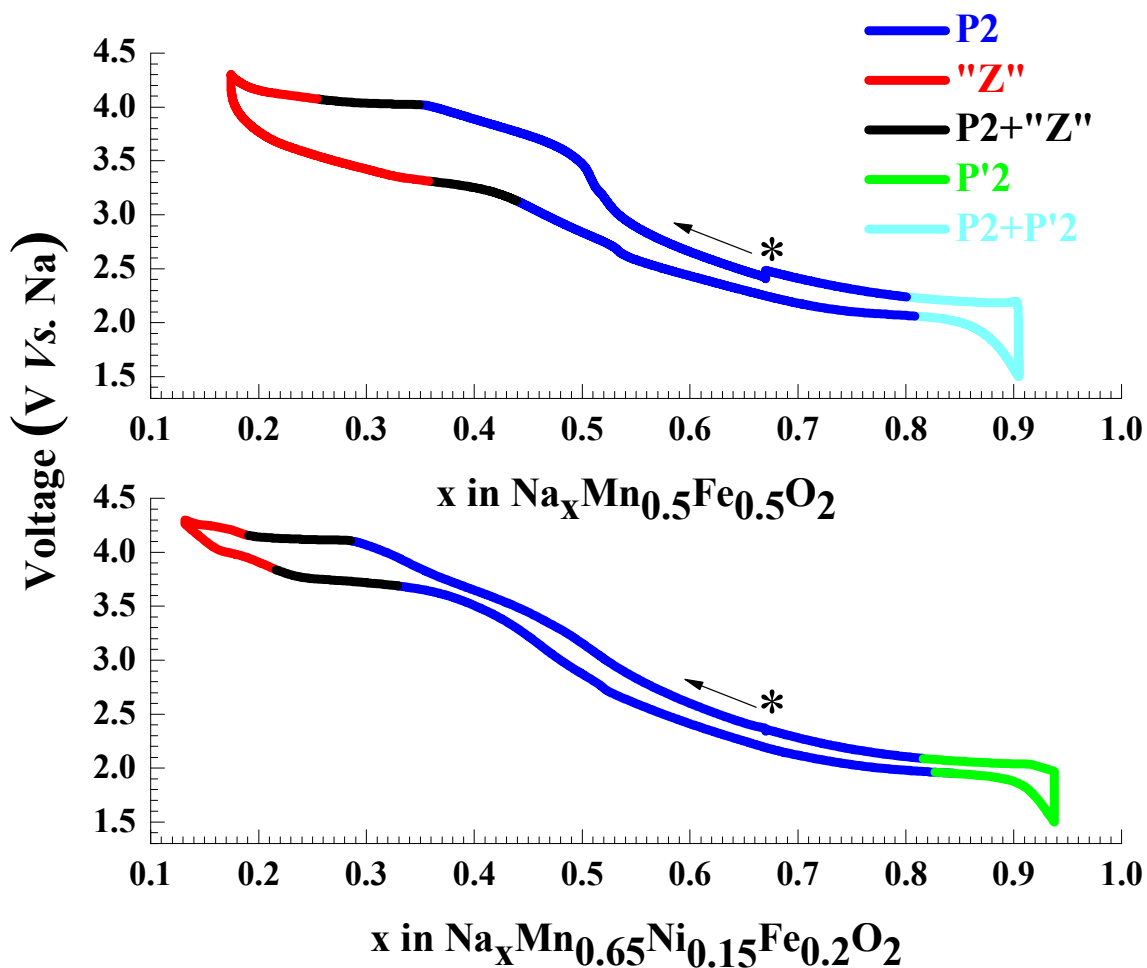
Figure 5: Phase evolution within: a) \text{Na}_{0.67}[\text{Mn}_{0.5}\text{Fe}_{0.5}]\text{O}_2 and b) \text{Na}_{0.67}[\text{Mn}_{0.65}\text{Ni}_{0.15}\text{Fe}_{0.2}]\text{O}_2 as a function of the sodium content during first cycle. The sign * shows the starting point of cycling.
