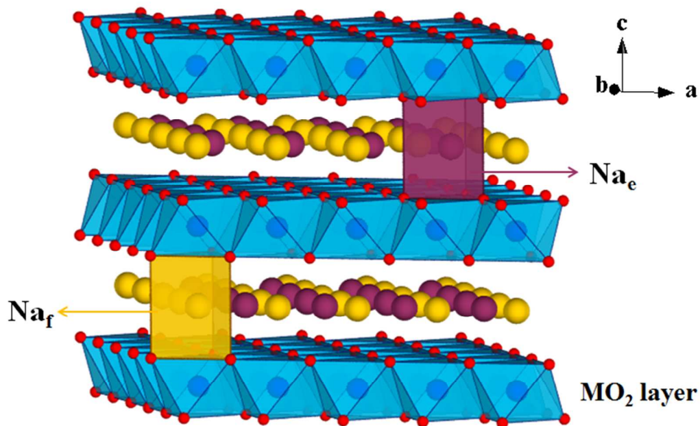
Figure 2. Schematic presentation of the P2-Na x MO 2 (M = Ni, Fe, Mn) crystal structure
