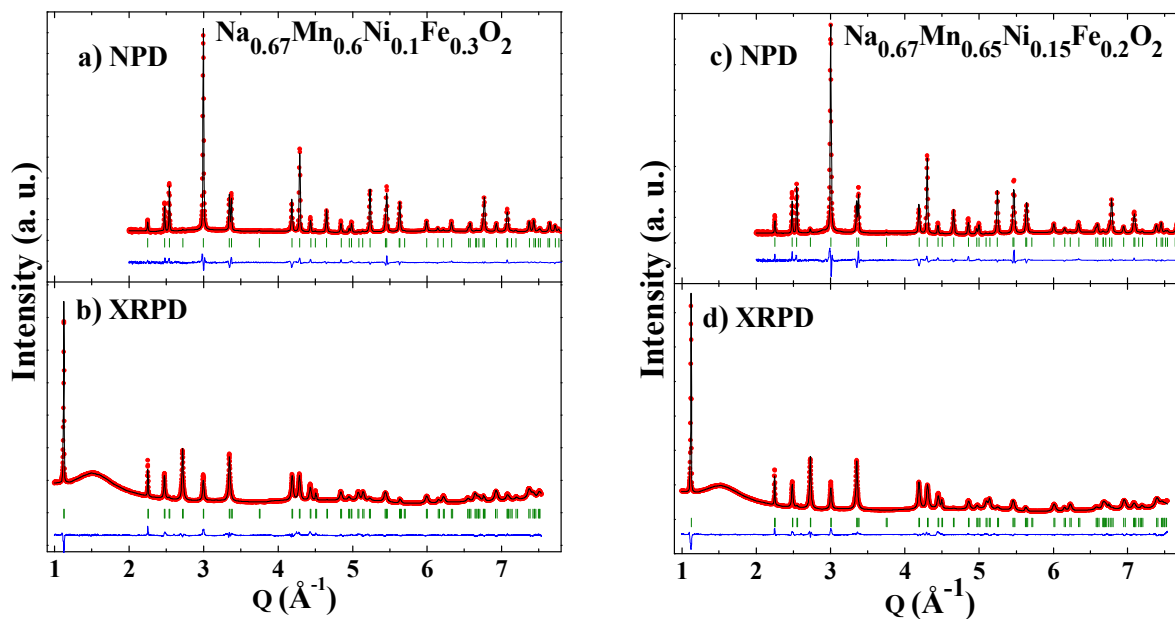
Figure 1: Combined Rietveld refinement of a) neutron and b) X-ray powder diffraction data of \text{Na}_{0.67}[\text{Mn}_{0.6}\text{Ni}_{0.1}\text{Fe}_{0.3}]\text{O}_2 and \text{Na}_{0.67}[\text{Mn}_{0.65}\text{Ni}_{0.15}\text{Fe}_{0.2}]\text{O}_2 . For each pattern, the measured data is shown by red symbols, the calculated pattern is shown in black, the difference curve is shown in blue and the Bragg peak position are marked by green ticks.
