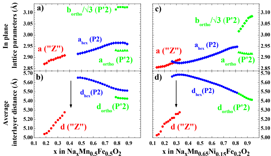
Figure 6: Evolution of lattice parameters, in-plane a), c) and out of plane b), d) of Na 0.67 Fe 0.5 Mn 0.5 O 2 a), b); and Na 0.67 [Mn 0.65 Ni 0.15 Fe 0.2 ]O 2 c), d) as a function of the sodium content during the first discharge.
