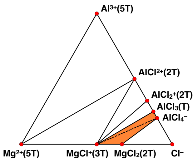
Fig. 8 Liquid Al-Cl-Mg-THF grand-potential phase diagram at the THF chemical potential. Red dots connected by black lines indicate the stable magnesium- and aluminum-chloride complexes. Coordinating THF molecules are indicated by T. Orange area and dashed line indicate the exchange reaction (c) (see Table 2 and text for more details). Tie-lines do not necessarily respect charge neutrality (see text and Supplementary Information).
