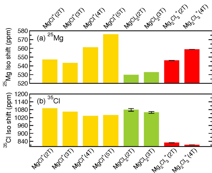
Fig. 9 a) ^{25}\text{Mg} and b) ^{35}\text{Cl} NMR isotropic shifts (in ppm) of relevant species magnesium-chloride complex ions in the MACC electrolytes. Colors for different magnesium-chloride complexes. Coordinating THF molecules indicated by T. Note that NMR data are not shifted to ^{25}\text{Mg} or ^{35}\text{Cl} standard reference compounds. Range of isotropic shifts for compounds with more than one Mg or Cl atoms is indicated by error bars.
