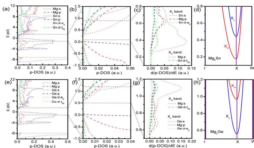
Fig. 5. Projected density of states (DOS) for \text{Mg}_2\text{Sn} (a-d) and \text{Mg}_2\text{Ge} (e-h). (a, b, e, and f) Energy versus p-DOS, (c, g) Energy versus d(p-DOS)/dE, (d, h) band structure.
