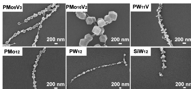
Figure 4. Effect of POM anion variation (cation: TBA) on the POM/CNT morphology. Sonication intensity =0.83 \text{ W}\cdot\text{cm}^{-2} , sonication time =4 h; sonication frequency =60 \text{ kHz} .
