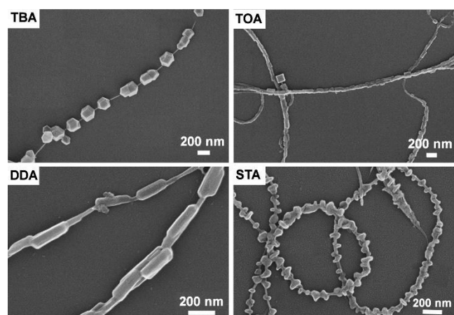
Figure 3. Effect of various cations on the deposition of \text{PMo}_{11}\text{V} on CNTs. TBA: tetra- n -butylammonium; TOA: tetra- n -octylammonium; DDA: dodecyltrimethyl-ammonium; STA: stearyltrimonium. Sonication intensity =0.83 \text{ W}\cdot\text{cm}^{-2} , sonication time =4 h; sonication frequency =60 \text{ kHz} .
