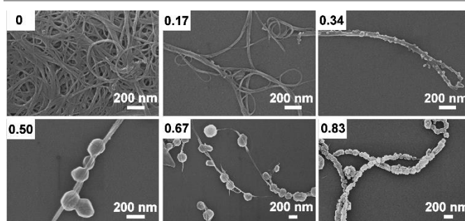
Figure 1. POM/CNT nanocomposites formation: variation of ultrasonic power intensity (inset numbers, unit: W cm -2 ) gives control over the POM-crystal size and morphology. Sonication time = 4h, sonication frequency = 60 kHz.
