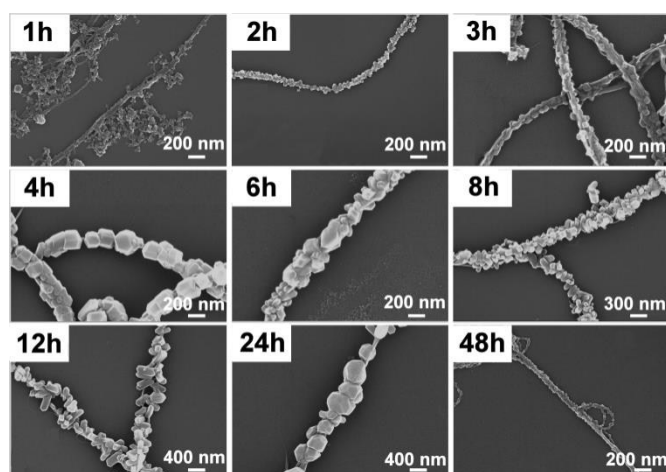
Figure 2. The influence of sonication time on the crystallization of TBA-PMo 11 V on CNTs. Sonication intensity = 0.83 W·cm -2 , sonication frequency = 60 kHz
