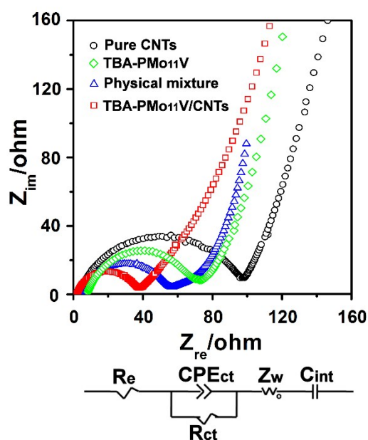
Figure 7. Nyquist plots of TBA-PMo 11 V/CNTs, the physical mixture of TBA-PMo 11 V and CNTs, TBA-PMo 11 V and pure CNTs after the first discharge–charge process at an OCV of 2.1 V. Bottom: The simulated equivalent circuit of the electrode/electrolyte interface for different electrode materials.
