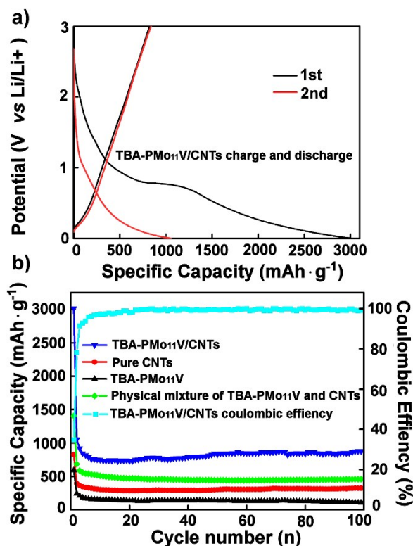
Figure 5. a) The first and second charging and discharging cycle of the LIB prototype based on the TBA-PMo 11 V/CNTs composite; b) the discharge capacity of the nanocomposite (blue), pure CNTs (red), pure POM (black) and the physical mixture (non-wired) of POM and CNTs (green) as well as the coulombic efficiency of the nanocomposite (light blue), current density is 0.5 mA·cm -2 .
