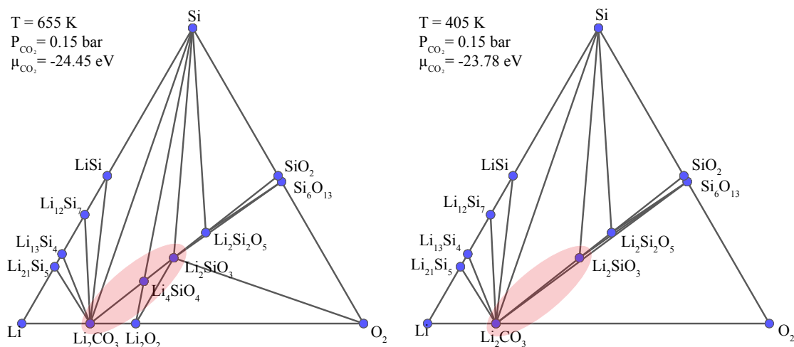
Figure 1: Ternary Li-Si-O phase diagrams under different \mu_{\text{CO}_2} obtained by applying the \text{CO}_2 grand potential to the Materials Project database. The physical equivalent of increasing the chemical potential is either an isothermal reaction performed with increasing p_{\text{CO}_2} , or an isobaric reaction under decreasing temperature. Vertices that are present in the lefthand phase diagram but are not present in righthand phase diagram represent phases which have decomposed as a result of the change in \mu_{\text{CO}_2} . The product phases of this decomposition reaction with \text{CO}_2 are situated at the vertices at either end of the edge where the original phase was formerly located. For example, \text{Li}_4\text{SiO}_4 transforms to a mixture of \text{Li}_2\text{CO}_3 and \text{Li}_2\text{SiO}_3 with increasing \mu_{\text{CO}_2} (see pink shaded area of the phase diagram).
