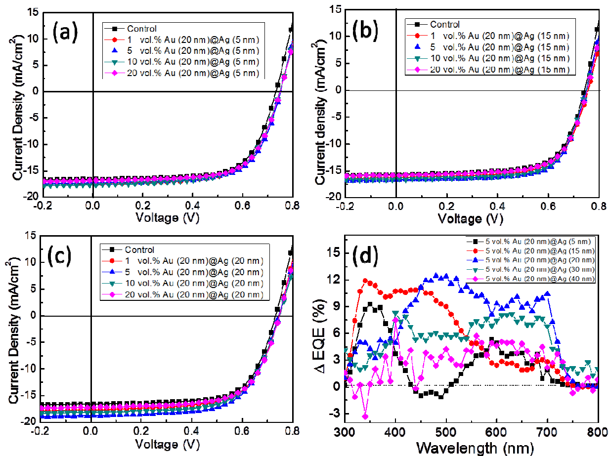
Figure 2. Current density-voltage (J-V) curves of the best control device and the OPVs with various addition levels (1, 5, 10, 20 vol%) of (a) Au(20nm)@Ag(5nm), (b) Au(20nm)@Ag(15nm), (c) Au(20nm)@Ag(20nm) NCs. (d) EQE enhancement ( \Delta EQE) of the OPVs with the addition level of 5 vol% of Au@Ag NCs with different Ag shell thicknesses.
