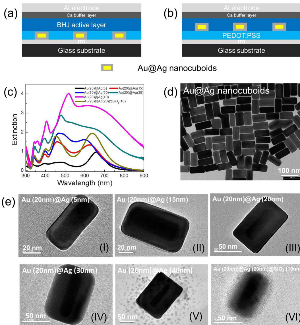
Figure 1. Scheme of OPVs with the incorporation of Au@Ag NCs in (a) PEDOT:PSS layer and (b) bulk heterojunction (BHJ) active layer. (c) Extinction spectra of Au@Ag NCs in aqueous solutions and Au@Ag@SiO 2 NCs in an ethanol solution. All samples have the same concentration of NCs in the solutions. The Au(20nm)@Ag(5nm), Au(20nm)@Ag(15nm), Au(20nm)@Ag(20nm), Au(20nm)@Ag(30nm) and Au(20nm)@Ag(40nm) NCs have the same diameter of Au rod (20nm) and different Ag shell thicknesses of 5, 15, 20, 30 and 40nm, respectively. (d) TEM images of Au(20nm)@Ag(20nm) NCs. (e) TEM images of individual Au@Ag NCs with different Ag shell thicknesses in (I-V) and an individual Au@Ag@SiO 2 NC in (VI).
