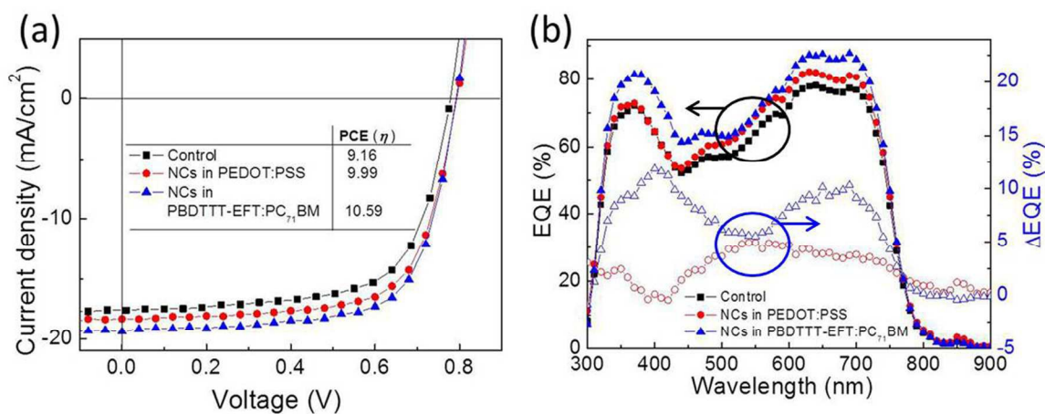
Figure 4. (a) J–V, (b) EQE (solid symbols) and EQE enhancement ( \Delta EQE) (open symbols) curves of PBDTTT-EFT:PC 71 BM -based OPVs with the Au@Ag@SiO 2 NCs embedded in PEDOT:PSS or PBDTTT-EFT:PC 71 BM layers.
