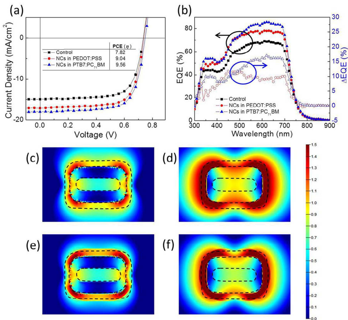
Figure 3. (a) J–V, (b) EQE (solid symbols) and EQE enhancement ( \Delta EQE) (open symbols) curves of PTB7:PC 71 BM-based OPVs with Au@Ag@SiO 2 NCs in the PEDOT:PSS layer or the active layer. (c–d) Simulated enhancement distribution of electric field intensity for Au@Ag@SiO 2 NCs in PEDOT:PSS with (c) the transverse dipole mode and (d) the longitudinal dipole mode at the resonance wavelengths of 492 nm and 621 nm, respectively. (e–f) Simulated electric field enhancement for Au@Ag@SiO 2 NCs in PTB7:PC 71 BM with (e) the transverse dipole mode and (f) longitudinal dipole mode at the resonance wavelengths of 513 nm and 691 nm, respectively. The dash lines show the boundaries between two different media. The enhancements of the electric field intensity are presented at the logarithmic scale.
