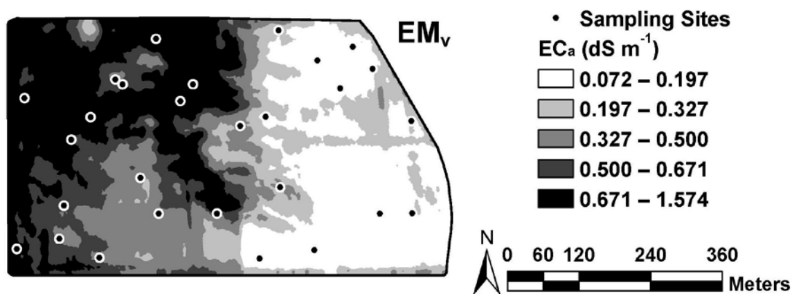
Figure 1. Maps showing the apparent soil electrical conductivity ( EC_a ) survey taken with electromagnetic induction in the vertical ( EM_v ) coil configuration for a 32-ha study site on Scott Brothers' Dairy Farm in San Jacinto, CA. The locations of 28 EC_a -directed soil sampling sites, which were selected using a stratified random sampling design, are identified by solid circles.
