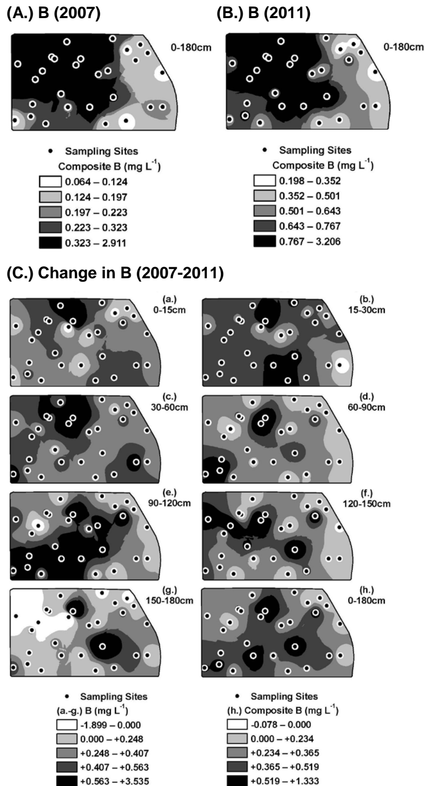
Figure 5. Field-scale distribution of B (saturation extract) at 0-1.8 m for the years (A.) 2007 and (B.) 2011, and (C.) change in B from 2007 to 2011 at depth increments of (a.) 0-15, (b.) 15-30, (c.) 30-60, (d.) 60-90, (e.) 90-120, (f.) 120-150, (g.) 150-180 cm and composite depth of (h.) 0-180 cm.
