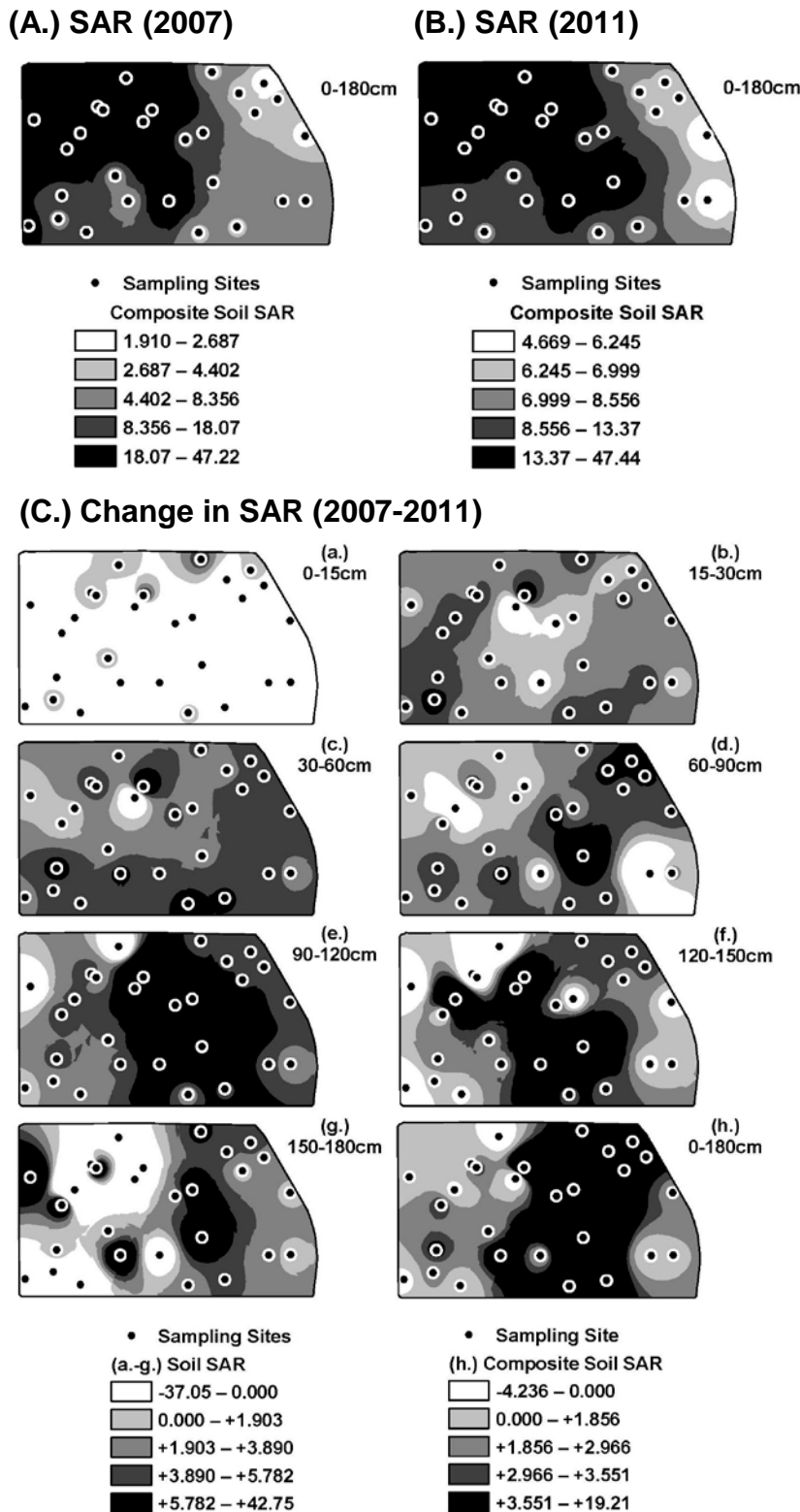
Figure 3. Field-scale distribution of SAR (sodium adsorption ratio) at 0-1.8 m for the years (A.) 2007 and (B.) 2011, and (C.) change in SAR from 2007 to 2011 at depth increments of (a.) 0-15, (b.) 15-30, (c.) 30-60, (d.) 60-90, (e.) 90-120, (f.) 120-150, (g.) 150-180 cm and composite depth of (h.) 0-180 cm.
