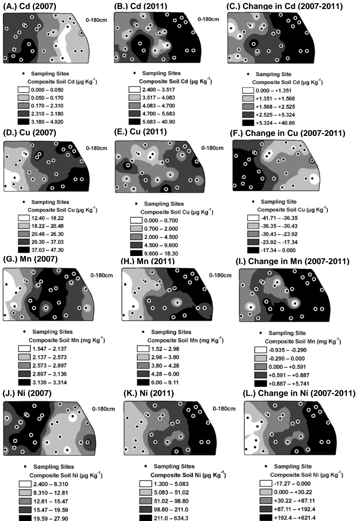
Figure 6(A-L). Distribution of metals (double acid extract) at 0-1.8 m for the years 2007, 2011, and change from 2007 to 2011: (A-C.) Cd, (D-F.) Cu, (G-I.) Mn, (J-L.) Ni, and (M-O.) Zn.
