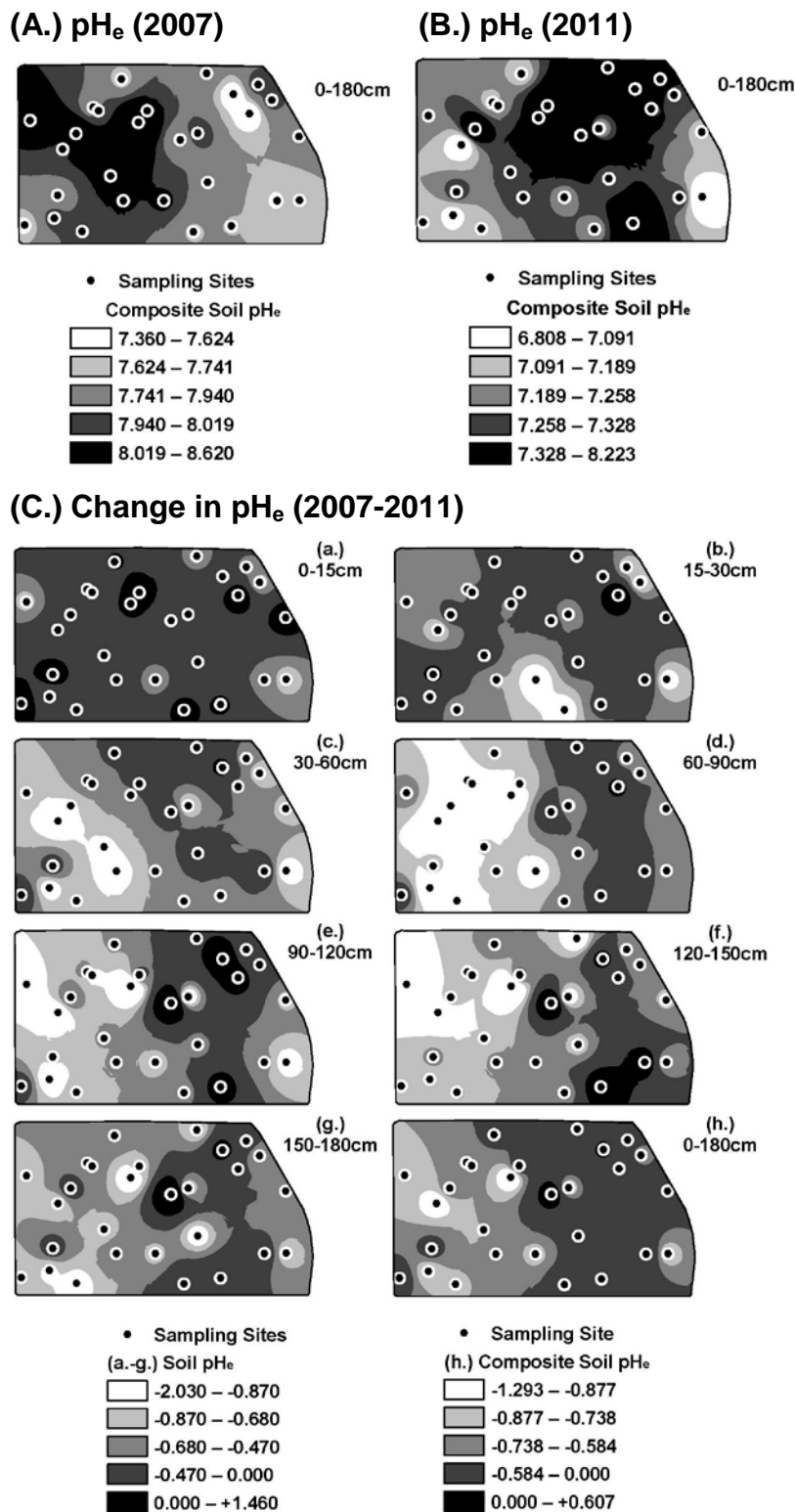
Figure 4. Field-scale distribution of pH_e (saturation extract) at 0-1.8 m for the years (A.) 2007 and (B.) 2011, and (C.) change in pH_e from 2007 to 2011 at depth increments of (a.) 0-15, (b.) 15-30, (c.) 30-60, (d.) 60-90, (e.) 90-120, (f.) 120-150, (g.) 150-180 cm and composite depth of (h.) 0-180 cm.
