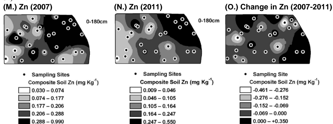
Figure 6(M-O; continued). Distribution of metals (double acid extract) at 0-1.8 m for the years 2007, 2011, and change from 2007 to 2011: (A-C.) Cd, (D-F.) Cu, (G-I.) Mn, (J-L.) Ni, and (M-O.) Zn.
