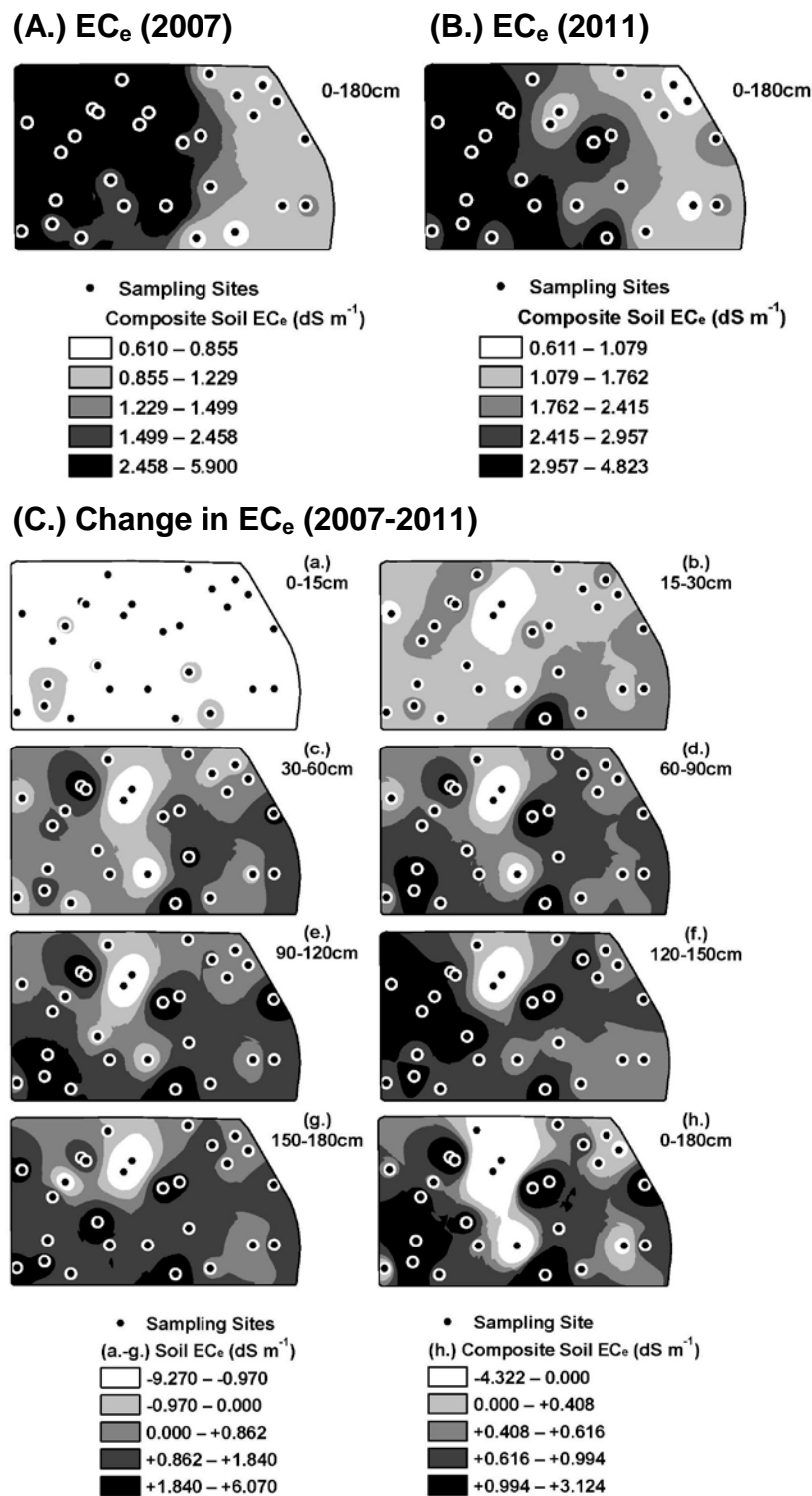
Figure 2. Field-scale distribution of salinity (i.e., EC_e , electrical conductivity of the saturation extract) at 0-1.8 m for the years (A.) 2007 and (B.) 2011, and (C.) change in salinity from 2007 to 2011 at depth increments of (a.) 0-15, (b.) 15-30, (c.) 30-60, (d.) 60-90, (e.) 90-120, (f.) 120-150, (g.) 150-180 cm and composite depth of (h.) 0-180 cm.
