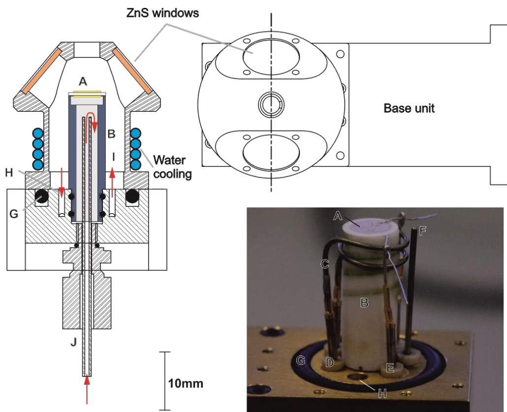
Figure 2 Detailed cross section of base and dome and a photograph of apparatus showing electrochemical cell (A), crucible (B) heating element (C), gold crimp connections for the heating wire (D) and the electrical cell connections (E), K-type thermocouple (F), dome Viton O-ring seal (G) cell, gas feed-throughs (H and I) and underside inlet port (J) (see text for more detail).
