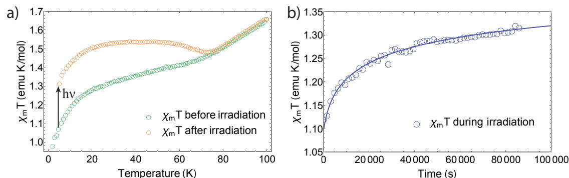
Fig. 4 a) Change of \chi_m T for a powder sample of 1 at an external field of 5000 Oe. After irradiation for 24 h at 5.4 mW, \chi_m T increases for about 20% at 5 K.; b) \chi_m T against time during irradiation and exponential fit ( \beta = 0.33 and \tau = 26700 s). Due to thermal fluctuations of 0.5 K, nonlinear temperature behavior of the susceptibility and very long relaxation time, the fit quality is questionable.
