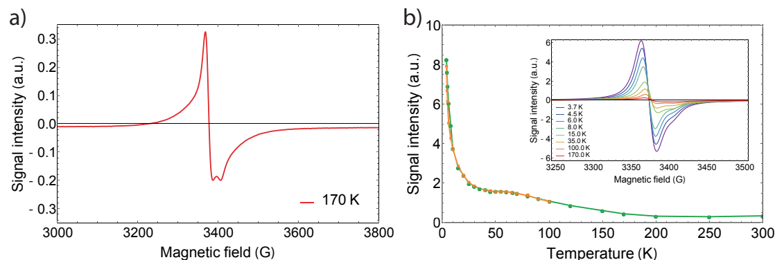
Fig. 3 a) Derivative EPR signal for 1 at 170 K.; b) Extracted signal intensities versus temperature at fixed microwave power. No thermal hysteresis has been observed between cooling (green) and warming (orange). Inset: X-Band spectrum at different temperatures.
