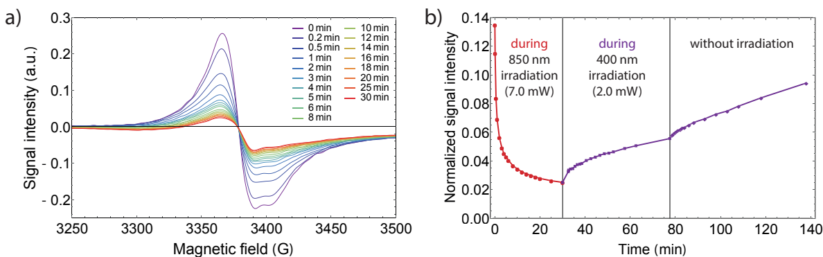
Fig. 7 a) EPR Signal intensity while irradiating with 850 nm light and 7 mW light power, after first irradiating for 70 min at 532 nm and 1.5 mW.; b) Wavelength dependent performance of the photoabsorption process at 3.75 K. After first irradiation at 532 nm, the normalized signal was reduced from 1.0 to 0.14, whereby the signal change is comparable to Fig. SI6. In contrast to some other Co VT compounds that show back switching behavior, the excitation is enhanced. The signal decreases even further down close to 0.02, which corresponds to a net excitation of 98%. By changing the wavelength to 400 nm at 1.5 mW, the signal increases again. As the signal increases faster after turning off the light source, the increase during irradiation at 400 nm is due to the fact that the relaxation goes faster than the excitation at this wavelength.
