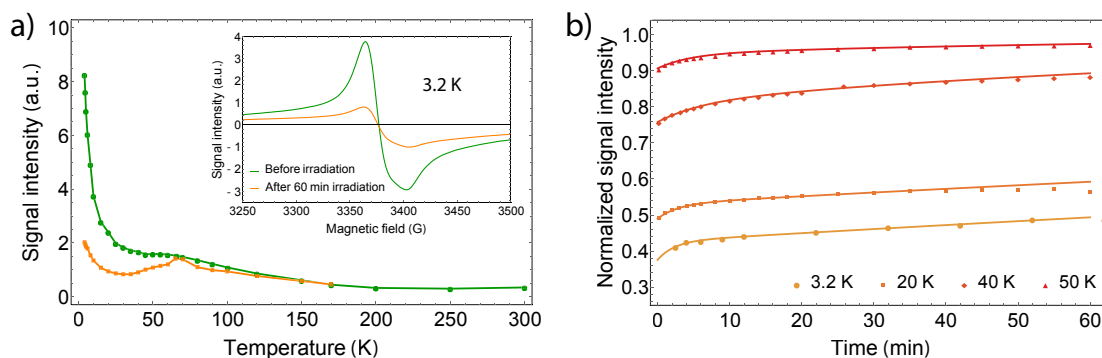
Fig. 5 a) EPR signal intensity of the derivative signal of spin-1/2 species while cooling down before (green) irradiation and by warming up after (orange). The inset displays the signal change after 60 min of irradiation (orange); b) Time dependence of the signal relaxation after 60 min irradiation of 532 nm light. The data has been fitted using two exponential functions, which account for relaxation and thermal assimilation.;
