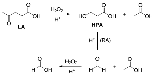
Scheme 2. Oxidation of LA to acetic and formic acids with \text{H}_2\text{O}_2 . RA = retro aldol.
