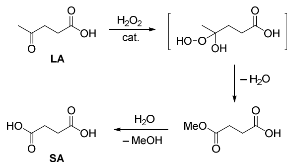
Scheme 1. Oxidation of LA to SA with H 2 O 2 .
