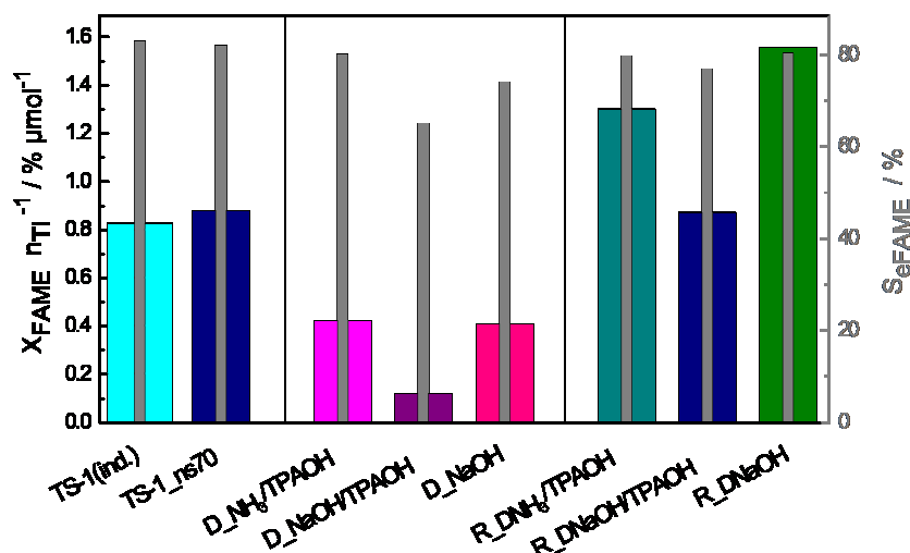
Fig. 13 Catalyst efficiency (conversion related to the amount of Ti atoms in the catalysts) for the epoxidation of biodiesel (FAME) with \text{H}_2\text{O}_2 over micro-/mesoporous TS-1 as well as epoxide selectivity ( S_{eFAME} ) after 5 h of reaction ( V_{\text{acetonitrile}} = 10 \text{ cm}^3 , C_{FAME} = 0.03 \text{ mol L}^{-1} , (n_{\text{H}_2\text{O}_2}/n_{FAME}) = 5 \text{ mol mol}^{-1} , m_{\text{cat}} = 150 \text{ mg} , T = 323 \text{ K} ).
