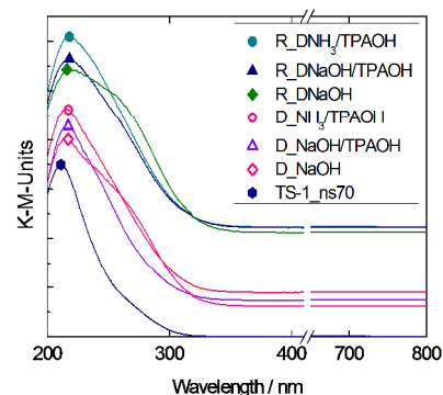
Fig. 7 DRUV-visible spectra (in Kubelka–Munk units) of the parent TS-1 ns70 , desilicated (D-series) and recrystallized TS-1 (R_D-series).
