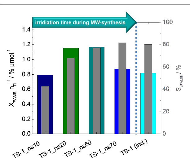
Fig. 11 Catalyst efficiency (conversion related to the amount of Ti atoms in the catalysts) for the epoxidation of biodiesel (FAME) with H_2O_2 over as well as epoxide selectivity ( S_{eFAME} ) over nano-sized TS-1 and conventional TS-1(ind.) after 5 h of reaction ( V_{acetonitrile} = 10 \text{ cm}^3 , c_{FAME} = 0.03 \text{ mol L}^{-1} , (n_{H_2O_2}/n_{FAME}) = 5 \text{ mol mol}^{-1} , m_{cat.} = 150 \text{ mg} , T = 323 \text{ K} ).
