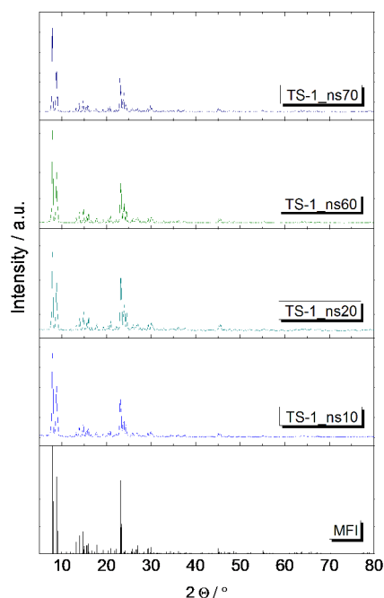
Fig. 1 Powder X-ray diffraction patterns of the TS-1_ns obtained after different irradiation times during microwave-assisted synthesis. The MFI-diffraction is adapted from 40 .
