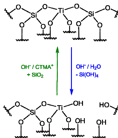
Fig. 12 Generation of defect sites (surface hydroxyl groups) in TS-1 by desilication (blue), "healing" of the defects by re-arrangement in the presence of \text{CTMA}^+ (green).
