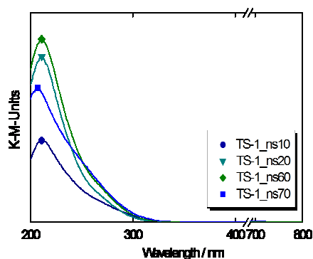
Fig. 3 DR-UV-Vis spectra (in Kubelka–Munk (K-M)-units) of nano-sized TS-1_ns obtained after different irradiation times during microwave-assisted synthesis.
