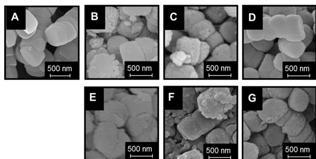
Fig. 6 SEM images of the parent TS-1 ns70 (A), desilicated (D-series) TS-1: D NH 3 /TPAOH (B), D NaOH /TPAOH (C), D NaOH (D) (upper part) and recrystallized TS-1 (R_D-series): R DNH 3 /TPAOH (E), R DNaOH /TPAOH (F), R DNaOH (G) (lower part).
