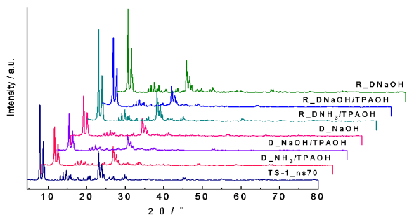
Fig. 5 Powder X-ray diffraction patterns of the parent TS-1 ns70 , desilicated (D-series) and recrystallized TS-1 (R_D-series).
