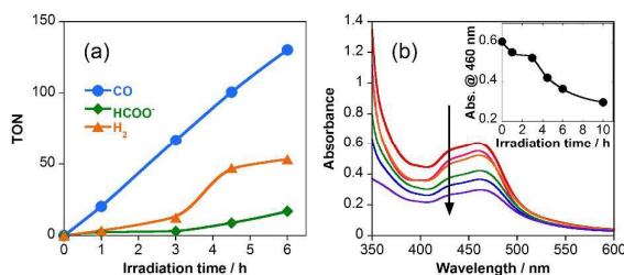
Fig. 1 (a) Time-dependent production of CO (blue), HCOO − (green), and H 2 (orange) in the photocatalytic reaction using RuRe . A 4 mL of NaOH (0.1 M) aqueous solution containing RuRe (0.05 mM) and BI(CO 2 − )H (10 mM) was irradiated at \lambda_{\text{ex}} > 500 nm under a CO 2 atmosphere. (b) UV–vis absorption changes during the photocatalytic reaction. The inset shows time-dependent absorbance changes at 460 nm.
