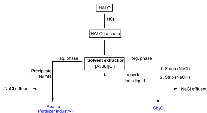
Figure 9. Schematic overview of the proposed recycling process. After full dissolution in diluted HCl, the antimony is selective extracted from the leachate using the ionic liquid Aliquat® 336 and pure Sb 2 O 3 is obtained after scrubbing and stripping. The remaining elements in the leachate are then reprecipitated as an apatite which can serve as feedstock in the fertilizer industry. The only waste of this process is an aqueous NaCl effluent which can be discarded in the sea.
