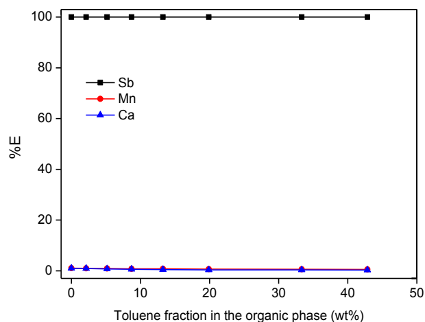
Figure 5. Influence of toluene in the IL phase on the extraction of Sb(III), Mn(II) and Ca(II) ions. The extraction was done from a HALO leachate, prepared by dissolving 25 g/L of HALO in 1 M HCl. A 2:1 phase ratio (wt:wt) was used for the aqueous phase and the IL phase [A336][Cl].
