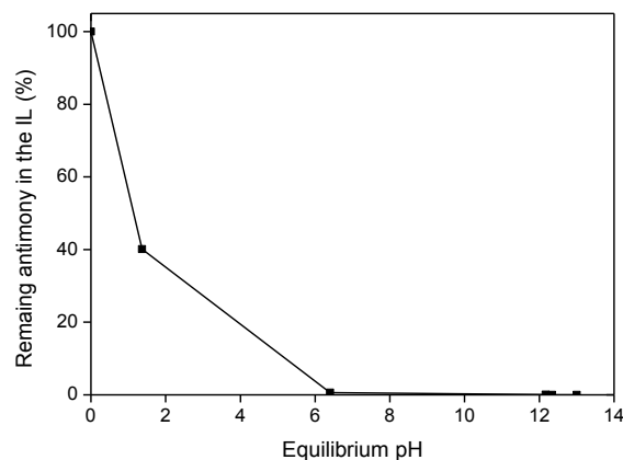
Figure 6. Stripping of Sb(III) ions from the ionic liquid phase as function of the equilibrium pH, using a water phase with increasing amounts of NaOH.
