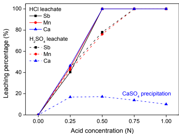
Figure 2. Dissolution of HALO (25 mg/g) in increasingly concentrated HCl and H 2 SO 4 solutions. The samples were shaken (2000 rpm) for 1 h at 25 °C.
