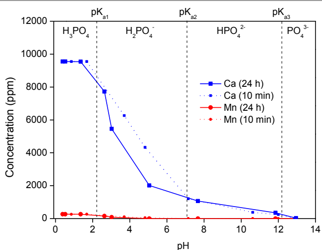
Figure 7. The remaining metal concentration in solution is shown to evaluate the precipitation of the apatite residue as function of pH. The initial pH of the leachate after extraction was 0.37 and the pH was increased by using NaOH.
