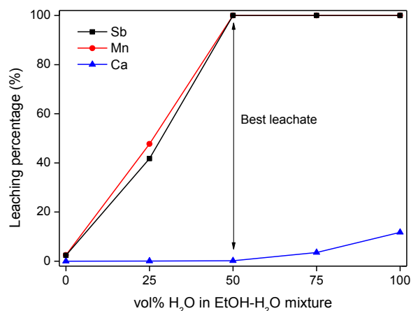
Figure 3. Influence of the EtOH–H 2 O ratio on the dissolution of HALO with 1 N H 2 SO 4 . The samples were shaken (2000 rpm) for 1 h at 25 °C.
