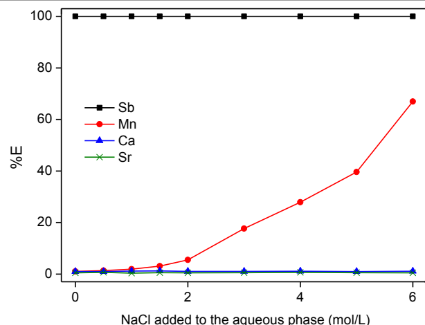
Figure 4. Percentage extraction (%E) of Sb(III), Mn(II), Ca(II) and Sr(II) ions as function of the addition of NaCl to the HALO leachate (the aqueous phase). The HALO leachate was prepared by dissolving 25 g/L of HALO in 1 M HCl. A 2:1 phase ratio (wt:wt) was used for the aqueous phase and the IL phase [A336][Cl].
