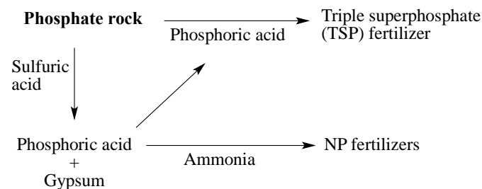
Figure 1. Main industrial production routes for phosphate fertilizers.
