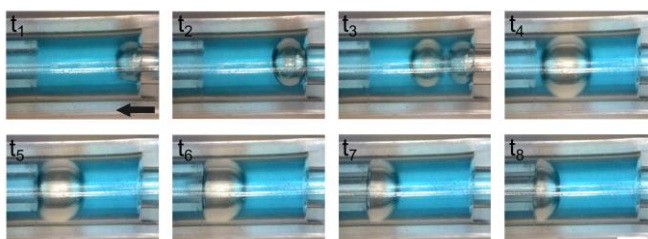
Figure 3 Experimental air bubble trapping. Snapshots of the bubble trapping with water as fluid at a flow rate of 110 \mu\text{L}/\text{min} . The black arrow indicates the flow direction. Scale bar 1mm.
