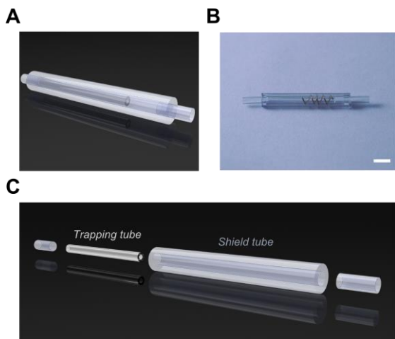
Figure 1 Schematic view of the air bubble trap. A 3D rendering and B a photograph of the assembled trap. C shows the rendered trap in explosion view with all components: connection tube, trapping tube, shield tube and second connection tube (from left to right). Scale bar 5mm.
