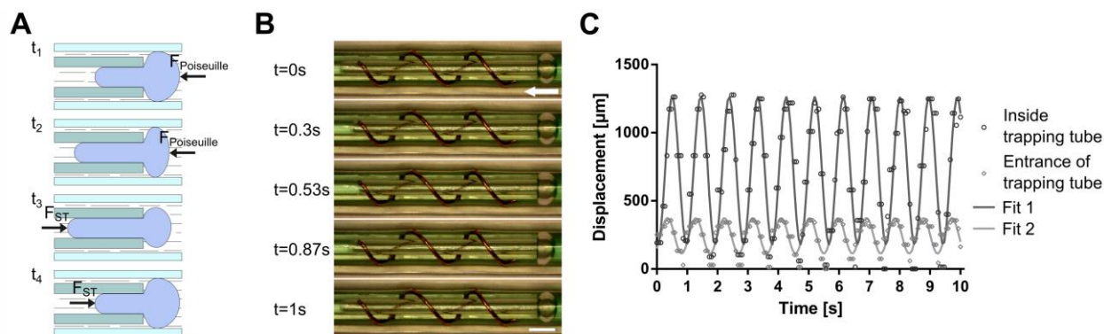
Figure 4 Bubble oscillation. A schematic of the bubble oscillation after trapping. The oscillation of the bubble (blue) is due to the combined and opposite forces induced by the hydrodynamic ( F_{\text{Poiseuille}} ) and surface tension ( F_{\text{ST}} ) forces. B Oscillation of an air bubble in 100% ethanol (white arrow indicates the flow direction). Scale bar 1.5mm. C Bubble oscillation as function of time. The circles and diamonds are the data points of the bubble displacement in the trapping tube and at the entrance, respectively. The solid lines represent the two sinusoidal curve fittings (Fit 1, Fit 2).
