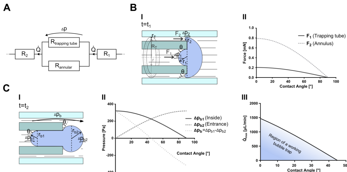
Figure 2 Principles of the trapping concept. A Schematic of the equivalent fluidic resistance circuit of the bubble trap. B I Schematic of a bubble at the entrance of the trap and the acting forces during the initial contact (cross-section). B II Corresponding forces as function of the contact angle for the dimensions given in Table 1. C I Schematic of the trapped bubble including the acting Laplace pressures (cross-section). C II The corresponding Laplace pressures as well as the maximal flow rate at which the bubble can be kept inside the bubble trap as function of the contact angle, for the given dimensions (Table 1) III .
