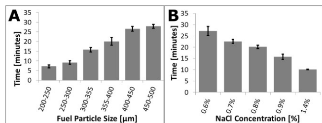
Figure 3: A: Mean time to reach 90% of the peak reaction temperature for various particle sizes of Mg-Fe fuel, n=6 minimum, error bars represent \pm one standard deviation. B: Mean time to reach 90% of the peak reaction temperature is plotted for various saline concentrations. Reaction power output was quantified by monitoring temperature change in a lab-built calorimeter, n=4 minimum, error bars represent \pm one standard deviation.
