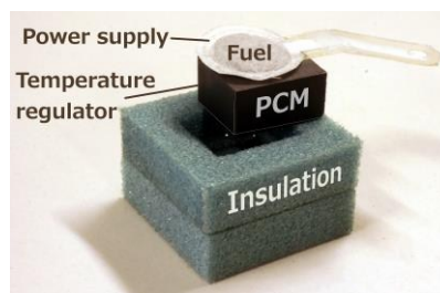
Figure 1: Precision heater designed for use with isothermal NAATs, partially disassembled view. The diagnostic assay sits beneath the PCM block within an appropriate cut-out in the insulation. Top insulation omitted for clarity. A NaCl solution is delivered to this type of power supply via a paper wick from a reservoir (not shown).
