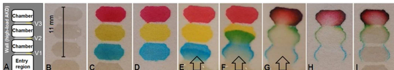
Figure 4: Paper microfluidic device based on selective permeability for multi-step chemical reactions. (A) Schematic overview of the device, which contains hydrophilic regions (white) separated by low-load AKD valves (light gray, V1-V3), the total of which is surrounded by high-load AKD walls (dark gray). (B) An actual device in which the hydrophilic regions are wetted with water. (C) The three chambers are filled with aqueous solutions of different dyes (4 \mu L) and (D) dried. (E-G) The device is dipped into 50% ethanol in water for elution of the dyes through the selectively permeable valves. Upon elution the different dyes mix and end up in the top chamber. (H) The device is dried and (I) rewetted with water to demonstrate that the valves are still intact.
