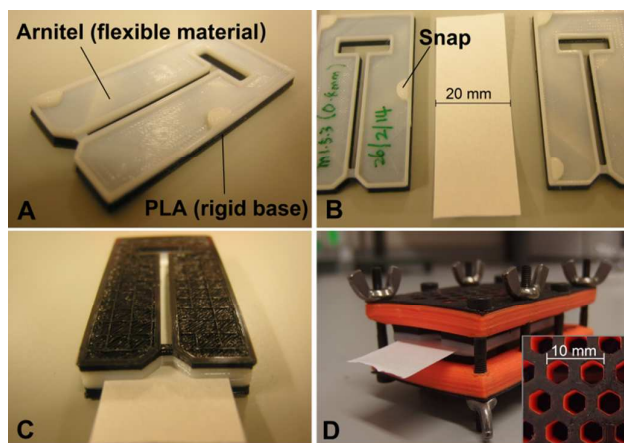
Figure 1: 3D-printed tools for the fabrication of AKD patterned paper microfluidic devices. (A) A mask part made of PLA (lower half, black) and flexible Arnitel (upper half, white). The rigid PLA base allows equal distribution of pressure over the mask, whereas the Arnitel top allows a tight seal upon the application of pressure. (B) Two mirror-image mask parts, which can be aligned with snap connections and an AKD-coated piece of chromatography paper. (C) The paper is sandwiched between the mask parts. The rigid PLA base, as well as the Arnitel top, contain ridges to focus pressure on the borders between shielded and non-shielded areas of the paper. (D) The mask and paper sandwich is put into an ABS clamp containing honeycomb cavities (inset) and pressure is applied by tightening the screws. The assembly is then exposed to oxygen plasma to re-hydrophilize the unshielded areas.
