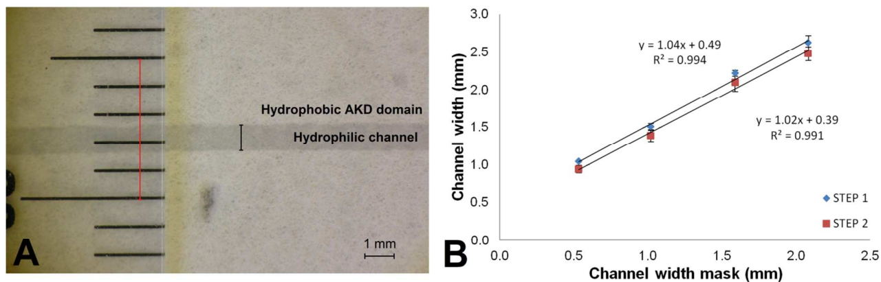
Figure 3: Characterization of both AKD application steps. (A) The channel width was measured with ImageJ from a photograph in which the channel was wetted with water and a ruler was used as size reference. The actual channel width was calculated by multiplying the ratio between the black vertical bar and the red vertical bar by 5 mm. (B) The average channel width ( n=5 devices per data point) is plotted versus the channel width of the 3D-printed mask parts for both application steps. Error bars show the standard deviation.
