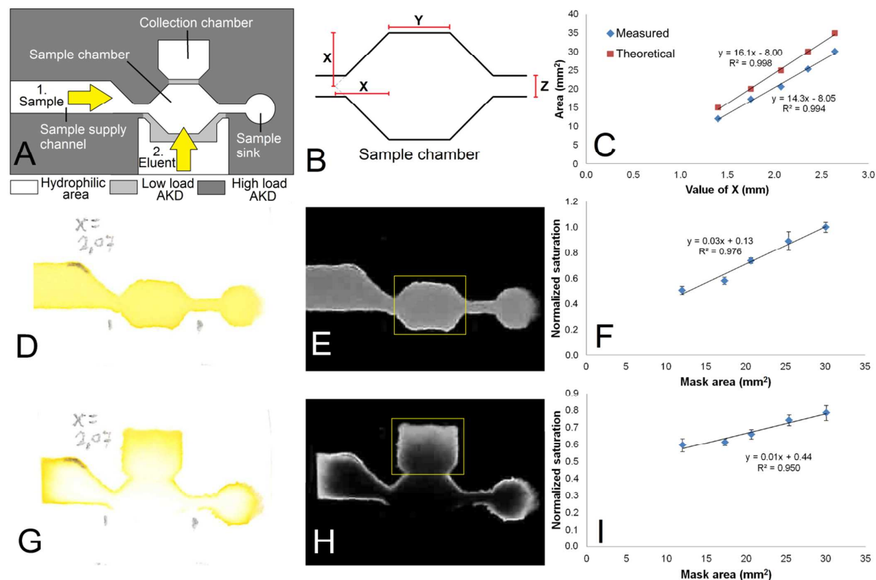
Figure 5: Volume-defined sampling with a paper microfluidic device. (A) Schematic representation of the device. White areas are hydrophilic, light gray areas have a low AKD load (valves) and dark gray areas have a high AKD load (walls). Sample can be loaded into this device via the left supply channel (labeled '1. Sample'). Sample wicks into a sample chamber and later into a sample sink, designed to prevent sampling bias. After the sample has dried, it can be eluted perpendicularly with 55% ethanol in water via the bottom entry channel (labeled '2. Eluent'). Due to the design, sample from within the sample chamber will be eluted upwards and collected in the upper collection chamber. Sample in other parts of the device will be drained via the sample supply channel or into the sample sink. (B) Schematic overview of the sample chamber. The value of X is varied in order to produce devices with different volumes for the sample chamber. The respective values for Y and Z are 4 mm and 0.5 mm. (C) Relation between the actual and theoretical areas of the sample chamber in the 3D-printed mask and the value of X. (D) Example of a device loaded with yellow dye solution. (E) The same device in HSB display (saturation) in ImageJ, which is used to quantify color in a certain region of the device. The total saturation of the area within the yellow lines was quantified. (F) The normalized saturation of the sample chamber is plotted against the area of the sample chamber in the mask ( n=3 devices per mask). Error bars show the standard deviation. (G-I) Same as D-F, but after elution and measured in the sample collection chamber. This last series represents the sample that can be used for downstream processing and/or detection.
