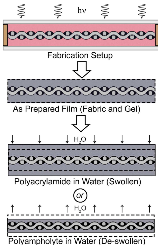
Figure 1 - Preparation of composite samples. Fabric with spacers attached is placed into a glass mold with a monomer solution (pink), and exposed to UV light. The as-prepared film is then placed into water, and swelling or de-swelling occurs, depending on hydrogel chemistry. De-swelling, which occurs with the polyampholyte composite sample, is considered an important mechanism for fabricating mechanically superior hydrogel composites.
