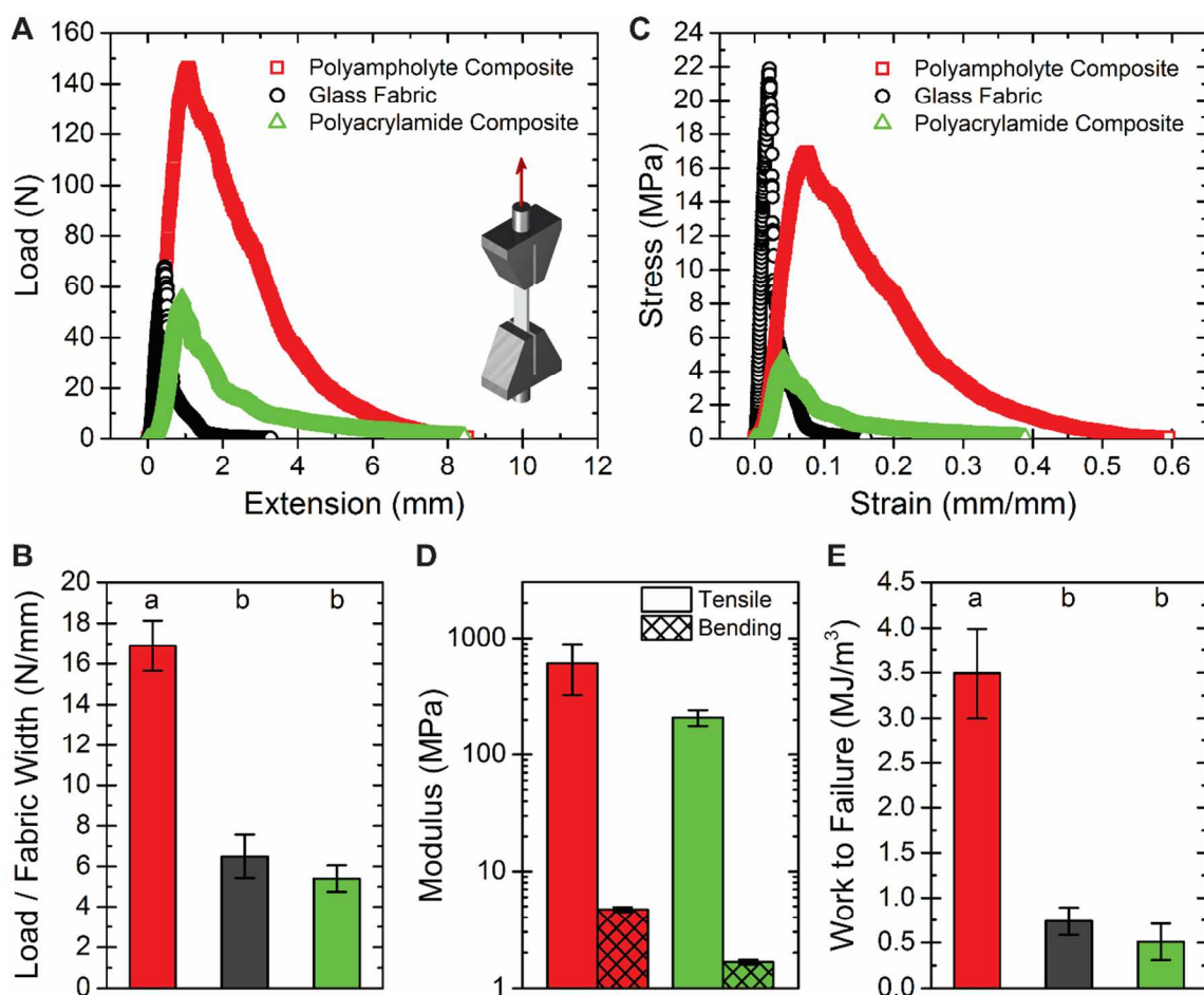
Figure 1 - (A) Representative load vs. extension curve for the three samples tested, with t = 0.31 mm w = 10.0 mm and L = 20.5 mm for the neat fabric, t = 0.94 mm, w = 9.2 mm, and L = 14.3 mm for the polyampholyte composite, and t = 1.16 mm, w = 10.0 mm, and L = 21.7 mm for the polyacrylamide composite. Testing geometry is shown as an inset. (B) Maximum load normalized by fabric width, for the three samples tested. The polyampholyte composite supports more than 2.5x the load per sample width when compared to the neat fabric or the polyacrylamide composite. (C) Stress versus strain curve for the samples presented in (A). (D) A comparison of the average tensile and bending modulus for the two composite samples. The fabricated composites exhibit highly anisotropic properties. (E) Work to failure for the three samples tested. Results agree with the tear strength results. For (B) and (E), ANOVA testing was used with a post-hoc Tukey test to determine significance, with P < 0.001 . Error bars represent standard deviation, with N > 5 .
