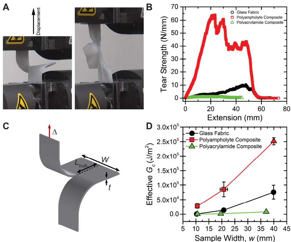
Figure 2 - (A) A polyampholyte hydrogel composite in the grips of a tensile tester before a tearing testing, and while undergoing large strain deformation in a tearing test. (B) Representative tear strength vs. displacement curves for neat fabric, polyacrylamide hydrogel composite, and polyampholyte hydrogel composite samples, with w = 20 mm. The polyampholyte composite exhibits much higher tear strength than the two control groups. (C) Schematic of the tear test specimen, with important dimensions labelled. (D) Effective G_c vs. sample width for the three test groups. As width increases tear strength increases for all samples, due to the fiber pull-out failure mechanism. Error bars represent standard deviation, with N > 4 .
