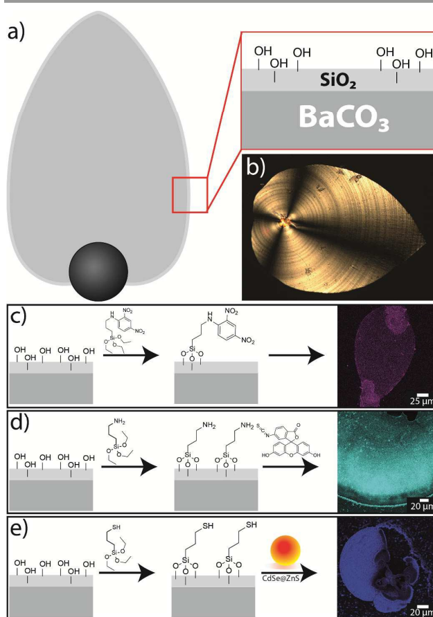
Figure 2. Post-functionalisation of biomorphs with different trialkoxysilanes. a) Schematic drawing of a biomorph sheet with a thick outer silica skin carrying free silanol groups accessible for coupling reactions. b) Polarised optical micrograph of a typical biomorph sheet. c-e) Schemes for the post-silanisation of as-grown biomorphs with c) DNPTEs, d) 3-APTES and further functionalisation with FITC, e) 3-MPTES and subsequent binding of CdSe@ZnS quantum dots. In all cases, successful functionalisation is proven by corresponding CLSM images (right).
