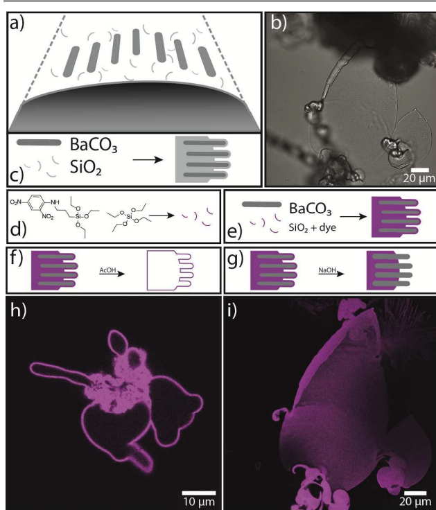
Figure 1. In-situ functionalisation of biomorphs by silane co-condensation. a) Schematic drawing of the growth of a biomorph by the continuous formation of carbonate nanocrystals (dark-grey rods) in the presence of silicate species (thin light-grey threads). b) CLSM image (transmission channel) of a biomorph sheet. c) Co-precipitation of \text{BaCO}_3 nanocrystals and unfunctionalised amorphous silica. d) Co-condensation of TEOS and DNPTEs into fluorescent “functional” silica. e) Incorporation of fluorescently labeled silanes into the siliceous component of biomorphs (magenta-coloured domains). f) Selective dissolution of the carbonate component by acid post-treatment, leading to a hollow silica structure. g) Partial dissolution of the (outer) silica component by NaOH post-treatment. h and i) CLSM images (fluorescence channel) of functional biomorphs after acid and base treatment, respectively.
