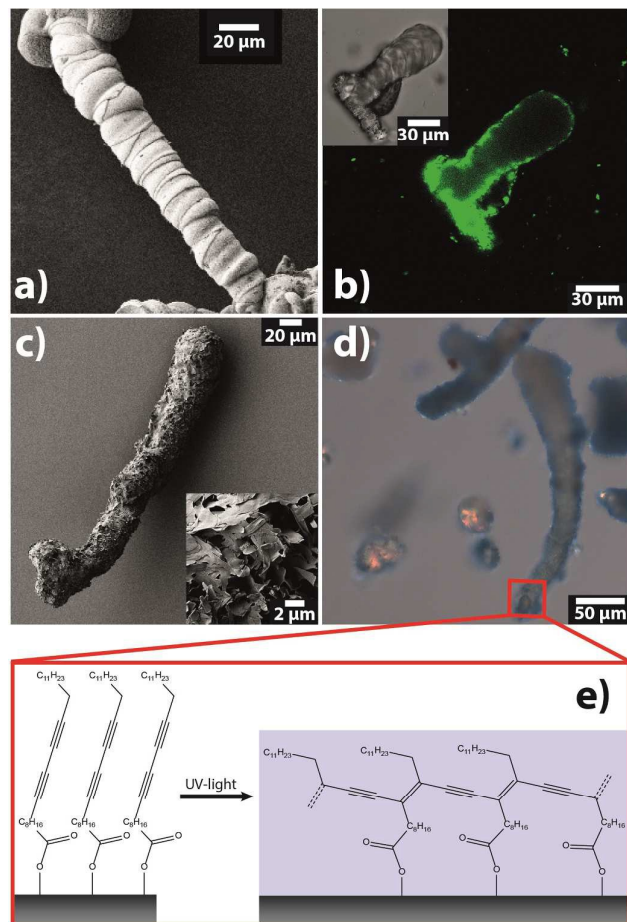
Figure 4. Organic polymerisation on biomorphs. a) SEM image of a structure with worm-like morphology before functionalisation. b) CLSM images (main window: fluorescence channel ( \lambda_{exc.} = 561 nm), inset: transmission channel) of another worm-like structure after functionalisation. c) SEM image of a poly(PCDA)-coated worm. The inset shows a zoom on the surface of the aggregate, revealing the flake-like character of the polymer coating. d) Optical micrograph of biomorphs after functionalisation,
