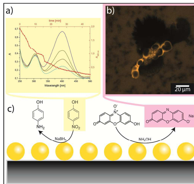
Figure 3. Catalytic reactions with AuNPs immobilised on biomorphs. a) UV-Vis spectra showing the reduction of p-nitrophenol by \text{NaBH}_4 . b) CLSM image of a AuNP-bearing biomorph in a solution of resazurin and hydroxylamine. The formation of the reduced state (resorufin) can be detected by enhanced fluorescence at the surface of the biomorph. c) Schematic drawing of the two test reactions using the immobilised particles as catalyst. The coloured molecules were analytically observed.
