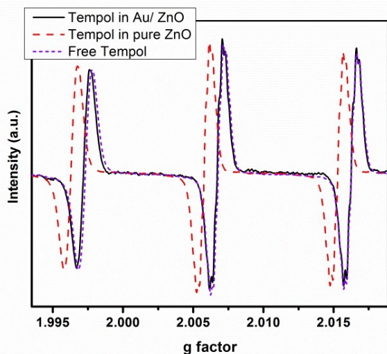
Figure 5. Comparison between the experimental degassed spectrum of free TEMPOL with those obtained in the presence of ZnO and Au/ZnO nanostructure. The spectrum obtained in the presence of ZnO is clearly different from the others, revealing the interaction of the TEMPOL with the semiconductor surface, see text .
