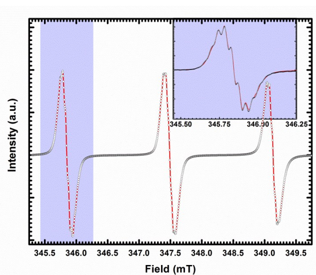
Figure 2. Room temperature EPR spectra of degassed TEMPOL dissolved in ethylene glycol, hollow circles in black account for the experimental data. The red lines are the results of the simulation, see text. The inset shows the peak centered at 345.75 mT with higher resolution.
