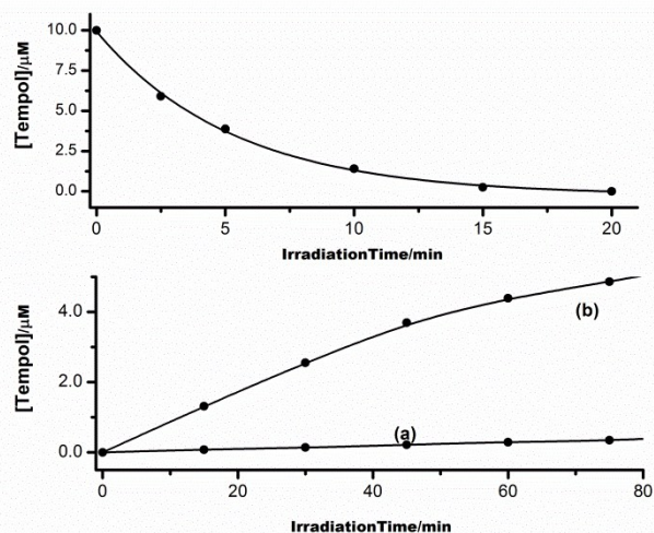
Figure 3. Upper panel: Decay of TEMPOL under UV irradiation. Lower panel: regeneration of TEMPOL in the dark (curve a) and under excitation of the nanostructures with wavelengths larger than 435 nm.
