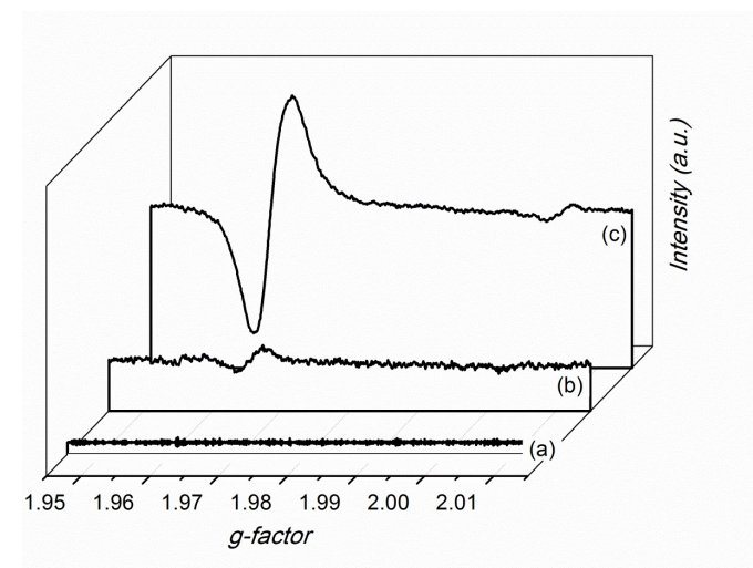
Figure 7. Room temperature EPR spectra of as-prepared ZnO nanoparticles suspended in ethylene glycol (a), and Au/ZnO nanoparticles before, (b), and during continuous irradiation at wavelengths longer than 435 nm, (c).
