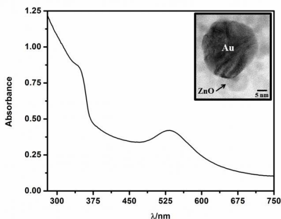
Figure 1. UV-Vis spectrum of the Au / ZnO nanostructures dispersed in ethylene glycol. The nanocomposite was obtained by reduction of a 62 \mu\text{M} \text{HAuCl}_4 solution in ethylene glycol in the presence of ZnO, ( [\text{ZnO}] = 8.1 \text{ mM} ) see reference 30. Inset HRTEM showing the contact between Au and ZnO.
