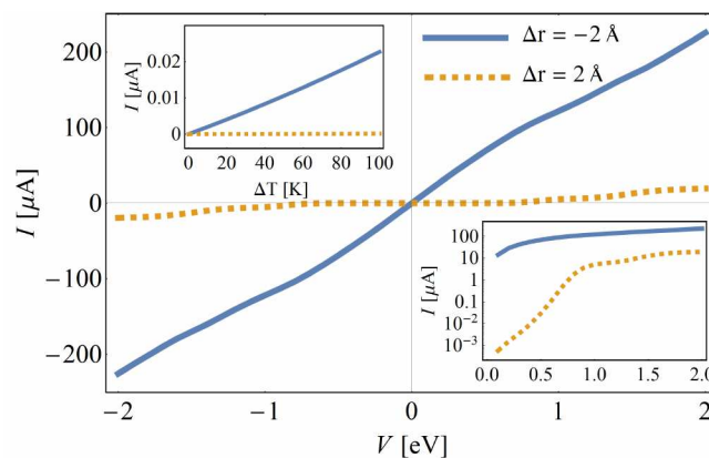
Fig. 5 Main panel: I-V curve of a 2,21-diaza[9]helicene (4) HMJ for two values of stretching distance, \Delta r = -2\text{\AA} (solid blue line) and \Delta r = 2\text{\AA} (dashed yellow line). A switching ratio of \sim 4 orders of magnitude between the "On" and "Off" state can be seen in the bottom-right inset, where the same is plotted on a log scale. Top-left inset: the thermo-current I as a function of temperature difference \Delta T for the two states, showing a switching behavior.
