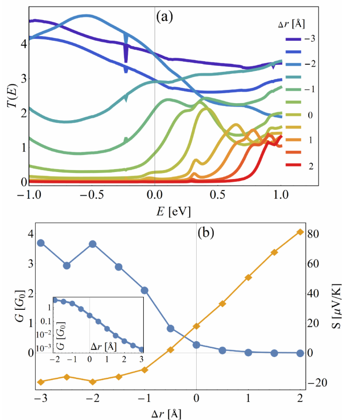
Fig. 3 Transmission and thermopower properties of HMJ formed by 2,21-diaza[9]helicene (4) and gold(1,1,1) electrodes:(a) Transmission T(E) as a function of energy E for different inter-electrode distances incrementally changed about \Delta r = -3, 2.5, -2, \dots, 1, 2 \text{ \AA} (measured from the relaxed inter-electrode distance). (b) Conductance (blue circles) and thermopower (yellow diamonds) as a function of \Delta r . Inset: Conductance on a logarithmic scale, demonstrating the order of magnitude change in conductance with changing \Delta r .
