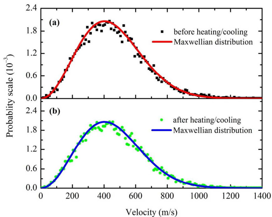
Figure 3. Atomic velocity distributions in 9.94 \times 40.19 \text{ nm}^2 ( x \times y ) armchair phosphorene. (a) Velocity distribution after 500 ps NVT and 500 ps NVE simulations. (b) Velocity distribution after 2 ns NEMD simulations. Good agreement between the MD simulation and Maxwellian velocity distribution is observed, indicating the temperature distribution has reached steady state before data collection.
