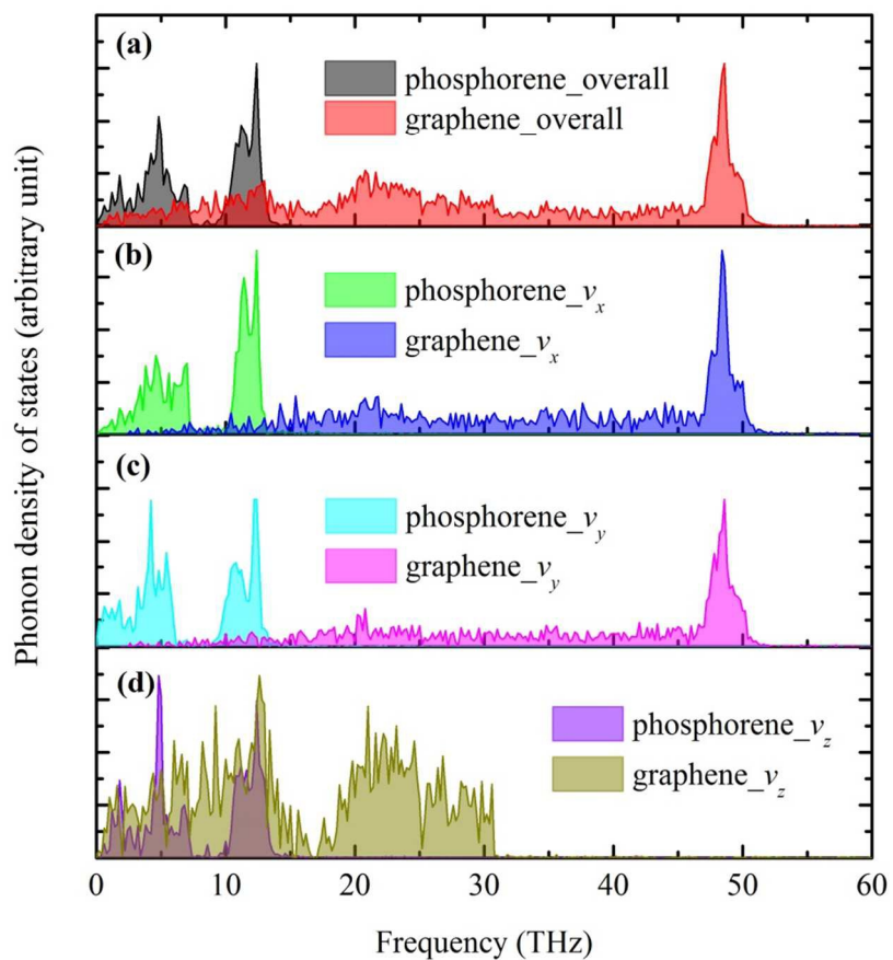
Figure 5. (a) PDOS of phosphorene and graphene sheets (for heat conduction in the armchair direction), respectively, at temperature 300 K. (b-d) Decomposed PDOS in x , y and z directions. The PDOS peak locations remain unchanged in phosphorene sheet. While the in-plane and out-of-plane phonons of graphene sheet are anisotropic.
