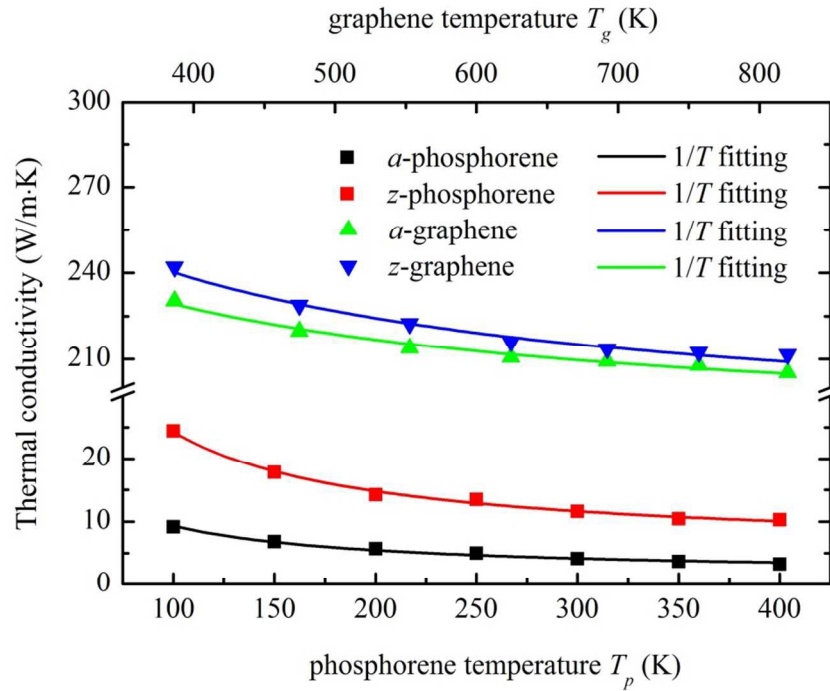
Figure 6. Temperature dependence of thermal conductivity for phosphorene /graphene in the armchair and zigzag direction. Fitting results by the inverse relationship with temperature ( \kappa \sim 1/T ) are plotted with solid lines. Quantum correction is applied to the MD temperature of graphene sheet and shown in the top x axis.
