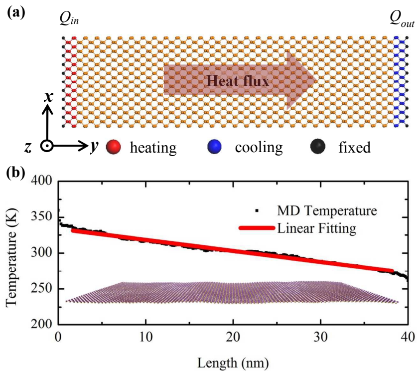
Figure 2. (a) Illustration of the NEMD process. Black atoms at the boundaries of the system are fixed in position. Free boundary is used out-of-plane z direction. Periodic boundary condition is applied in the width ( x ) direction. Red and blue areas are denoted as heat bath and heat sink respectively. (b) Temperature distribution along the heat flux direction ( y ) in the 9.94 \times 40.19 nm 2 ( x \times y ) phosphorene in the armchair direction. Red solid line denotes the linear fitting results. Atomic configuration of phosphorene after the heating/cooling process is shown in the inset.
