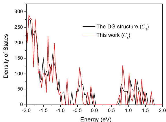
Figure 8. Comparison of the total electronic density of states between the DG structure (Ref. 23) and the best structure (isomer a in Figure 5) from the present work.
