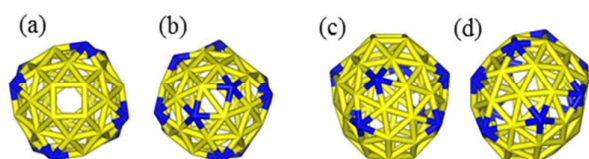
Figure 7. Comparison of the \text{Au}_{58} shell structures between the best structure from this work (a, top view; c, side view) and the best structure (the DG structure) from Ref. 23 (b, top view; d, side view). Blue, five-coordinated Au atoms.
