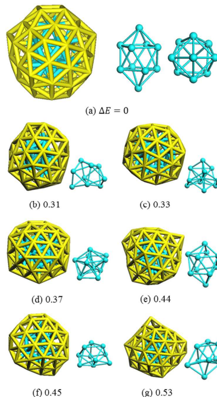
Figure 5. The most stable isomer (a) and other less stable ones as labeled in Figure 3. Core structures are also shown (cyan). The number shows the DFT total energy (eV) relative to isomer (a).
