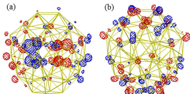
Figure 6. (a) HOMO and (b) LUMO of isomer (a) of \text{Au}_{58} : positive, blue; negative, red.
