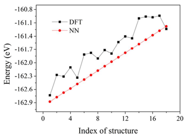
Figure 2. Comparison between NN and DFT energies of 18 Au 58 structures spanning a 1.8-eV energy window. The NN energies were chosen intentionally to be equally spaced.
