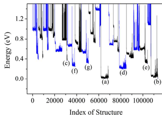
Figure 3. The energy landscape of 20 BH run based on NN potential. Adjacent two BH are indicated by different colour (blue or black). (a)-(g) are the local minima with structure shown in Figure 5.
