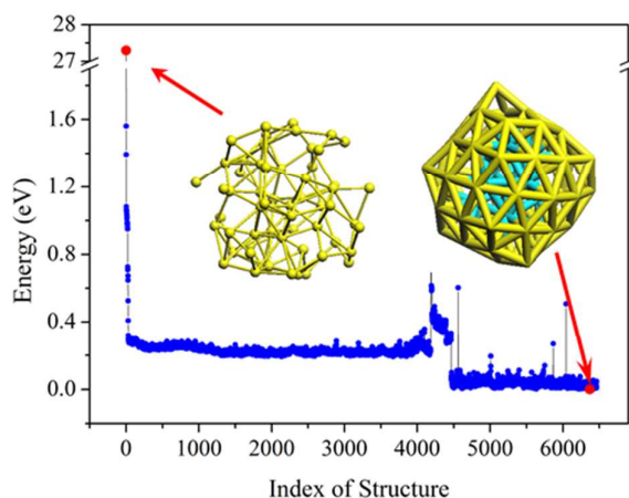
Figure 4. Energy landscape of an example single BH run based on NN potential with 6500 steps. Red dots denote the initial random structure and the most stable structure found by the BH.
