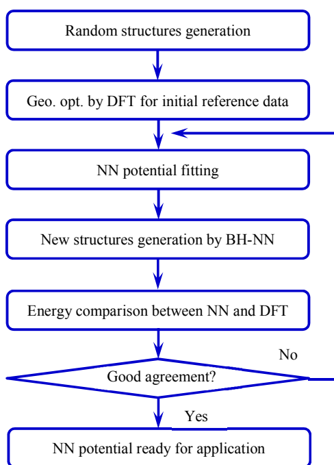
Figure 1. Flow chart of the NN potential construction. BH: basin-hopping algorithm; NN: neural network potential; DFT: density functional theory.
