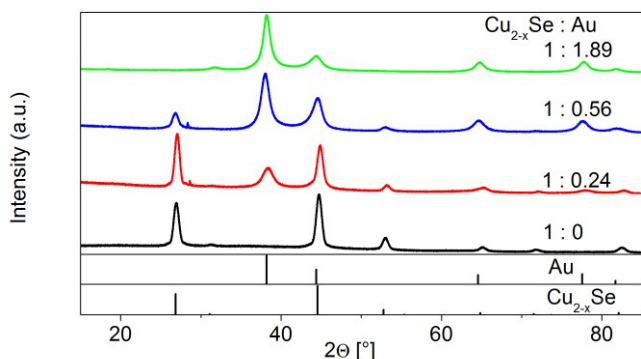
Fig. 5 XRD patterns of the original \text{Cu}_{2-x}\text{Se} seed particles ( 1:0 ) and of the \text{Cu}_{2-x}\text{Se} -Au hybrid structures with different \text{Cu}_{2-x}\text{Se}:\text{Au} ratios ( 1:0.24 , 1:0.56 and 1:1.89 ). The reference structural data shows fcc \text{Cu}_{2-x}\text{Se} berzelianite (PDF card #: 01-072-7490) and fcc Au (PDF card #: 00-004-0784).
