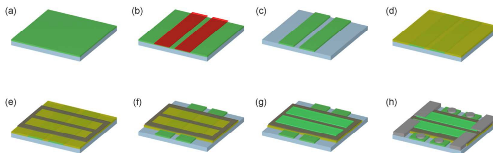
Figure 2. Illustration of the all-solution TOLED fabrication process: (a) deposition of the conductive PEDOT:PSS electrode, (b) masking of the cathodes by adhesive tape, (c) dissolution of the unprotected PEDOT:PSS and subsequent removal of the tape, (d) deposition of all functional layers other than the electrodes, (e) application of another adhesive tape to define the shape of the anode, (f) outer removal of functional layers to access the bottom cathode, (g) application of the PEDOT:PSS/AgNW top electrode utilizing selective wetting within the adhesive tape voids and (h) application of metal contact pads that do not affect the working principle of the all-solution processed TOLED.
