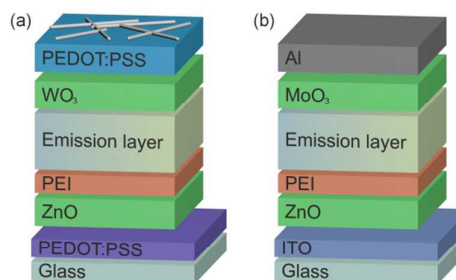
Figure 1. Device architectures of (a) the all-solution processed TOLEDs comprising PEDOT:PSS bottom cathodes and PEDOT:PSS/AgNW top anodes and (b) the opaque reference OLEDs.
