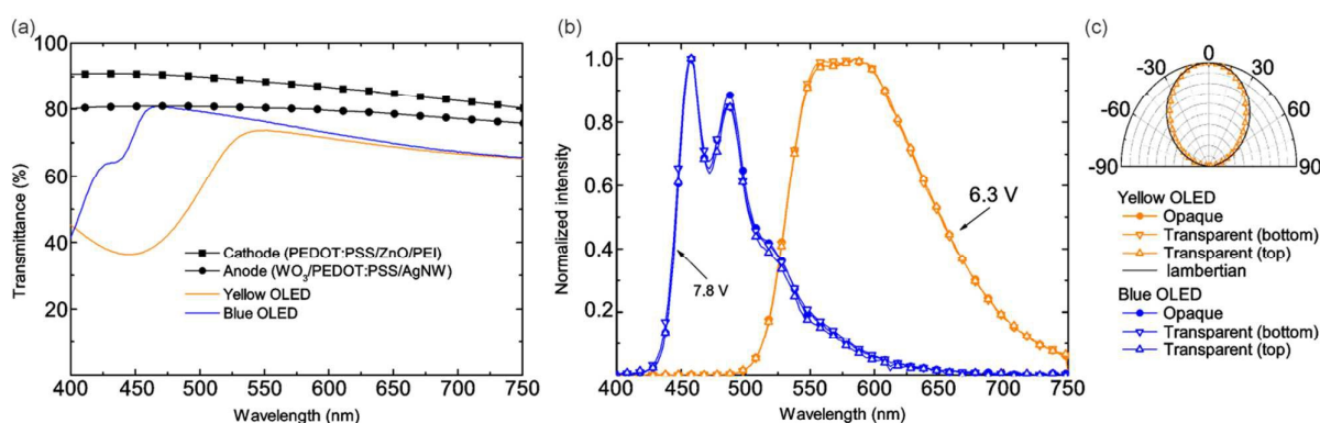
Figure 3. (a) Typical transmittance spectra of the top and bottom electrodes, and of an entire device comprising either of the light-emitting polymers Super Yellow or Merck Blue. (b) Emission spectra of the yellow and blue reference OLEDs and TOLEDs at 6.3 V or 7.8 V driving voltage, respectively. The shapes of the emission spectra in top and bottom direction match the shape of the emission spectra of the respective opaque devices. (c) Lambertian distribution of the light emitted through the PEDOT:PSS/AgNW electrode (Yellow OLED).
