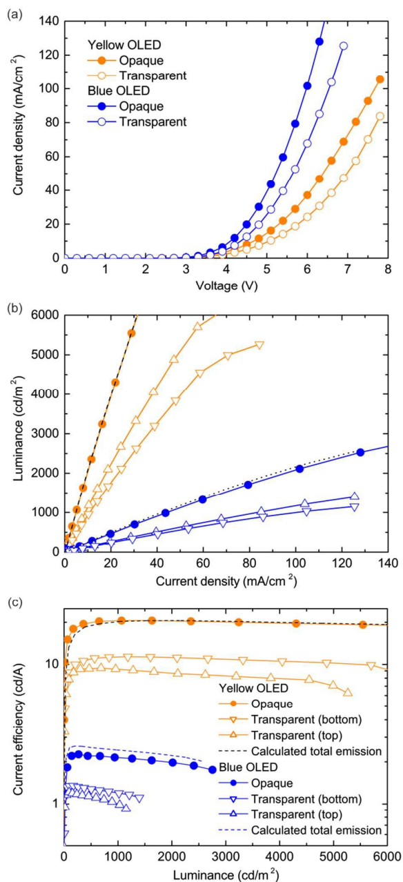
Figure 5. Optoelectronic characteristics of the yellow- and blue-emitting TOLEDs in comparison to the respective opaque reference devices. In bottom configuration, the light emitted through the glass substrate was collected by the spectrometer, whereas, in top configuration, the light emitted through the anode was analysed. (a) Current density vs. voltage ( J - V ), (b) luminance vs. current density ( L - J ), (c) current efficiency vs. luminance.
